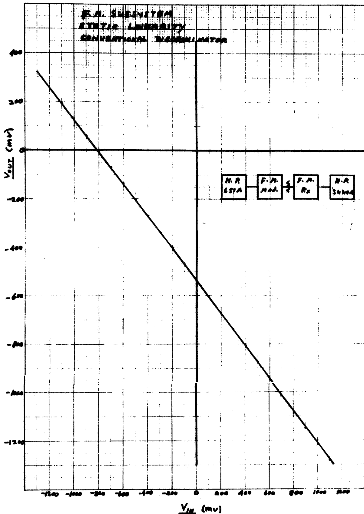
Figure 3.3.3. F. M. Subsystem Static Linearity Conventional Discriminator
