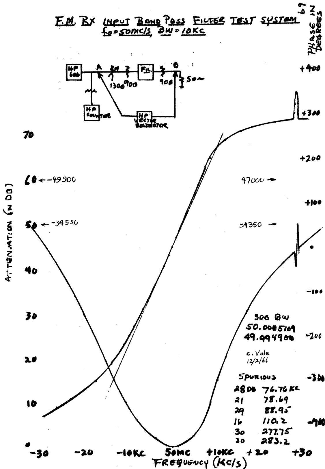
Figure 3.3.2.12. F. M. Rx Input Band Pass Filter Test System f_0 = 50 \text{ Mc/s} , BW = 10 \text{ Kc} .
