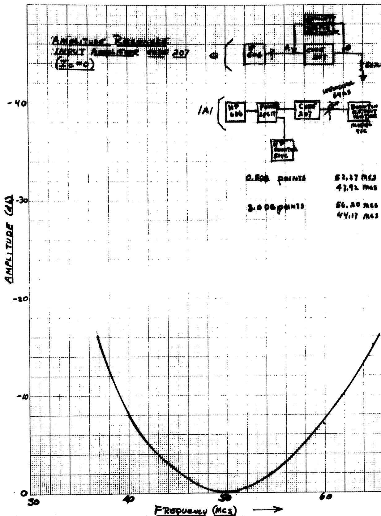
Figure 3.2.2.2. Amplitude Response Input Amplifier Code 207 ( I_c=0 )
