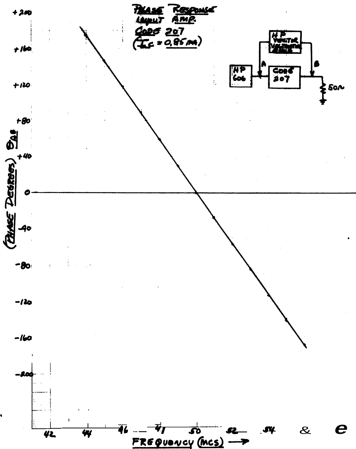
Figure 3.2.2.5. Phase Response Input Amplifier Code 207 ( I_c = 0.85 \text{ MA} )
