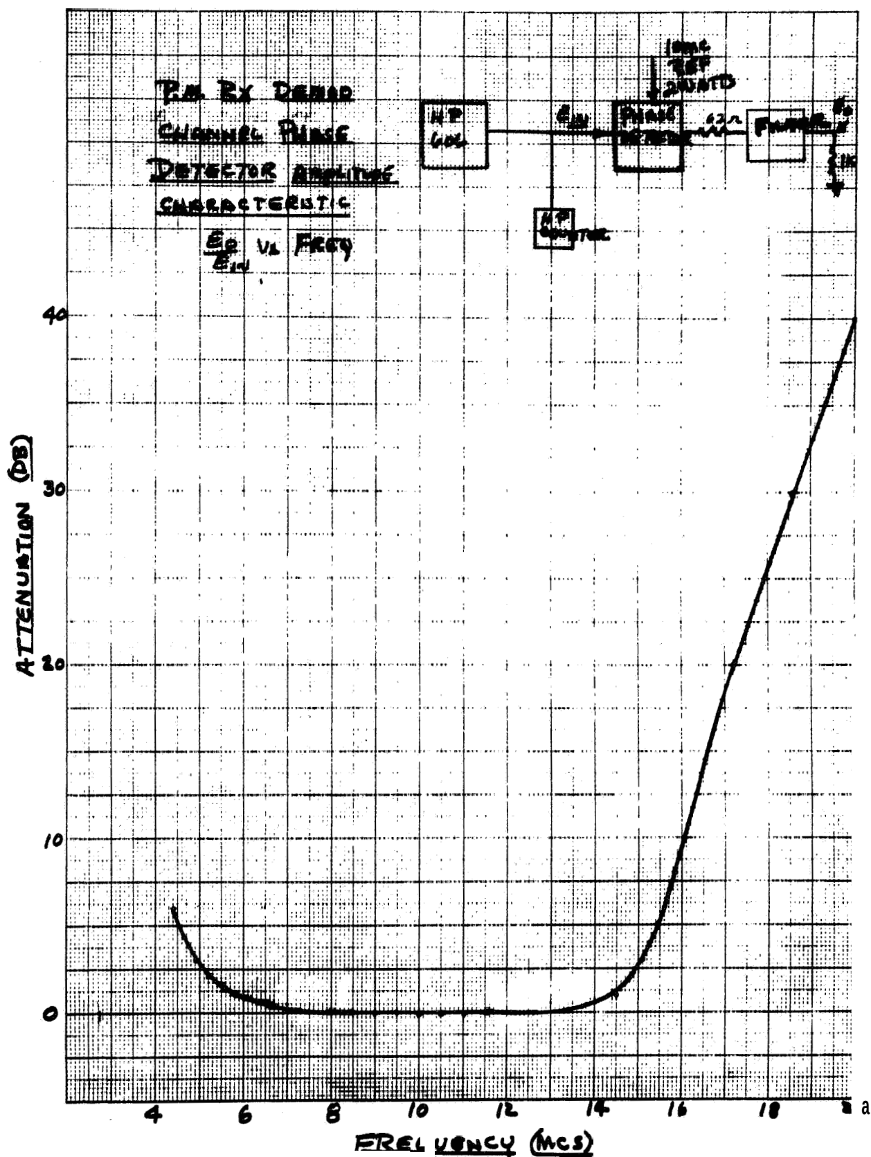
Figure 3. 2. 2, 13. P. M. Rx Demod Channel Phase Detector Amplitude Characteristic \frac{E_o}{E_{in}} Vs Freq.
