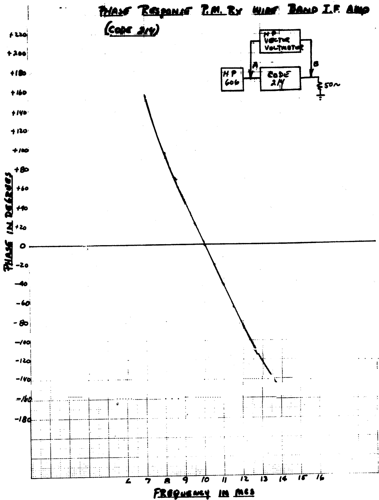
Figure 3.2.2.12. Phase Response P.M.RCVR Wide Band I-F Amplifier (Code 214)
