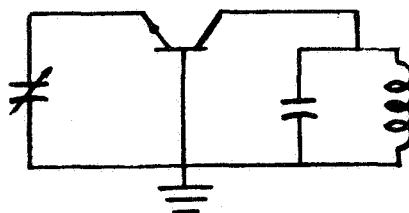
Figure 3.2. 1 3. 3. Basic Oscillator Circuit
