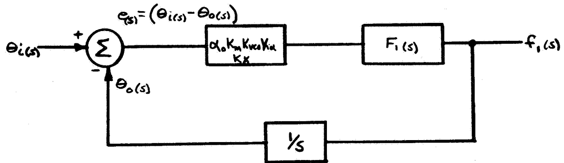
Linear Phase Model Phase Lock Loop
