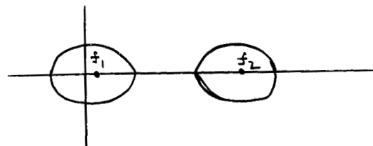
fig. 1b a_1 < 0, a_2 > 0
