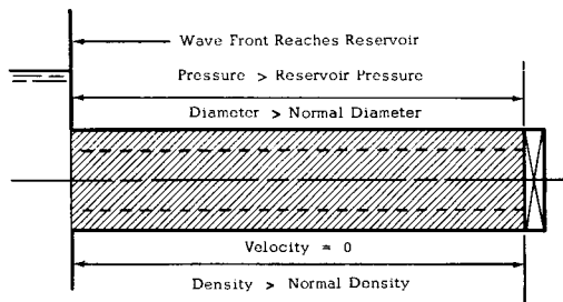
1 (c). FIRST POSITIVE WAVE REACHES RESERVOIR
