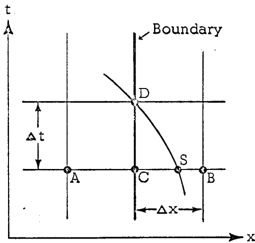
8(a). Left-hand Boundary
