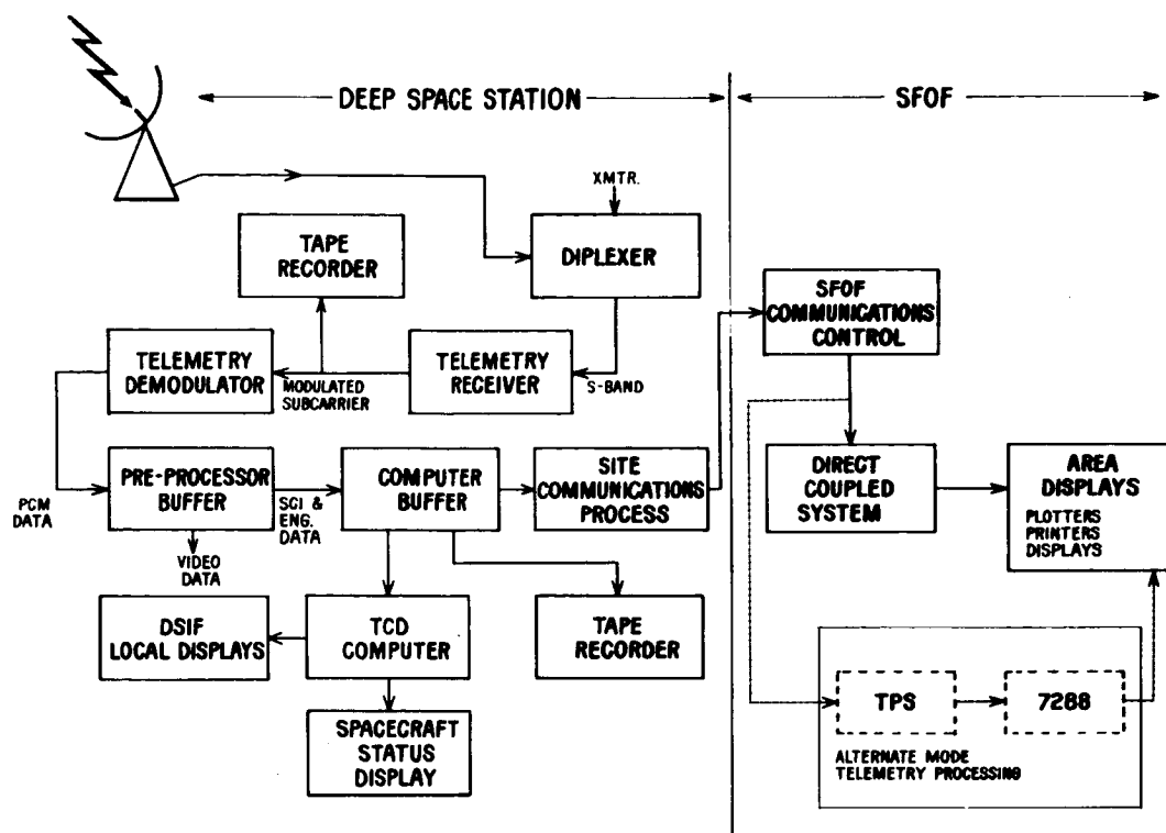
Figure 12. Telemetry Data Flow
