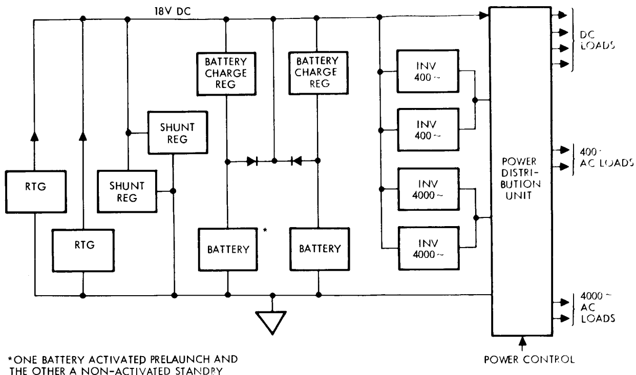
Figure 59. Schematic of Electrical Subsystem
