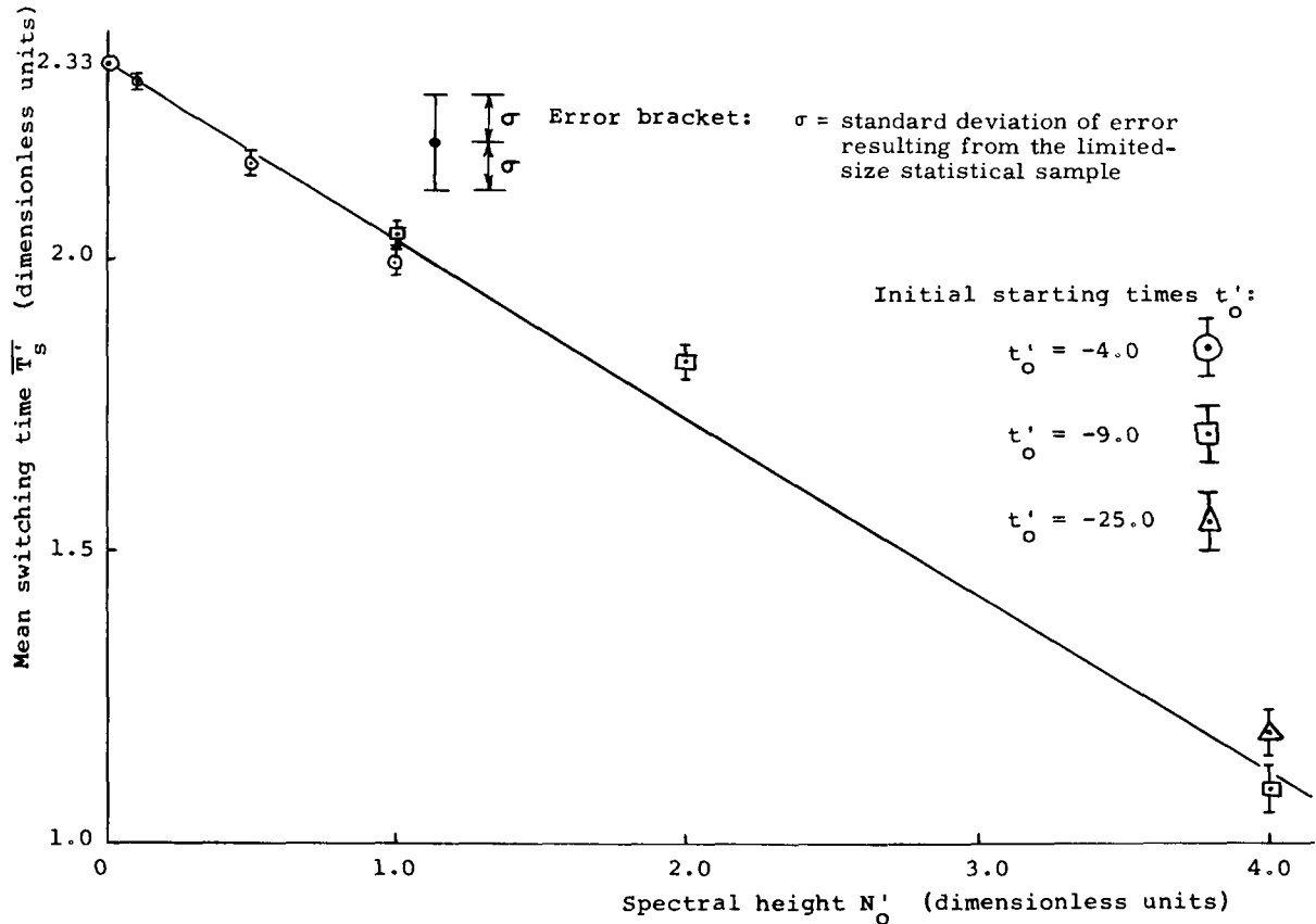
Fig. 19. Mean switching time, \overline{T'_S} , vs noise spectral height, N'_O .
