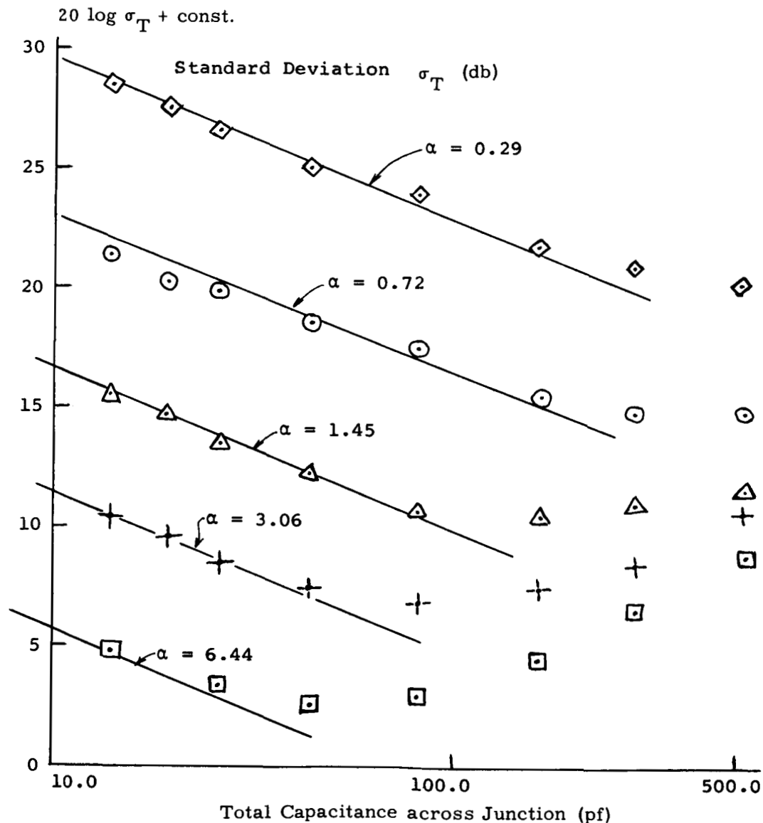
Fig. 22. Jitter standard deviation \sigma_T vs total capacitance C across junction for several values of slope \alpha . The lines shown have a theoretical slope, -6.6 \text{ db/decade} , and were visually fitted to the points.
