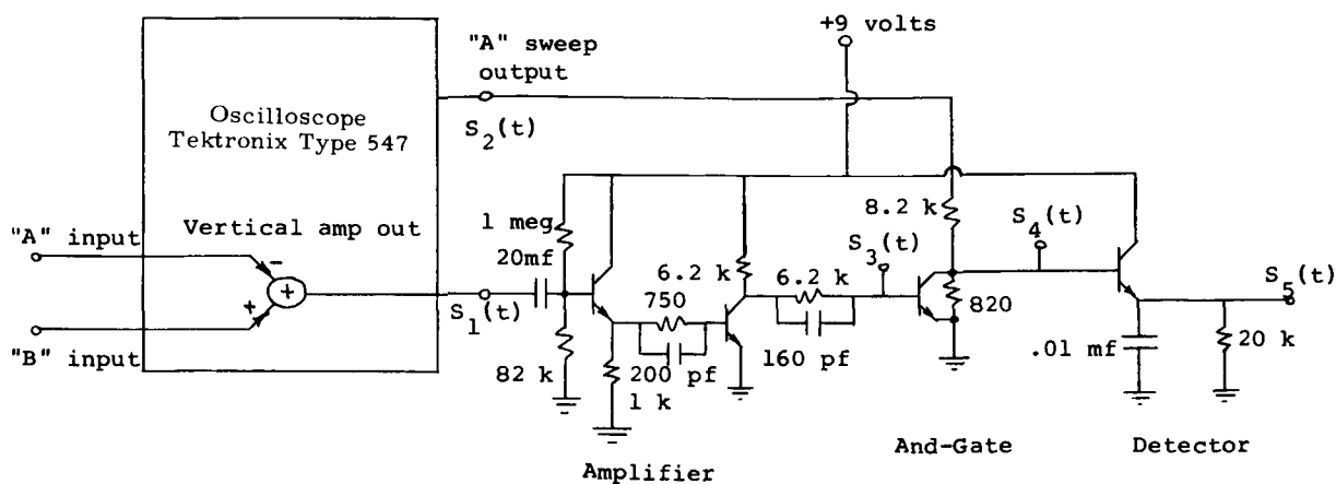
Fig. 28. Differential time-to-height converter.
