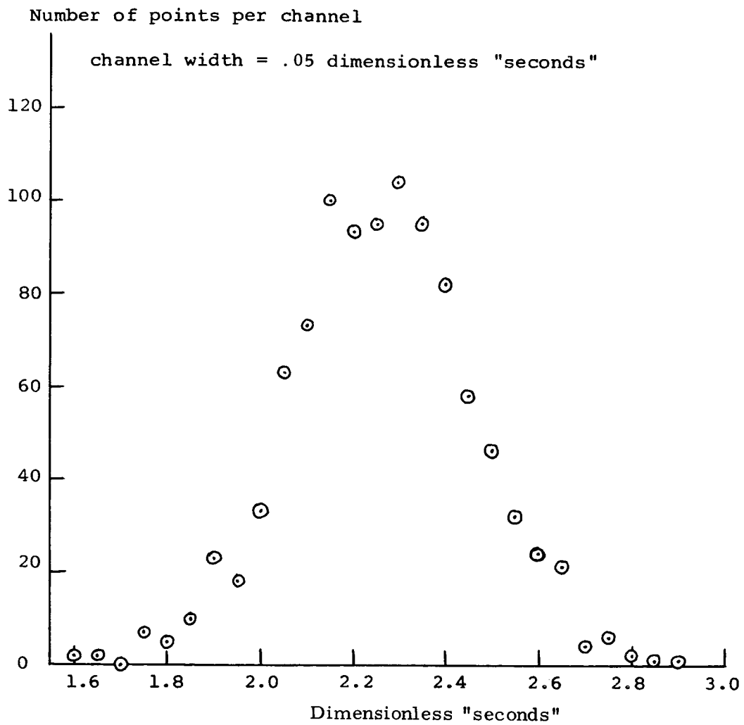
Fig. 16. Typical computed distribution P_{T_s}(t') . N'_0 = 0.1 . Number of samples: 1000.
