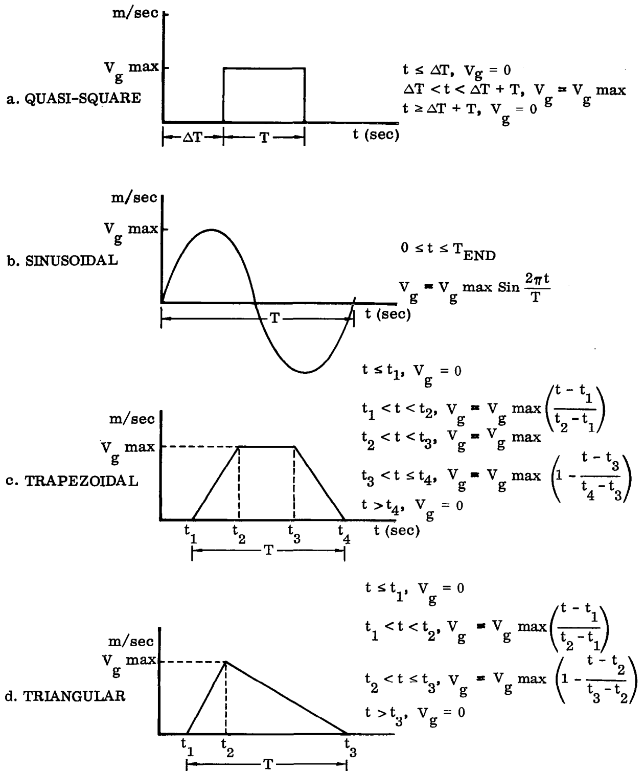
Figure 3. Typical Discrete Gust Waveforms
