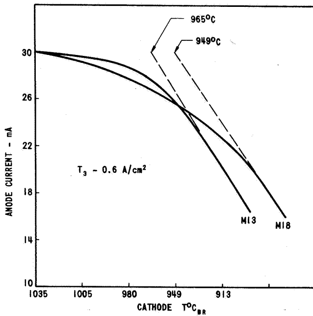
Figure 11 Pore-Type Dispenser Cathode Dip Test
