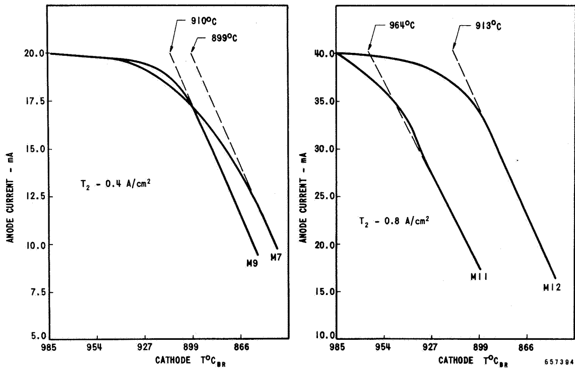
Figure 10 Pore-Type Dispenser Cathode Dip Test
