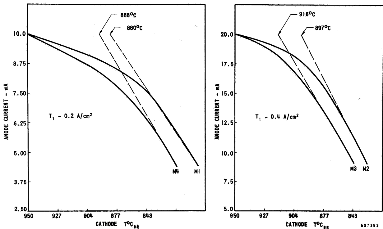
Figure 9 Pore-Type Dispenser Cathode Dip Test
