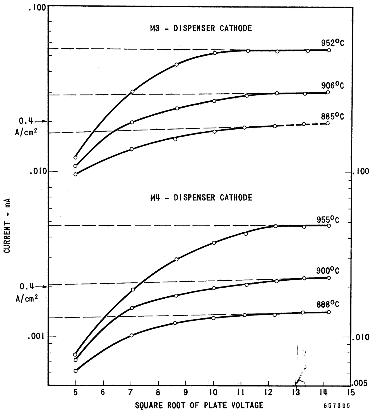
FIGURE 8 Zero Field Current Density
