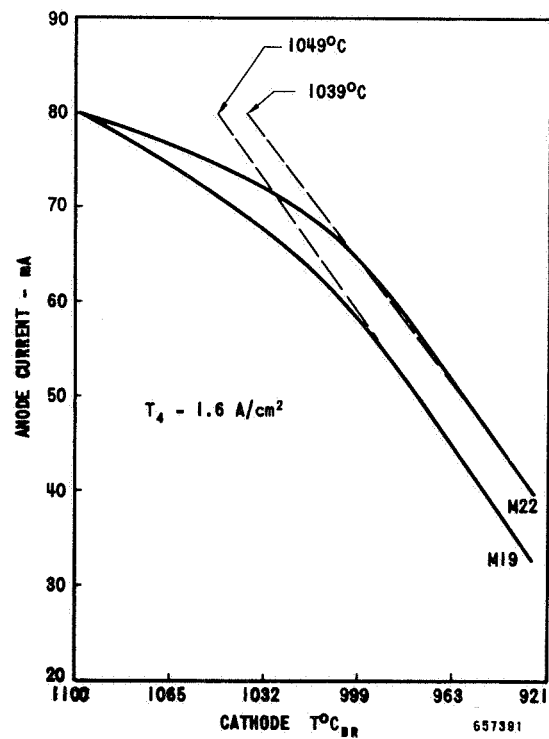
Figure 12 Pore-Type Dispenser Cathode Dip Test
