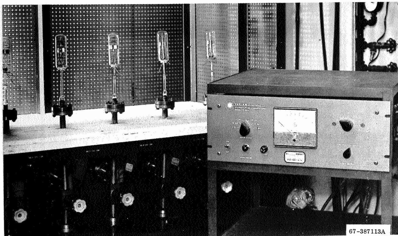
Figure 4. Exhaust System for Diode Test Vehicle (Cathode Laboratory)
