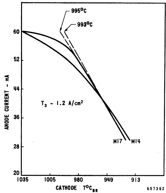
Figure 11 Pore-Type Dispenser Cathode Dip Test
