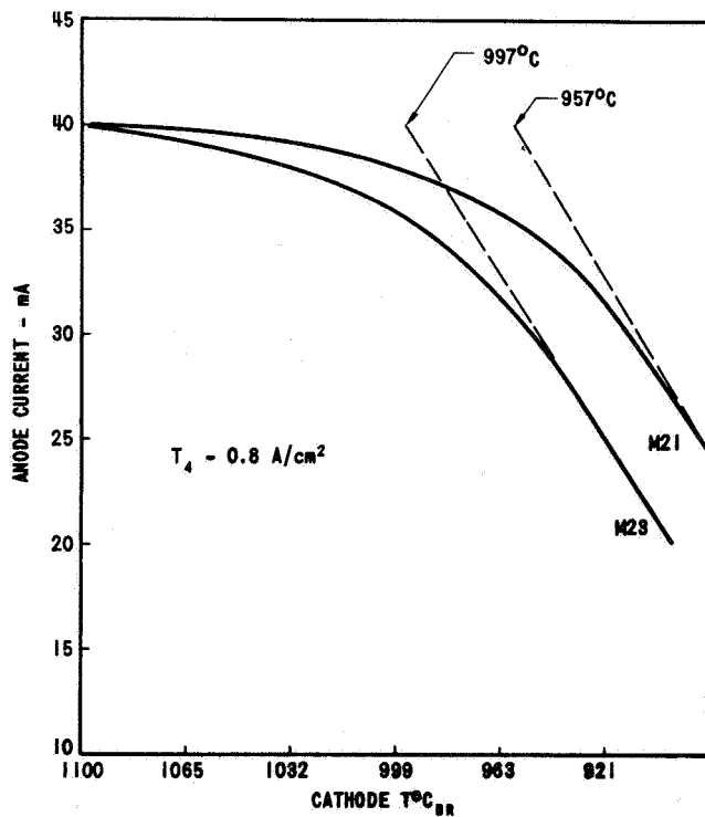
Figure 12 Pore-Type Dispenser Cathode Dip Test
