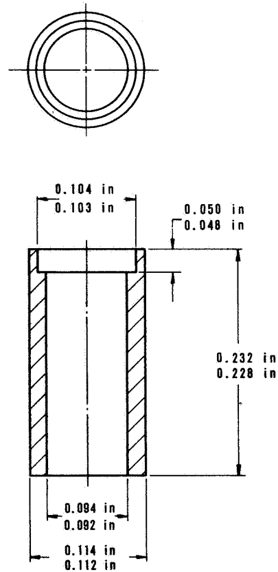
Figure 3. Sleeve for Emission Pellet
