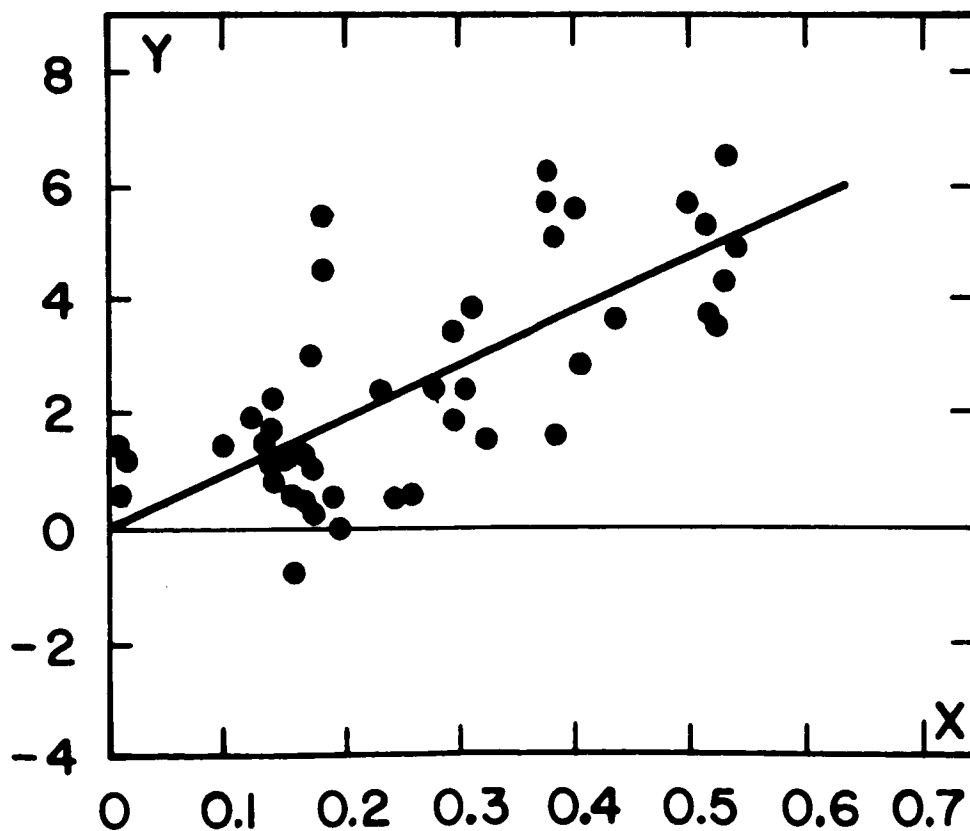
Fig. 4. The X-Y plot for a Rayleigh atmosphere at 0.61 \mu (after Dollfus and Focas 1966; see text for definitions and derivation of X and Y).
