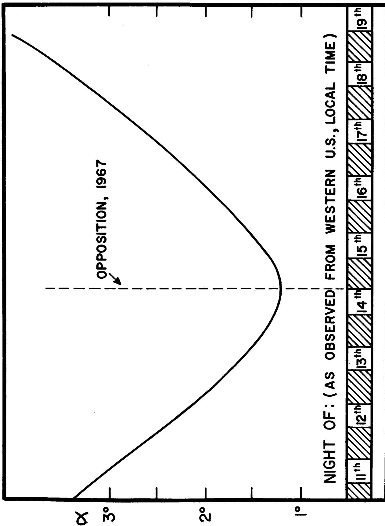
Fig. 7. Phase angle of Mars versus observational opportunities from
