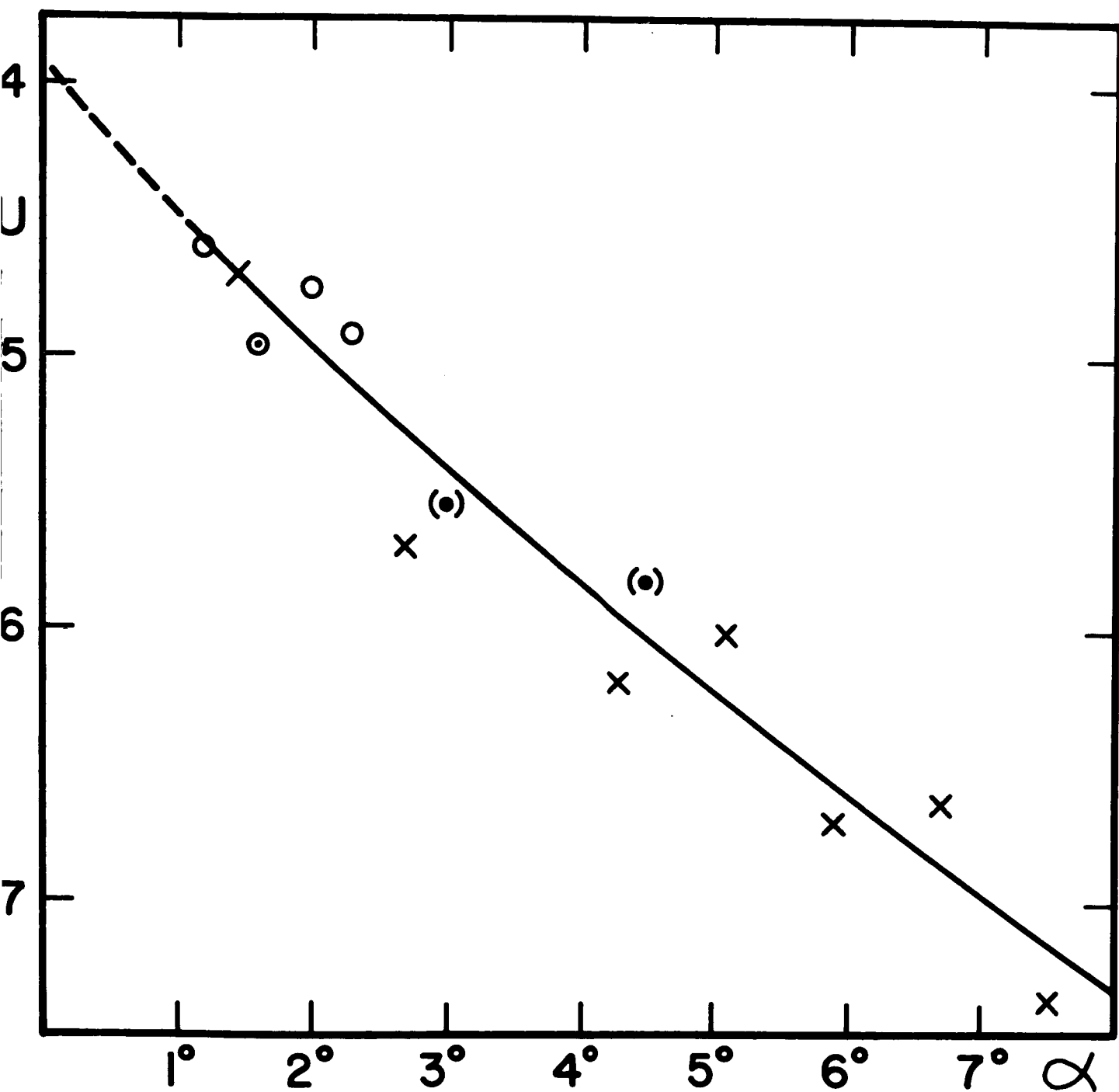
Fig. 14. Variation of the absolute magnitude (uncorrected for transformation errors) of the Martian disk with phase at \lambda = 0.36 \mu during the 1967 opposition. Each point represents an average of the most-often observed positions of rotation of Mars (see text). Point symbols follow the nomenclature of Fig. 12.
