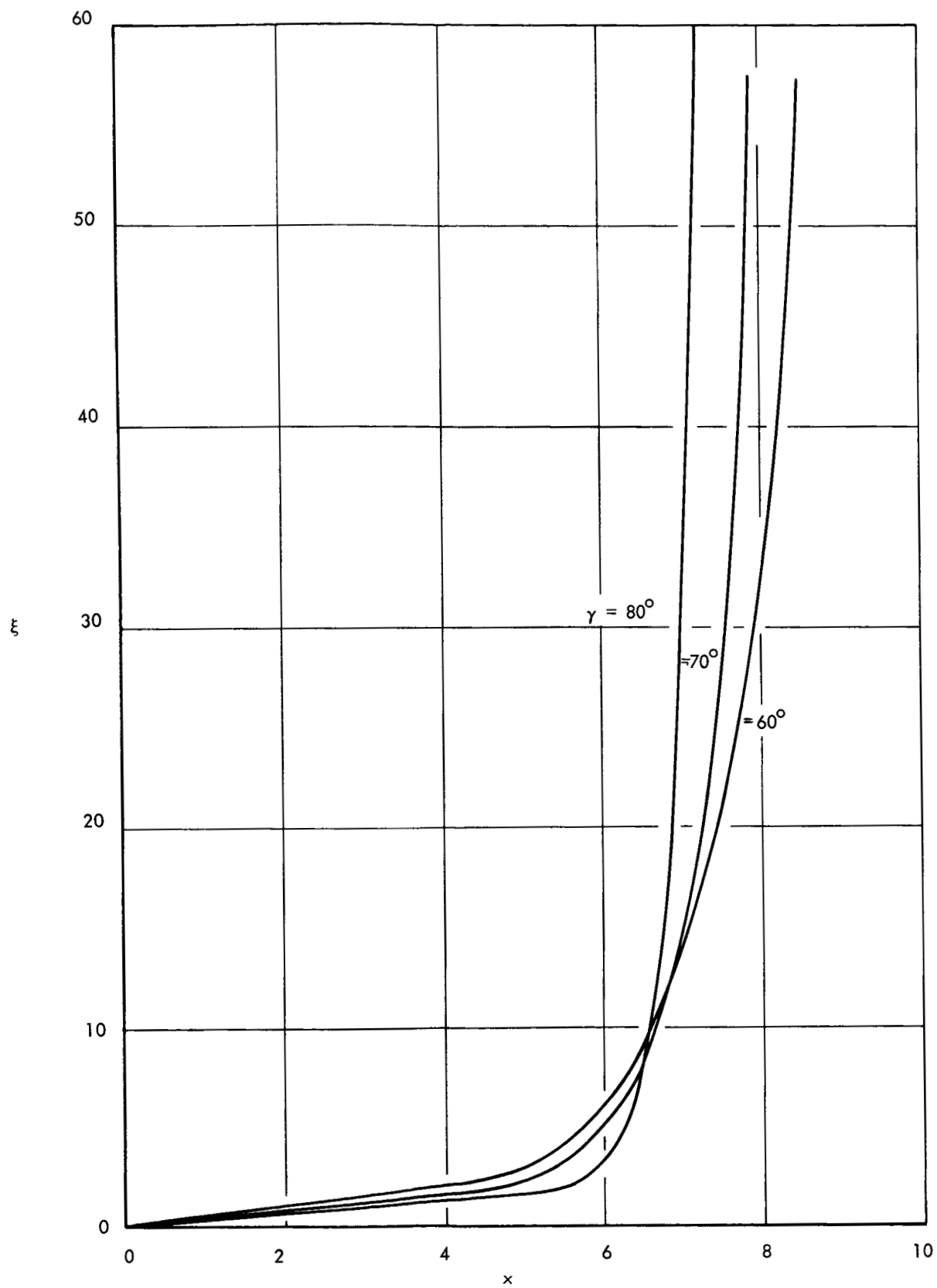
FIGURE 2a - RELATIONS BETWEEN PHYSICAL COORDINATES (x, y) AND TRANSFORMED COORDINATES (\xi, \eta)
