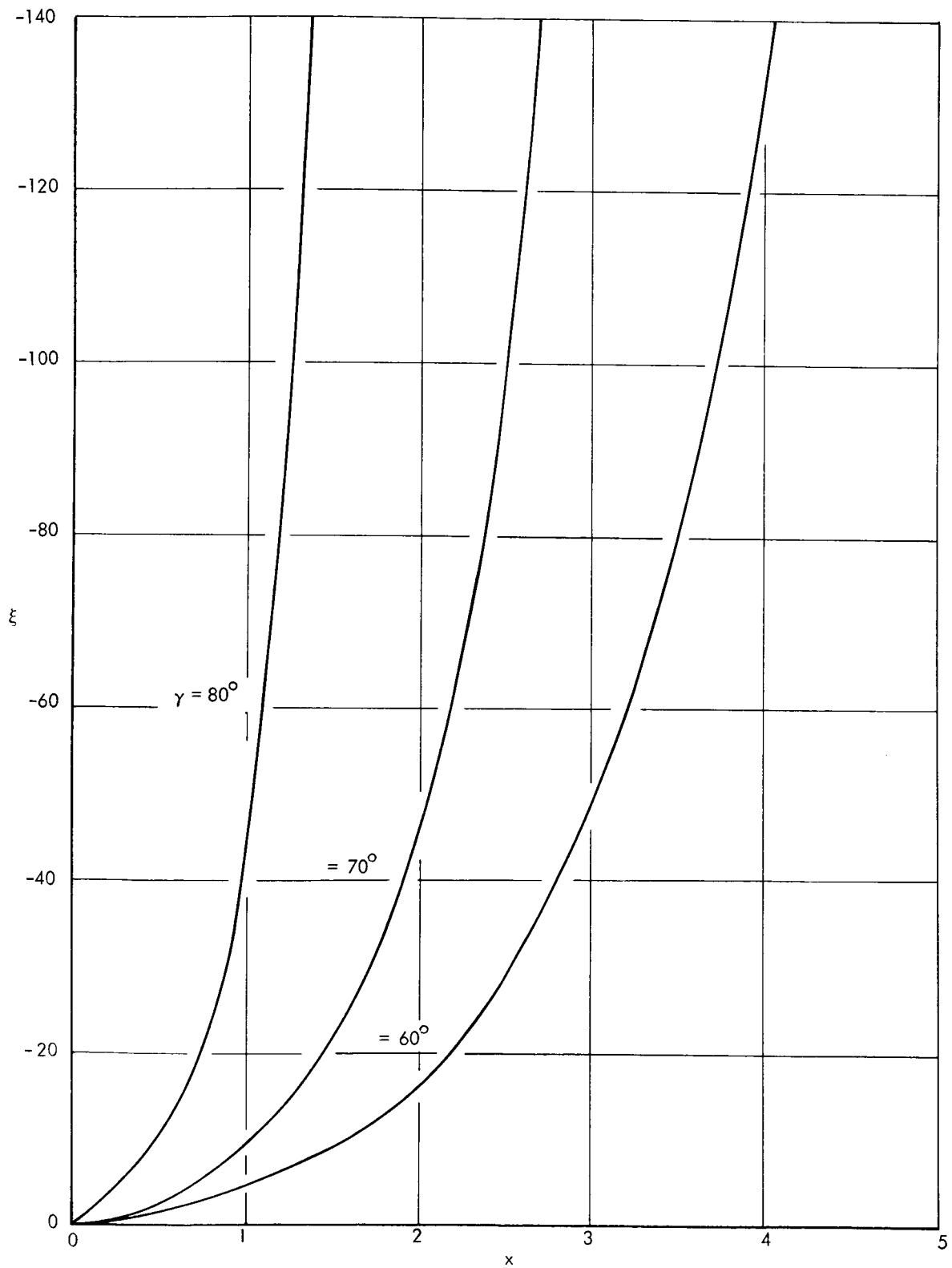
FIGURE 2b - RELATIONS BETWEEN PHYSICAL COORDINATES (x, y) AND TRANSFORMED COORDINATES (\xi, \eta)
