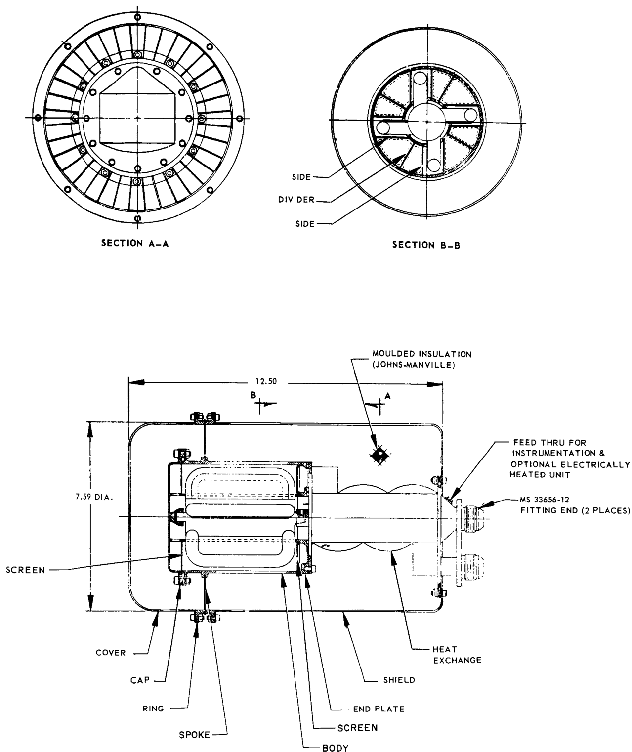
Fig. 1 - IHCOS Conventional Insulation Design
