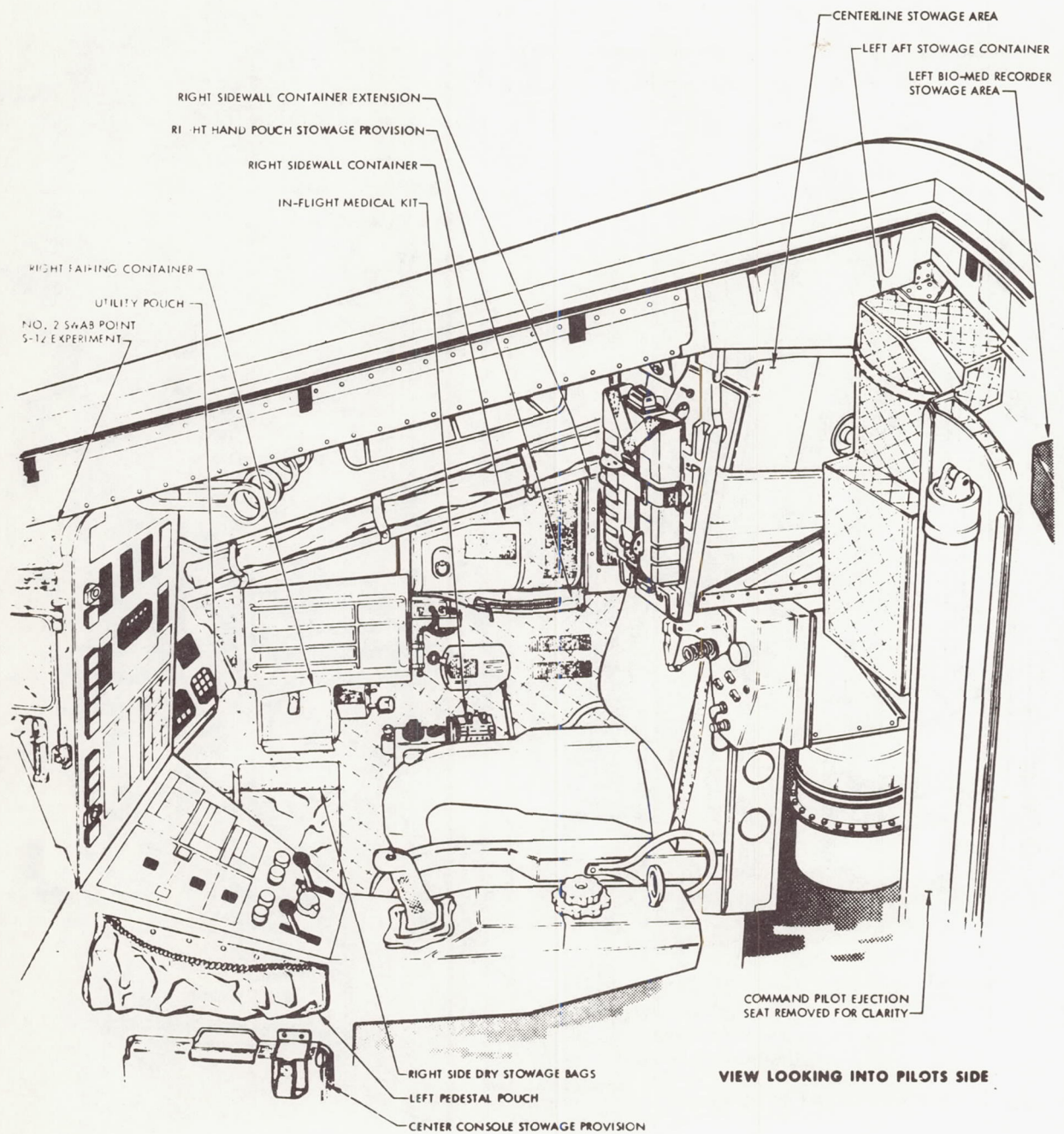
Spacecraft Interior Storage Areas (Sheet 2 of 2)
