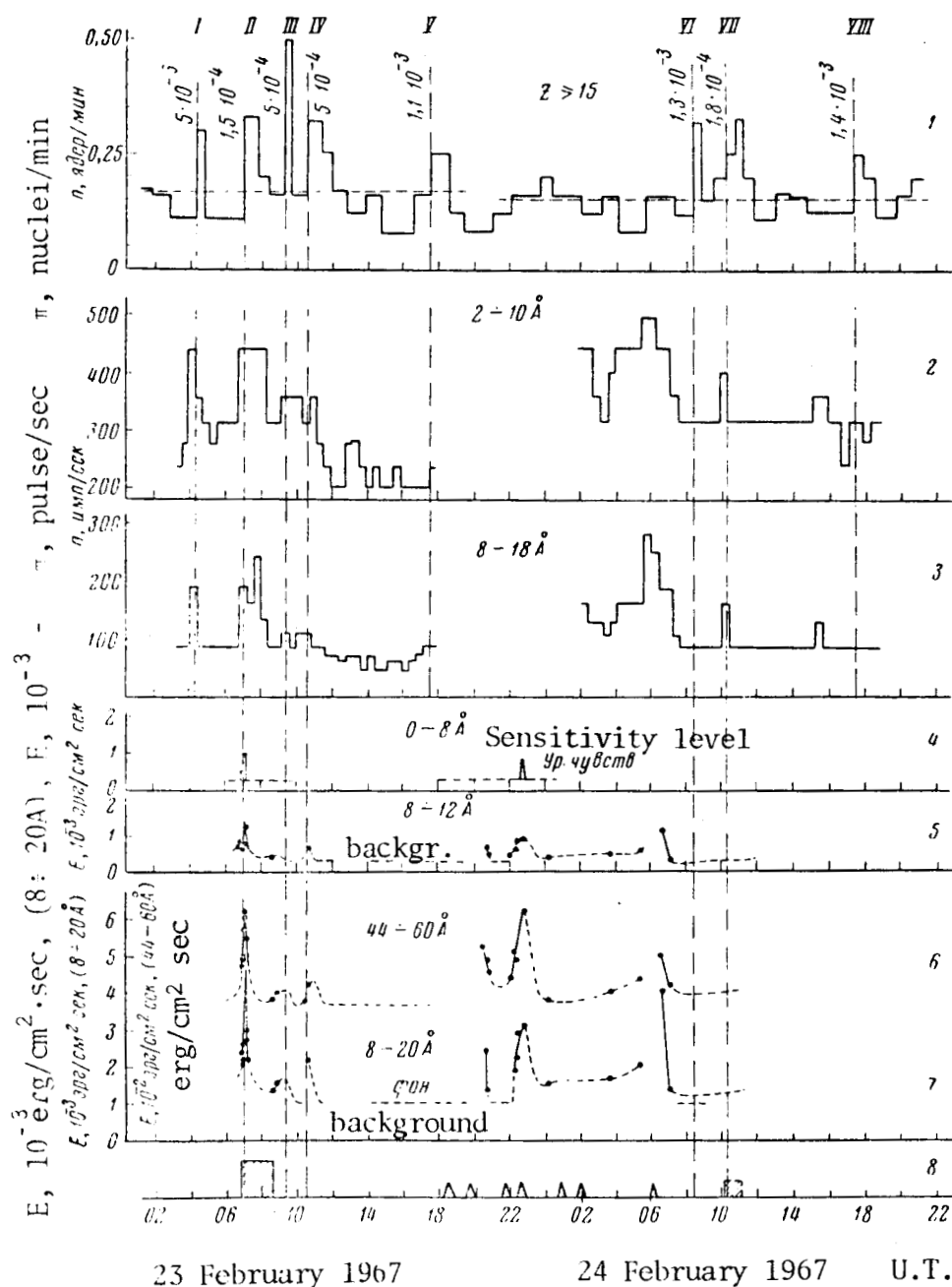
Fig.2. Fine Structure of Flux of Nuclei Increase
