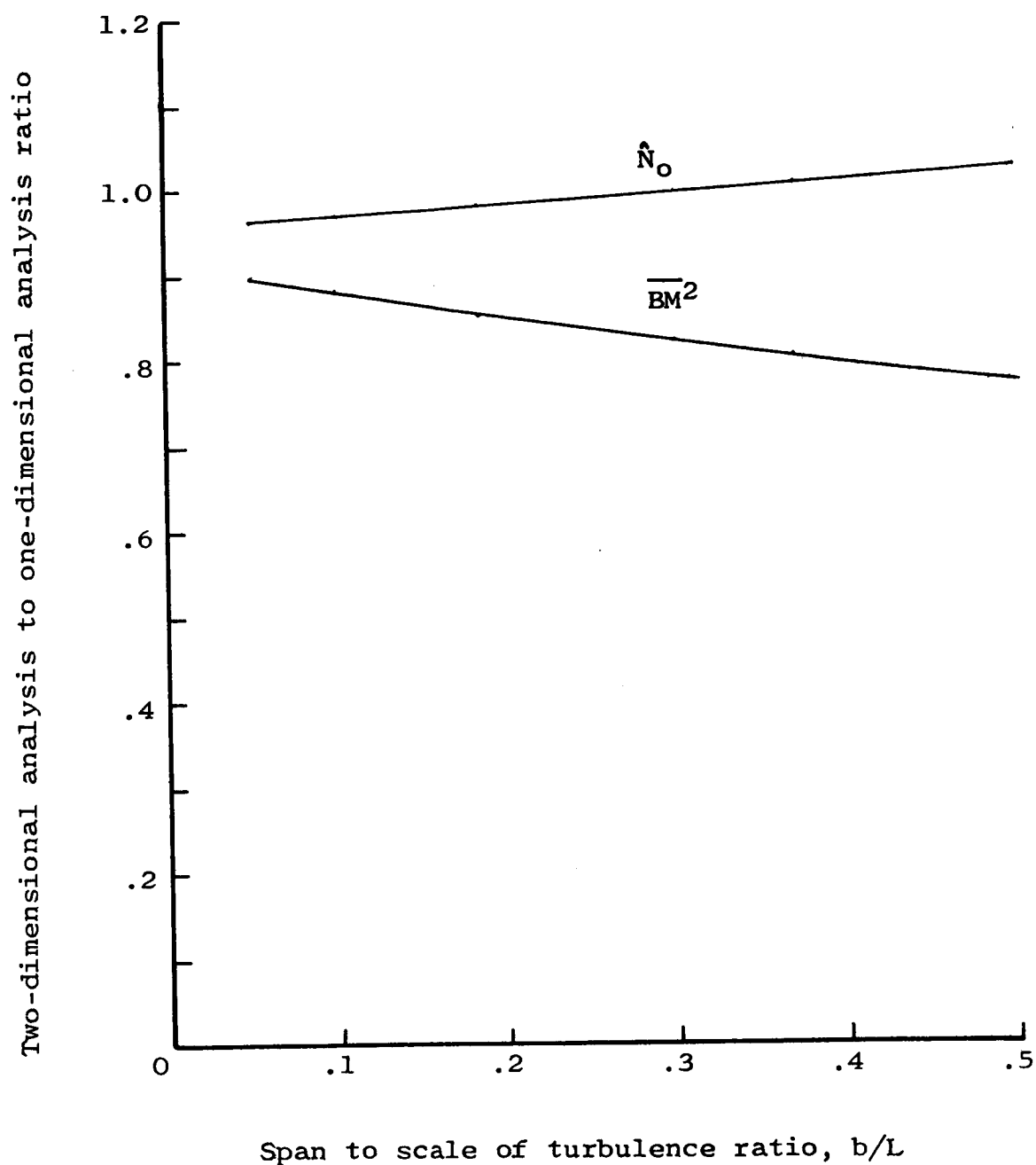
Figure 17.- Reduction of flexible bending moment mean square value and \hat{N}_o given by two-dimensional analysis variation with b/L (mass ratio = 0.585).
