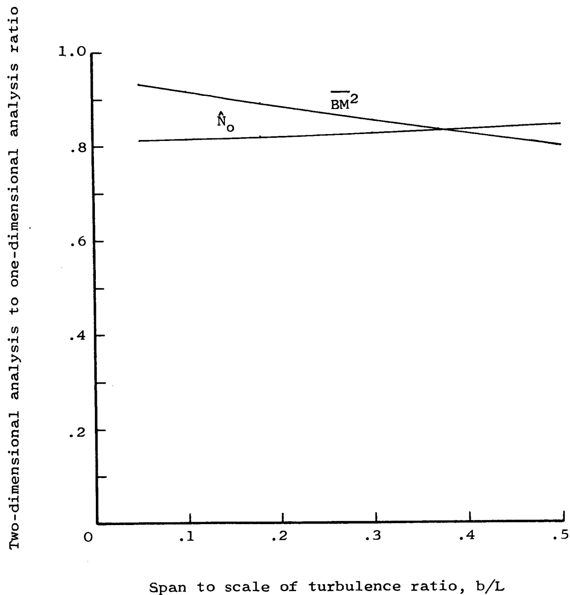
Figure 10.- Reduction of rigid body bending moment mean square value and \hat{N}_o given by two-dimensional analysis variation with b/L (mass ratio = 0.585).
