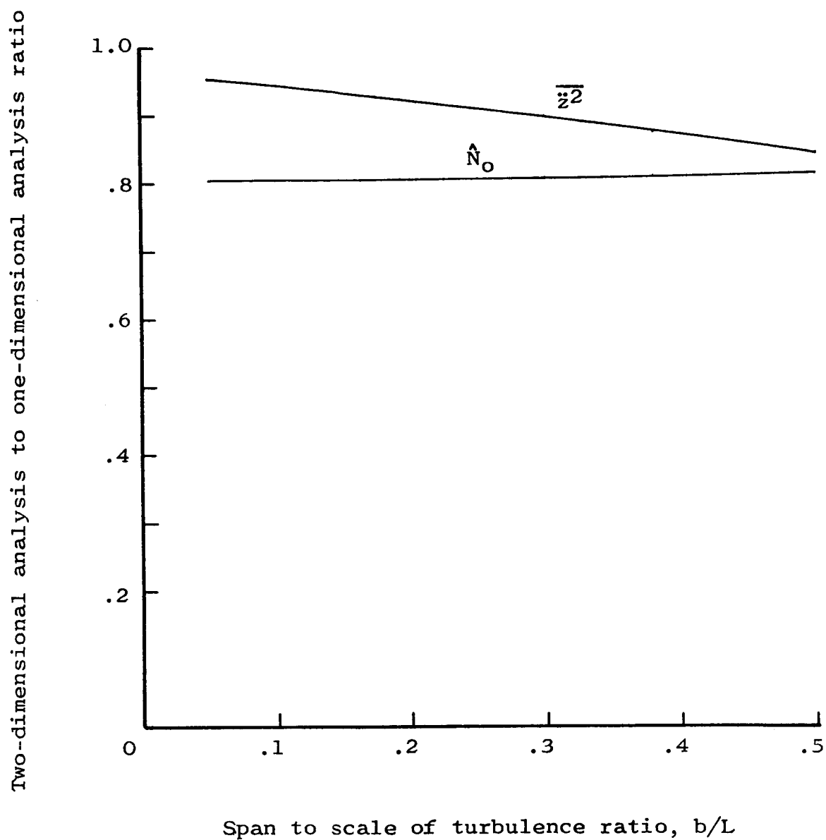
Figure 5.- Reduction of rigid body acceleration mean-square value and \hat{N}_o given by two-dimensional analysis variation with b/L .
