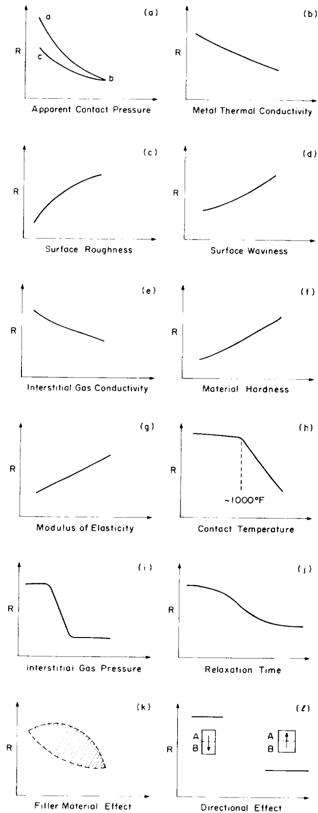
Fig. 2 Parameters Influencing Overall Thermal Contact Resistance
