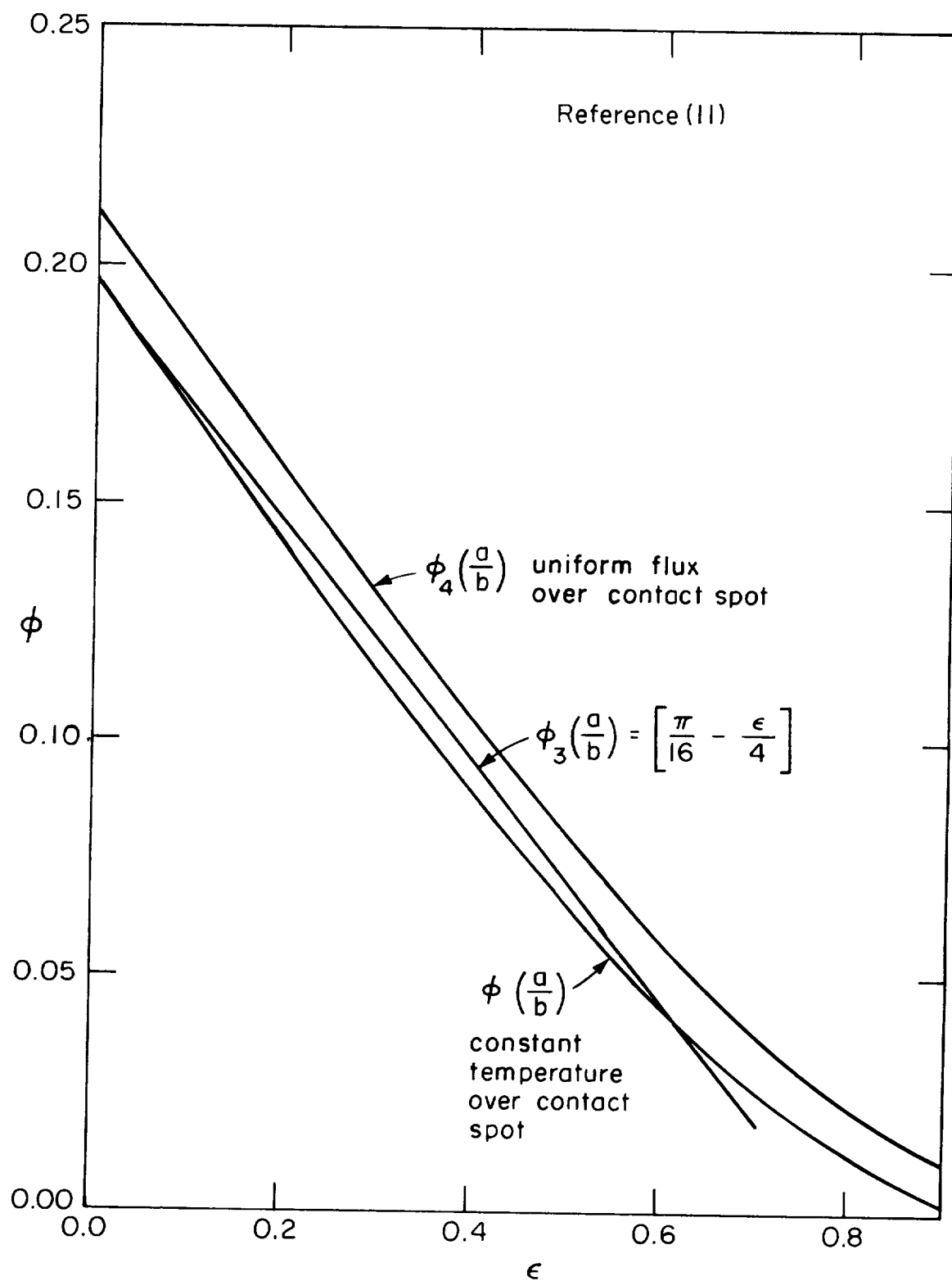
Fig. 12 Geometric Factor for Symmetric Contact
