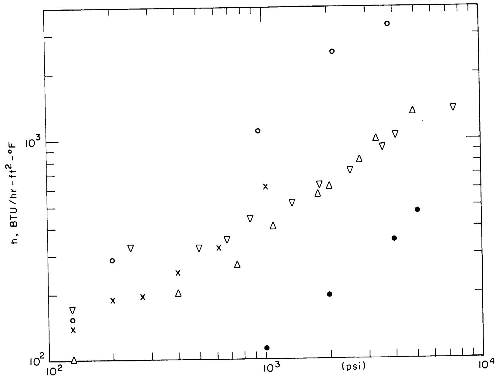
Fig. 32 Thermal Conductance Data vs. Apparent Pressure
