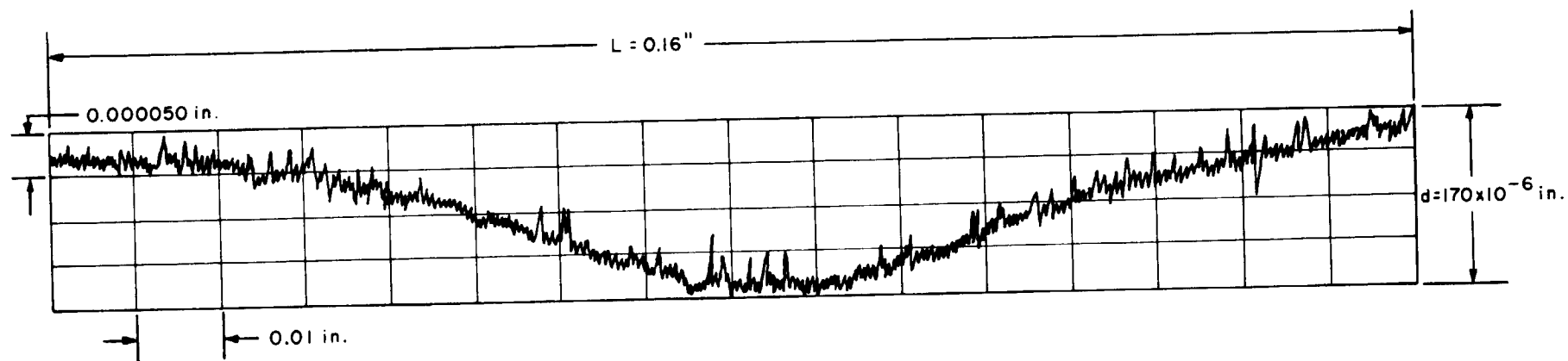
Fig. 6 Typical Trace Showing Waviness and Roughness
