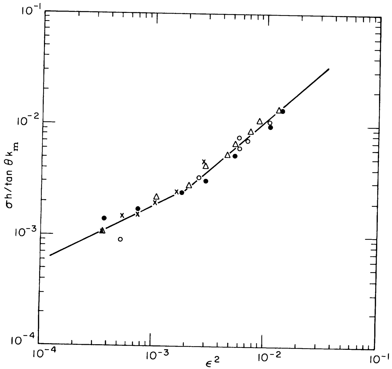
Fig. 33 Thermal Conductance Number vs. Area Ratio
