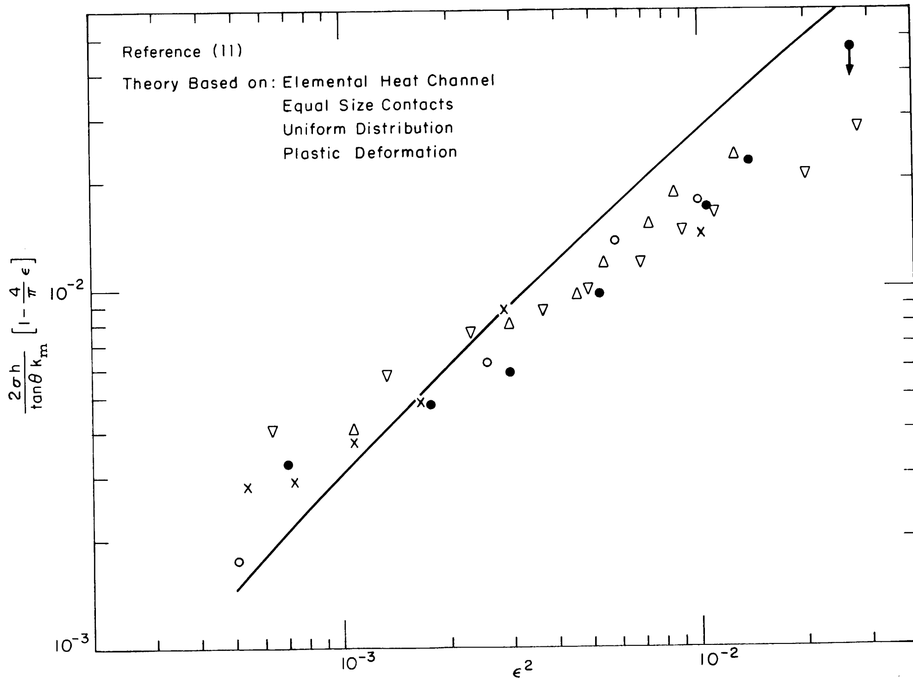
Fig. 34 Thermal Conductance Number vs. Area Ratio
