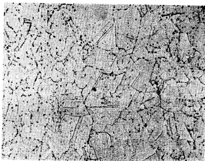
FIGURE 32. MICROSTRUCTURAL STUDY OF VARESTRAINT SPECIMENS SHOWING EFFECT OF THERMAL TREATMENT C AT 1850 F ON 0.040-INCH MATERIAL
