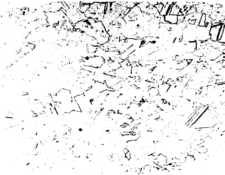
FIGURE 24. MICROSTRUCTURE OF AS-RECEIVED MATERIAL; Heat 6394
