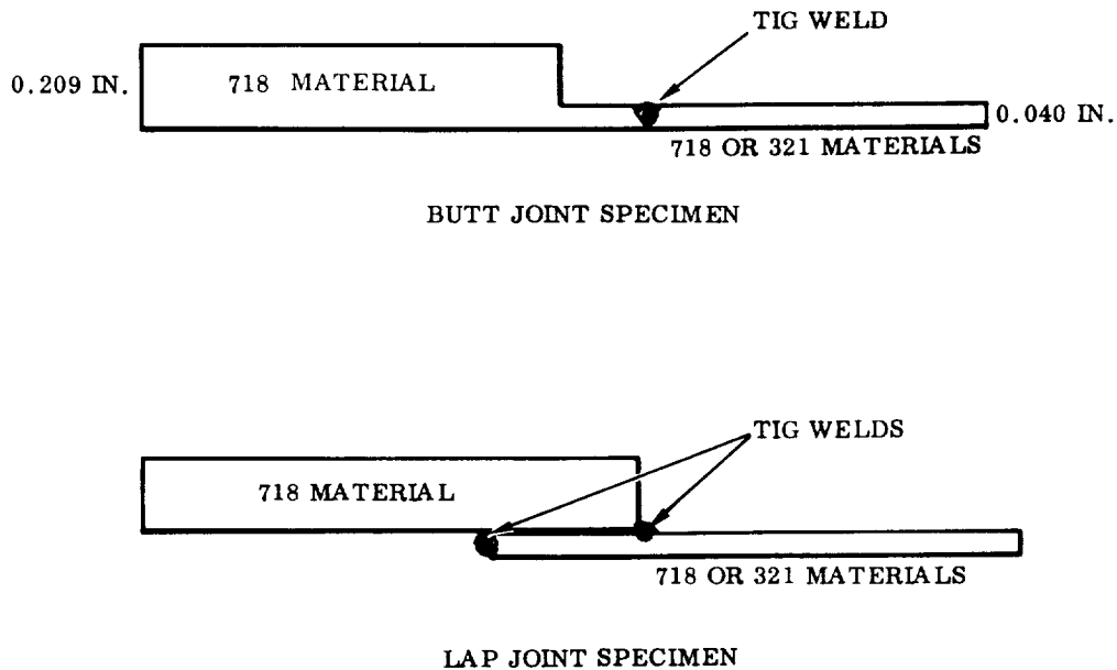
FIGURE 70. TENSILE AND FATIGUE SPECIMEN CONFIGURATION: Phase II Evaluation
