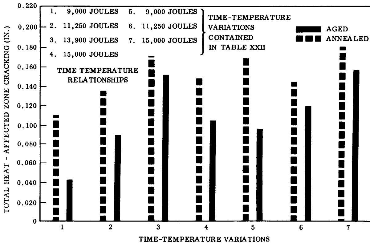
FIGURE 80. VARESTRAINT TESTING TO DETERMINE CRACKING SENSITIVITY OF 0.209-INCH MATERIAL IN RELATION TO VARIATIONS IN ENERGY INPUT
