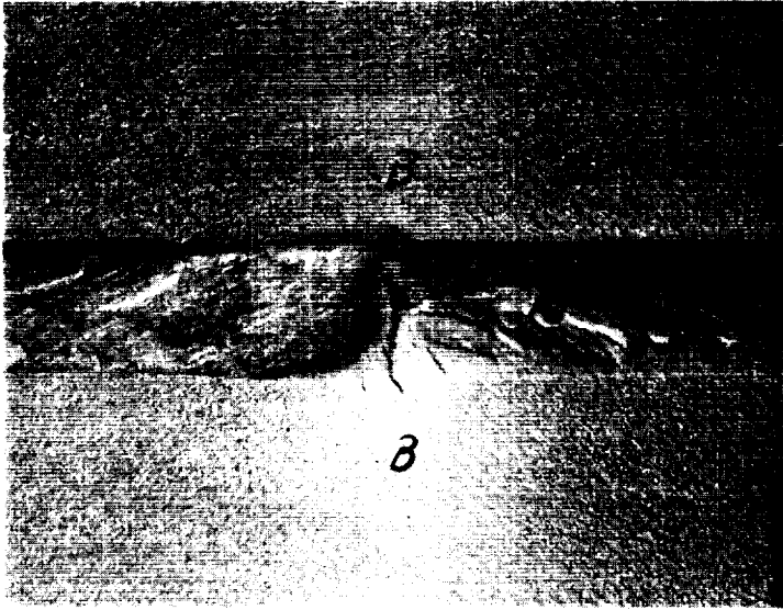
Macrograph showing typical cracking pattern in the 0.040-inch Inconel 718 Vareststraint specimens.
