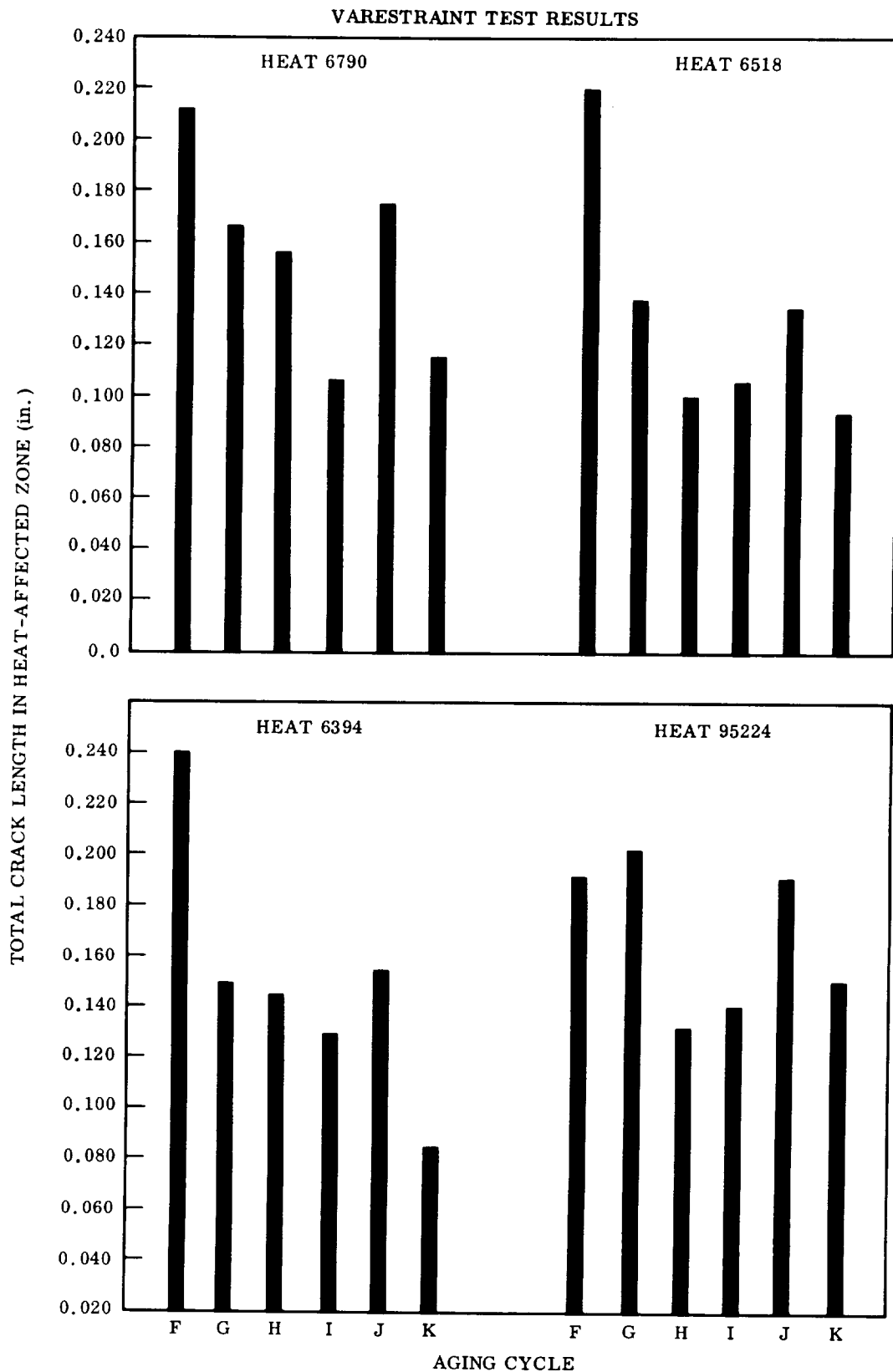
FIGURE 20. EFFECT OF ABBREVIATED AGING CYCLE ON VARESTRAINT TEST RESULTS; 0.209-Inch Material at 1850 F
