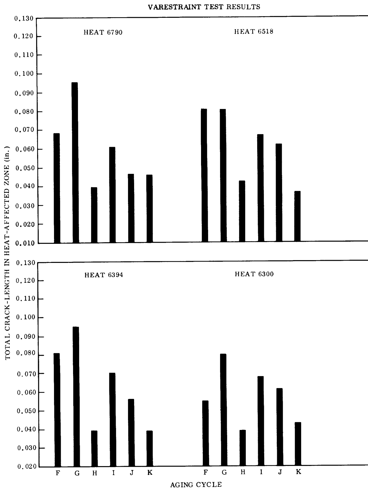
FIGURE 17. EFFECT OF ABBREVIATED AGING CYCLE ON VARESTRAINT TEST RESULTS; 0.040-Inch Material at 1850 F
