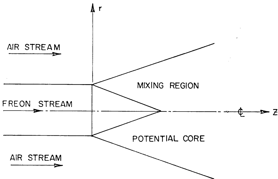
FIGURE I.1 FLOW SYSTEM
