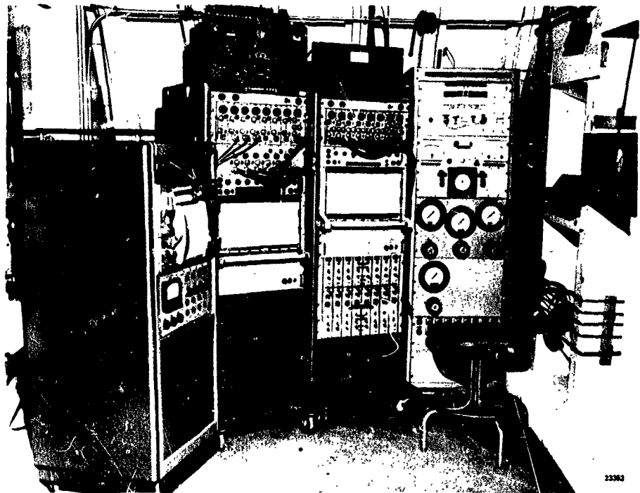
Figure 36 - Task 3 Hot Gas Test Control Panel
