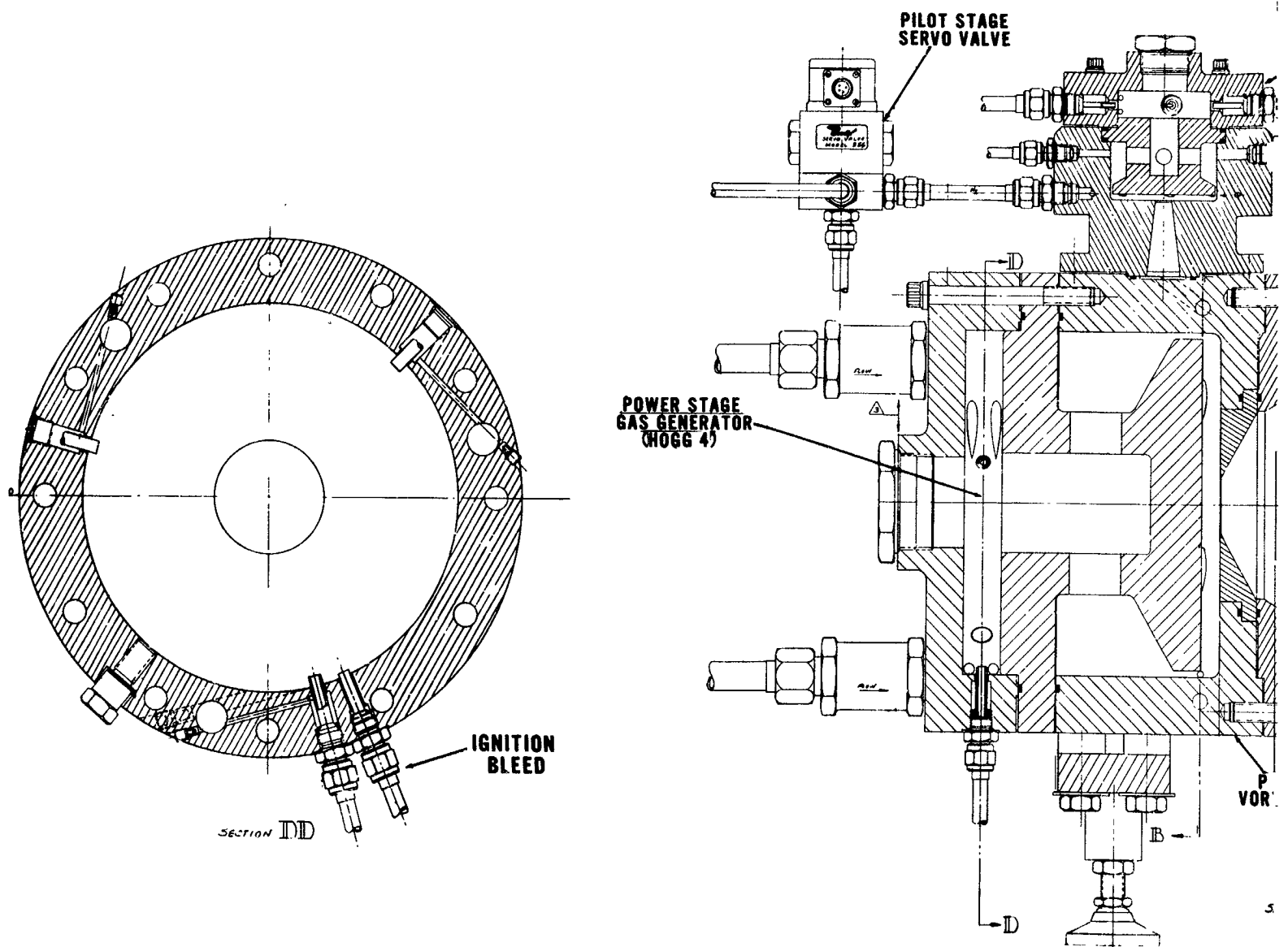
Figure 33 - Task 3 Two-Stage
