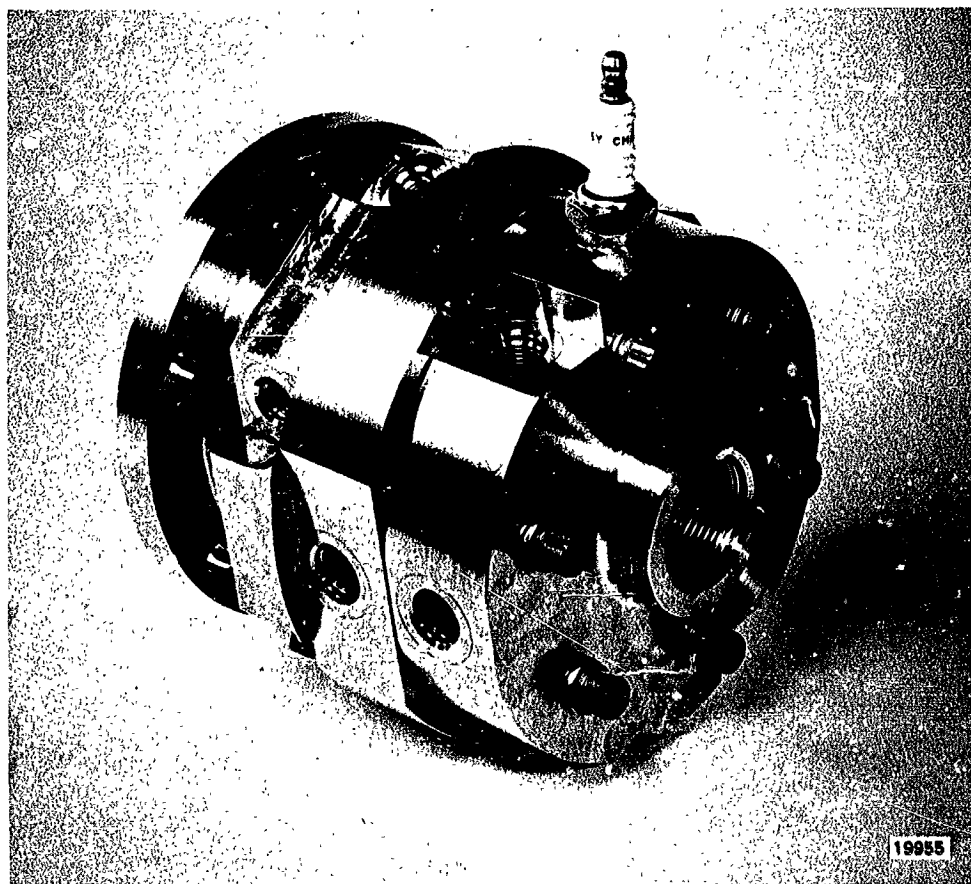
Figure 20 - HOGG3 Assembled
