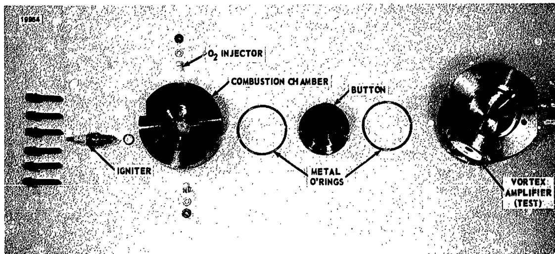
Figure 19 - HOGG3 Disassembled
