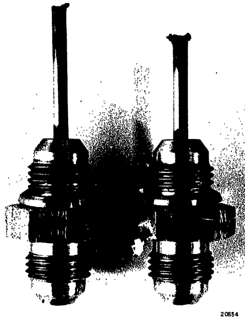
Figure 26 - Stainless Steel Injectors After Test
