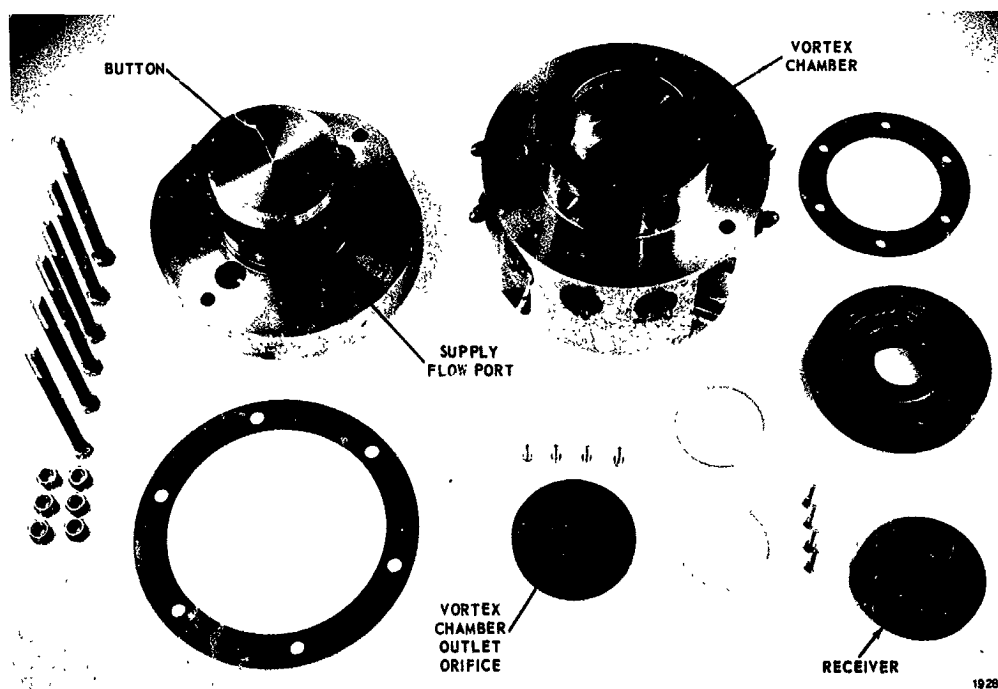
Figure 4 - Phase 1 Vortex Amplifier - Disassembled
