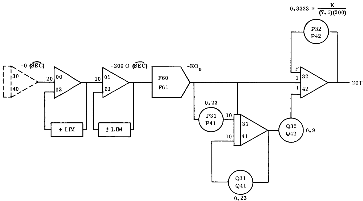
Figure 6-3. Control Loop for Twin 2 DOF CMG's
