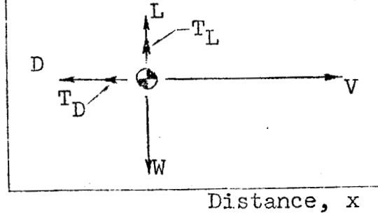
Fig. 2 Orientation of Force and Velocity Vectors for Deceleration
