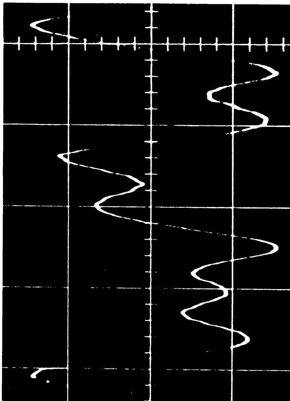
Fig. 18 Coating Thickness 200 \mu in. Deep Gap Field 2500 oe (1 x Saturation), 5000 BPI a) Experimental Waveform b) Computed versus Experimental c) Computed Cross-Correlation F. O. M.
