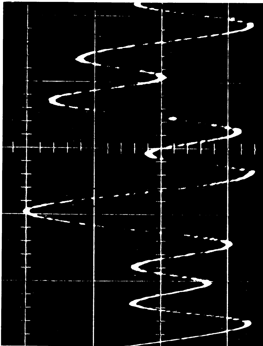
Fig. 8 Coating Thickness 400 \mu in. Deep Gap Field 2250 oe ( 1/2 \times Saturation) 5000 BPI a) Experimental Waveform b) Computed versus Experimental c) Computed Cross-Correlation F. O. M.
