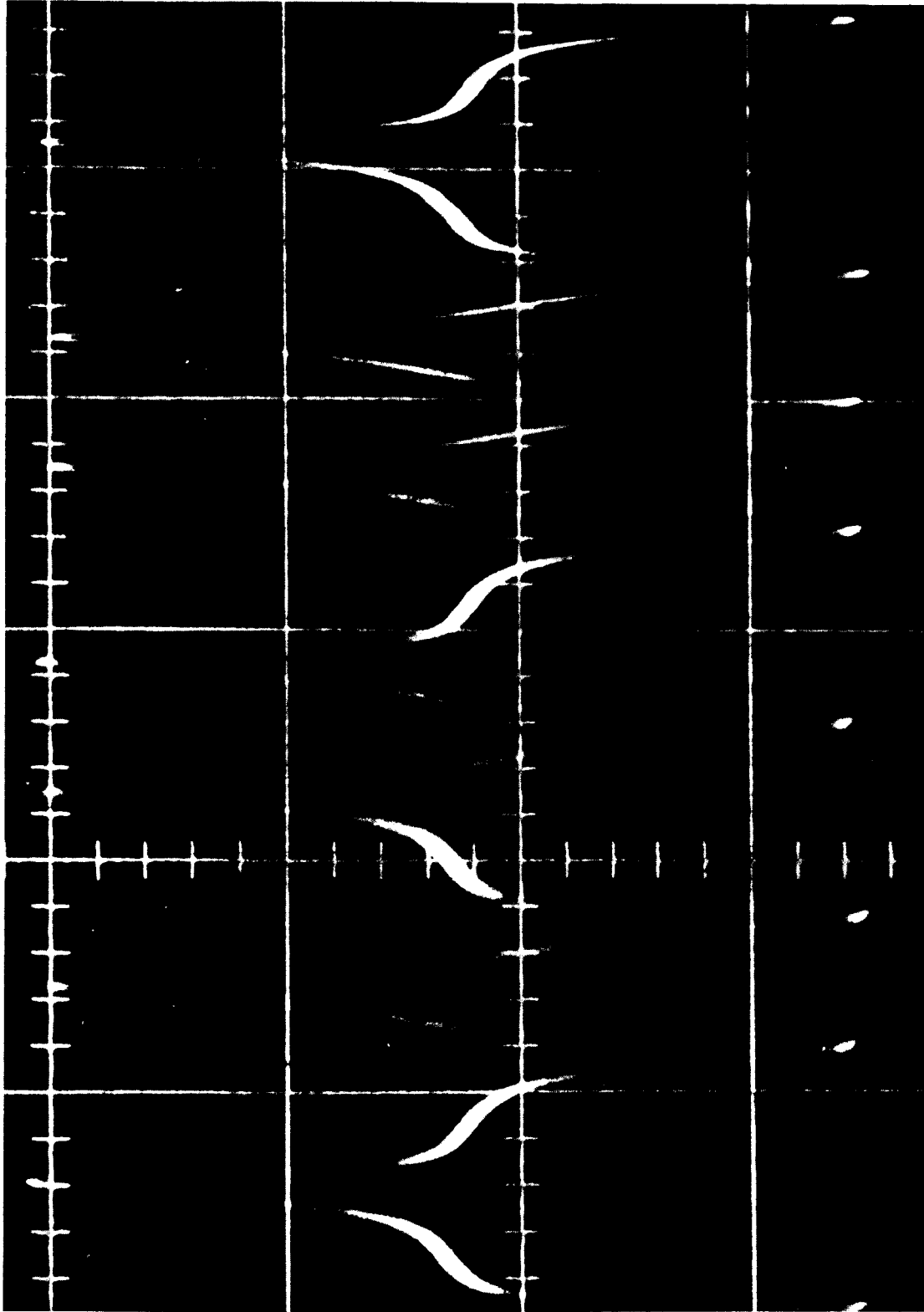
Fig. 5 Coating Thickness 400 \mu in. Deep Gap Field 2250 oe ( 1/2 \times Saturation) 625 BPI a) Experimental Waveform b) Computed versus Experimental c) Computed Cross-Correlation F. O. M
