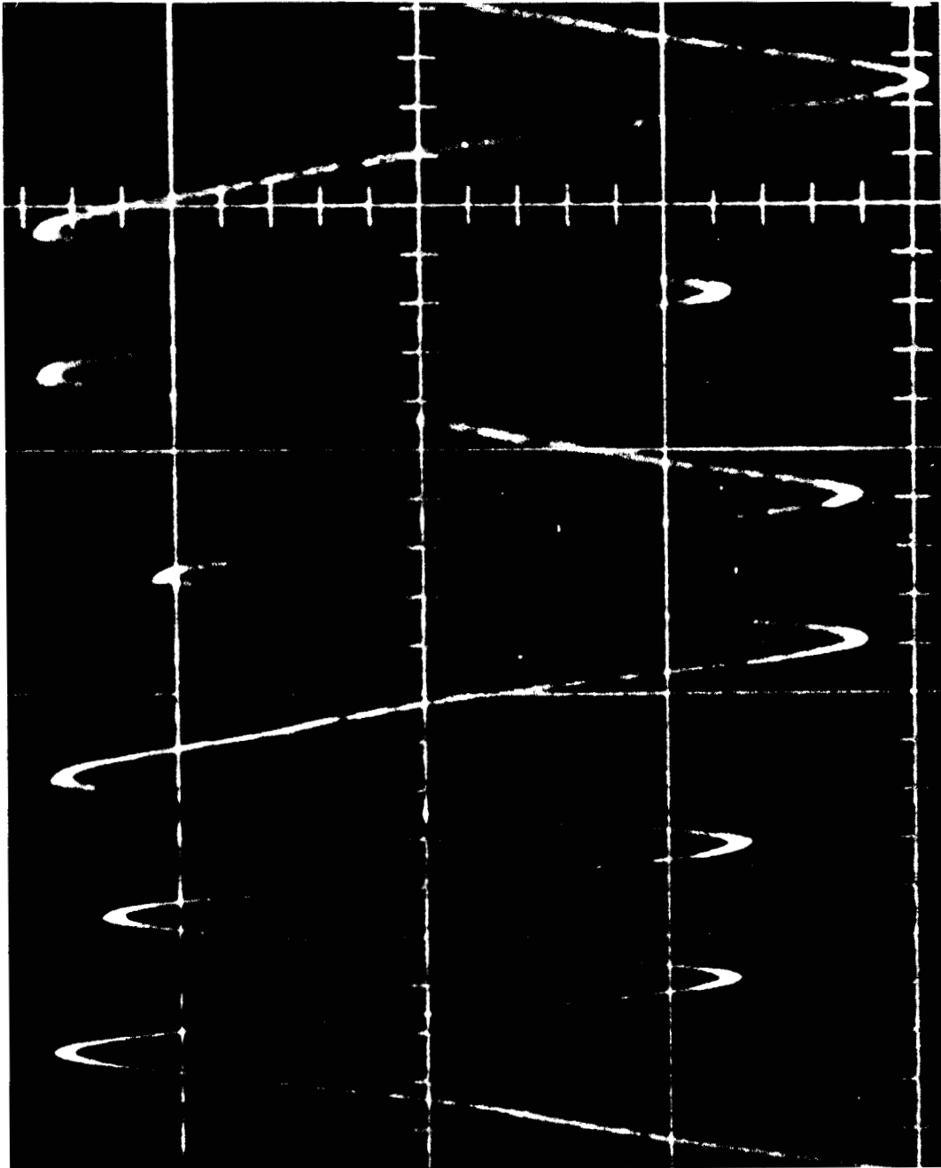
Fig. 7 Coating Thickness 400 \mu in. Deep Gap Field 4500 oe ( 1/2 \times Saturation), 2500 BPI a) Experimental Waveform b) Computed versus Experimental c) Computed Cross-Correlation F. O. M.
