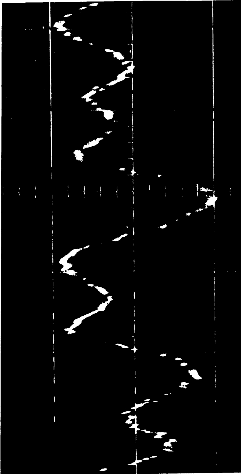
Fig. 13 Coating Thickness 400 \mu in. Deep Gap Field 1100 oe (1/4 x Saturation) 7500 BPI a) Experimental Waveform b) Computed versus Experimental c) Computed Cross-Correlation F. O. M.
