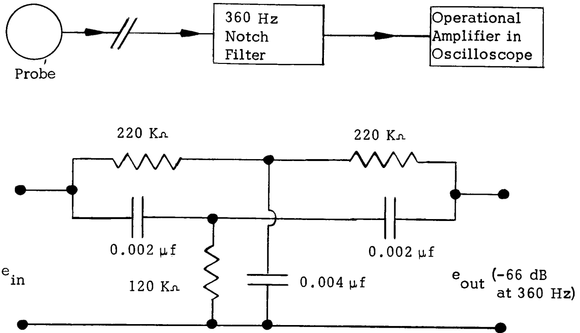
Fig. IV-3. Diamagnetic Probe Circuit and Associated Notch Filter Circuitry.
