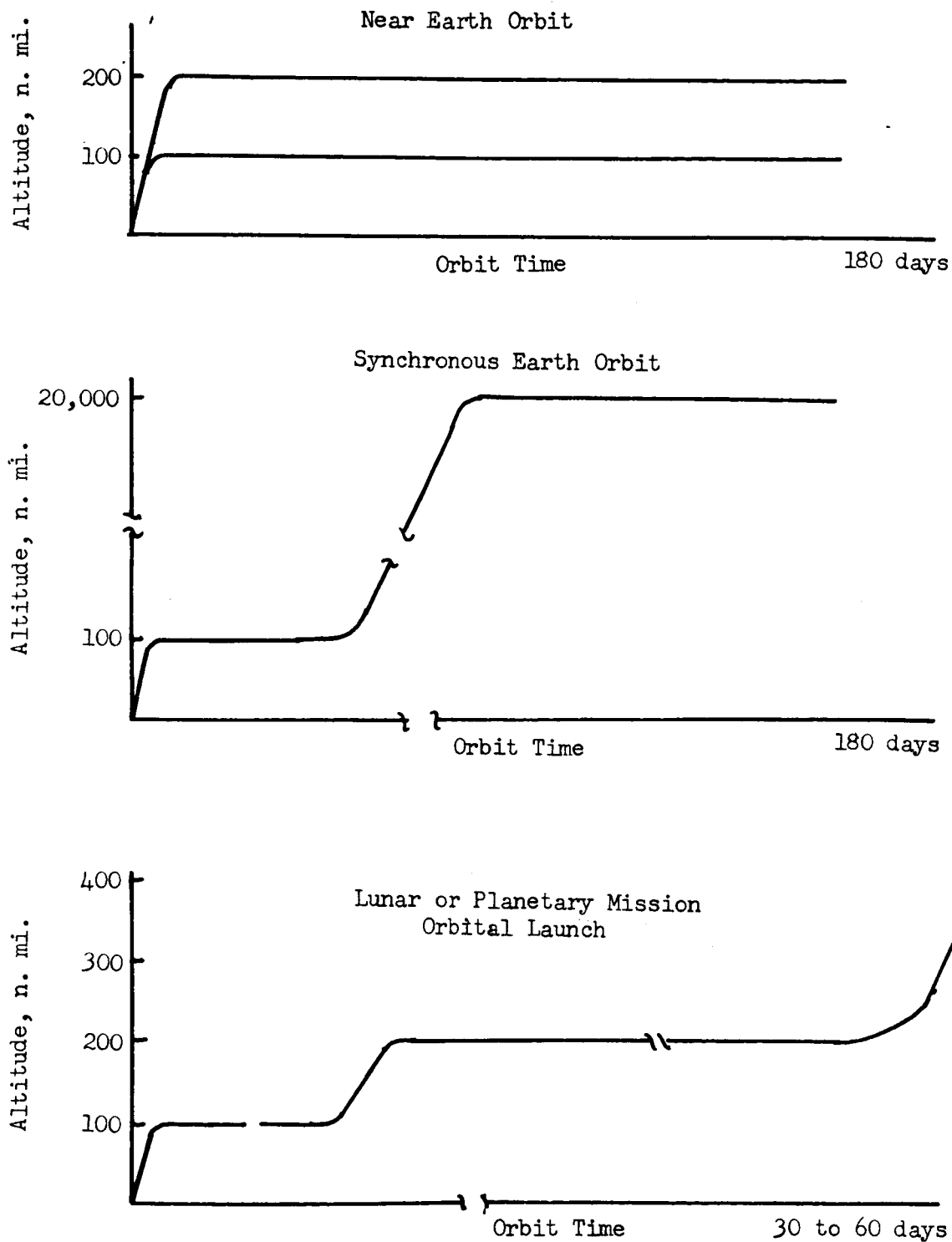
Figure 2. Basic Mission Profiles
