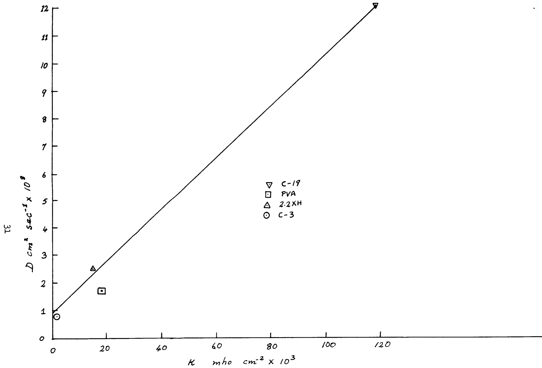
Figure 21. The Diffusivity of Zincate in Separators Versus the Conductivity of the Separator in Electrolyte
