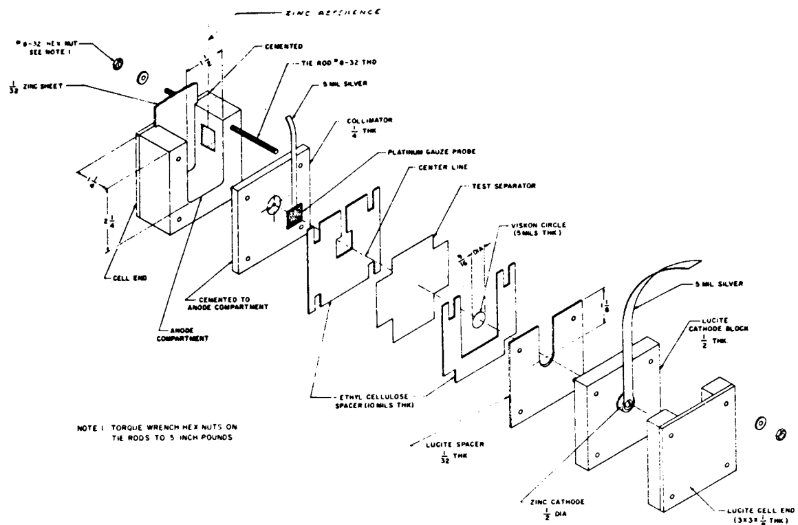
Figure 32 Zinc Penetration Test Cell (Exploded View)
