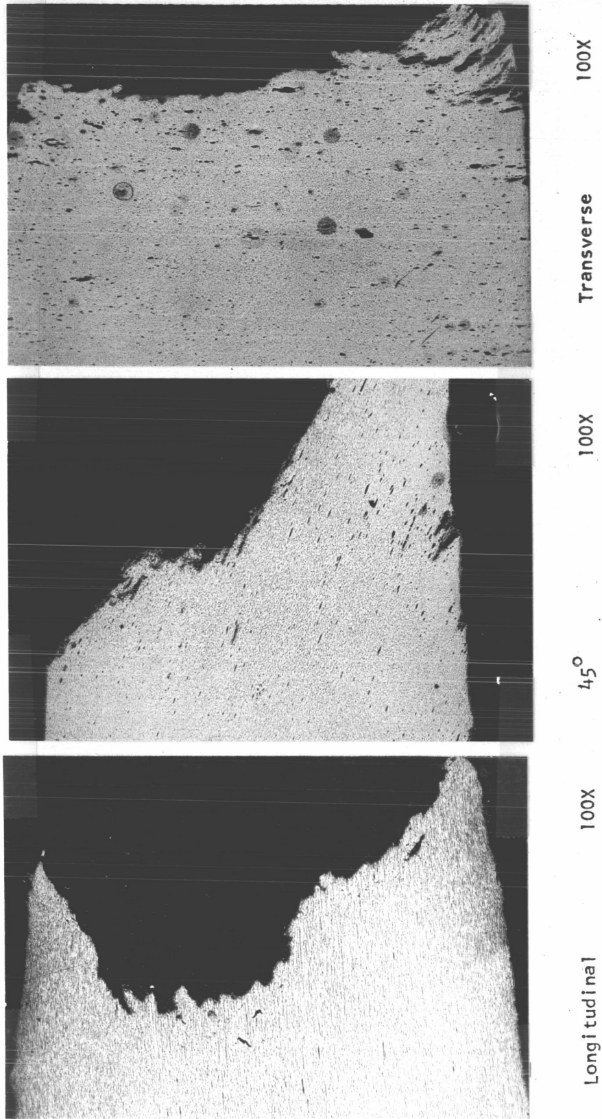
Figure 6. Internal Cracking as a Function of Specimen Orientation for Commercial TD Nickel Bar Tensile Tested at 2000°F.
