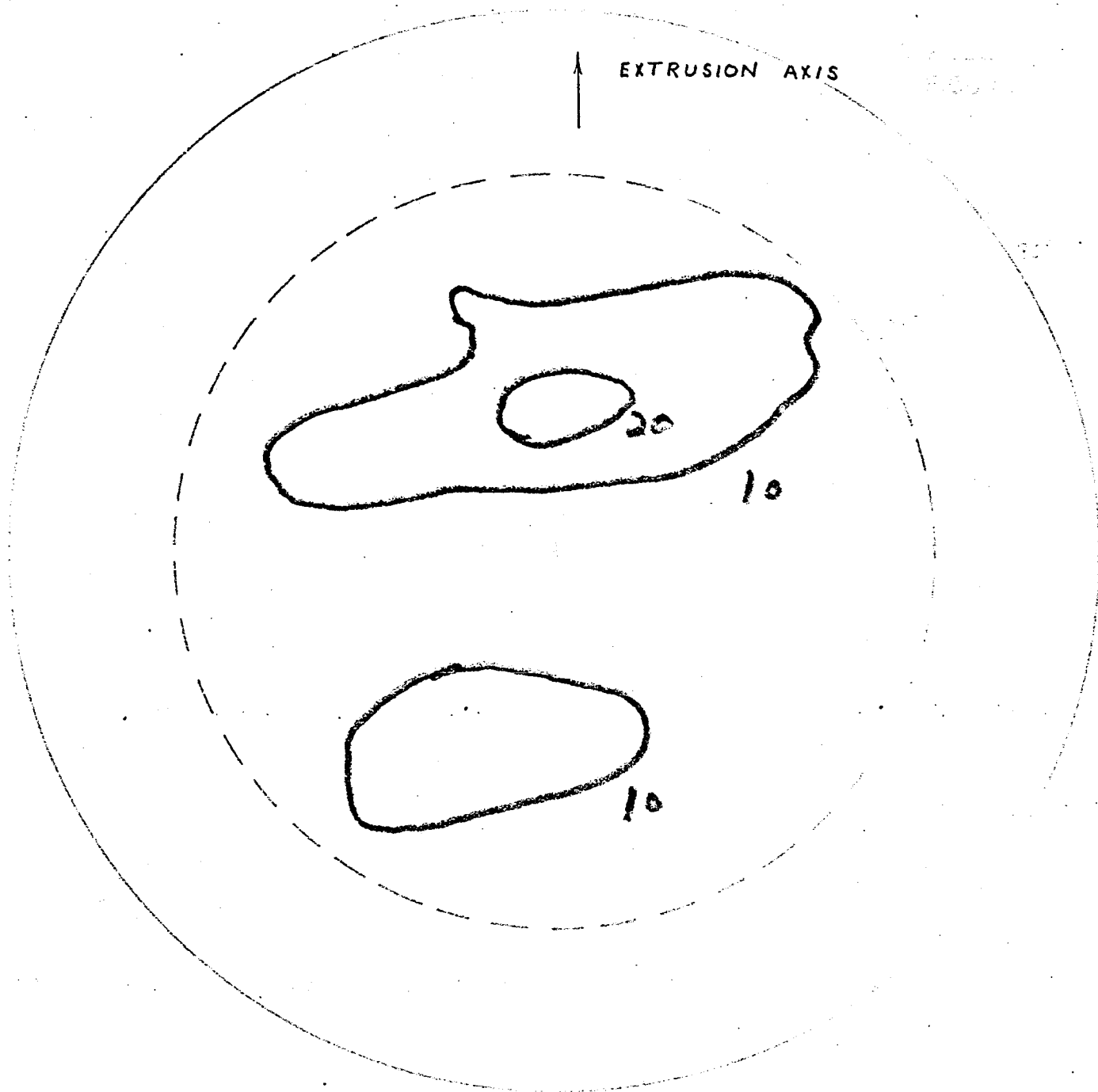
Figure 27. Pole Figure of As-Extruded TD Nickel.
