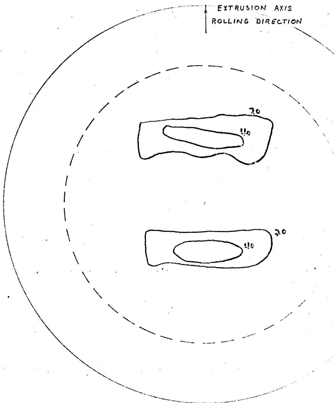
Figure 28. Pole Figure of As-Extruded TD Nickel Rolled 37% in Longitudinal Direction.
