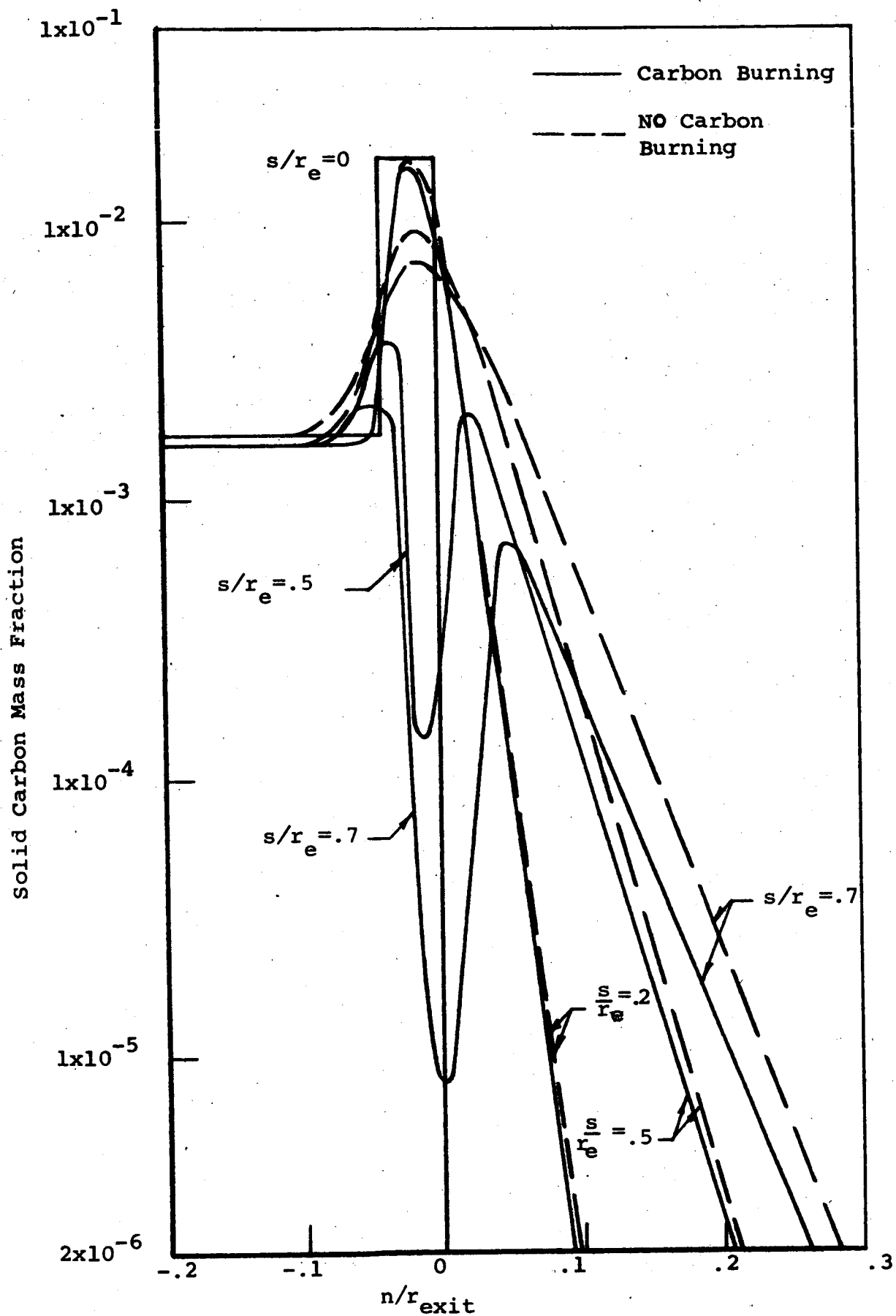
FIGURE 22 - DISTRIBUTION OF SOLID CARBON IN FLOW FIELD WITH AND WITHOUT CARBON BURNING CASE A -83-
