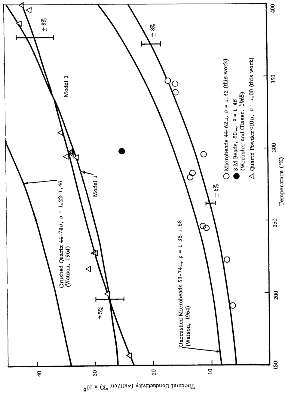
FIGURE IV-5 EFFECTIVE THERMAL CONDUCTIVITY OF GLASS BEADS AND QUARTZ POWDER
