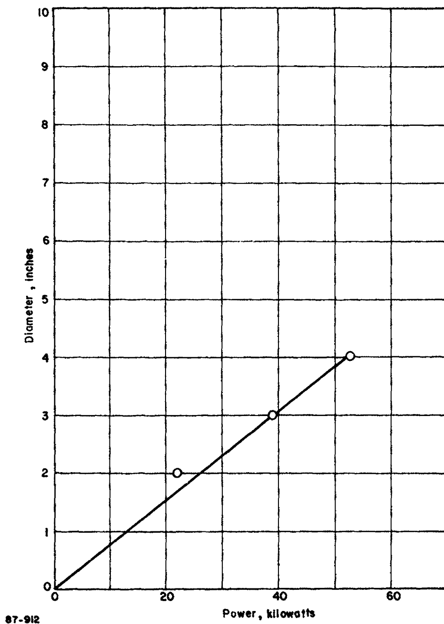
Figure 30 ANODE DIAMETER VERSUS MAXIMUM POWER FOR RADIATION-COOLED MPD THRUSTORS
