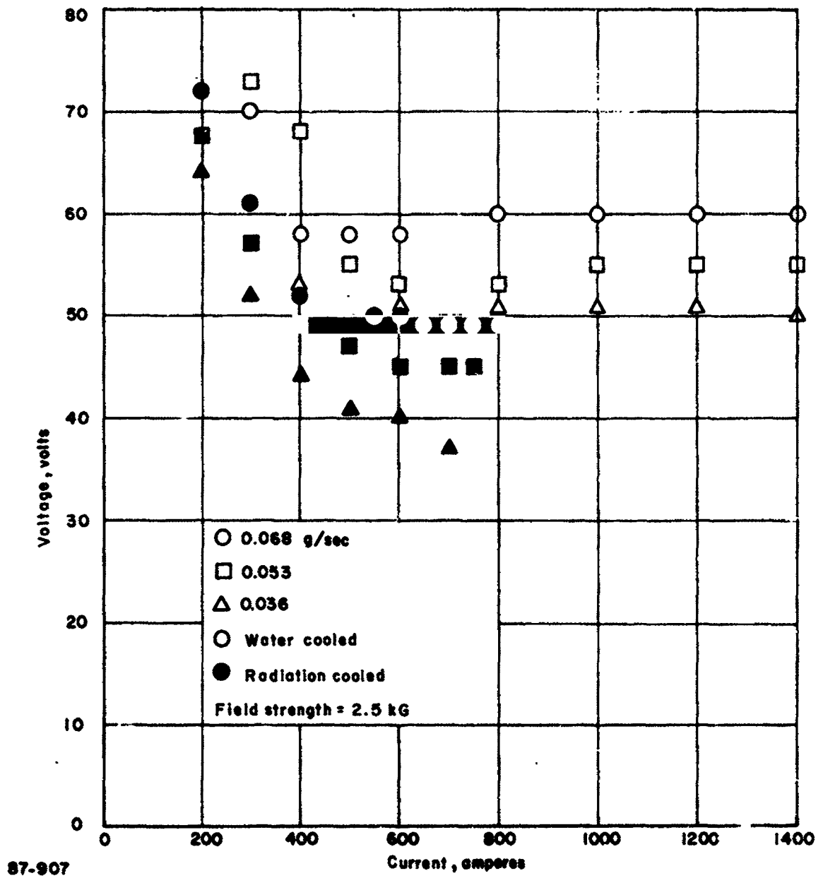
Figure 25 ARC VOLTAGE VERSUS CURRENT FOR THE 3-INCH-DIAMETER WATER-COOLED AND RADIATION-COOLED THRUSTOR
