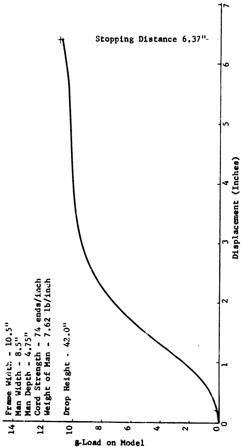
FIGURE 15 LOAD ATTENUATION CURVE FOR TEST SPECIFICATION, PROPOSAL "B" FILAMENT WOUND CONCEPT
