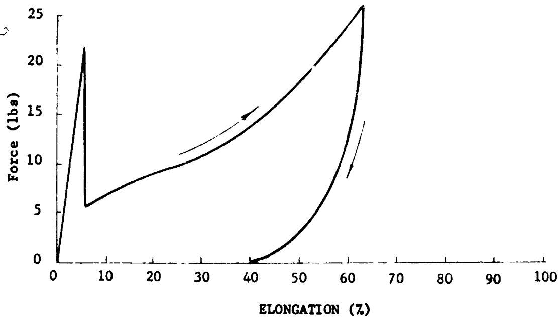
FIGURE 4 STATIC LOAD - ELONGATION OF A LOAD BEARING ASSEMBLY, WOVEN TAPE CONCEPT
