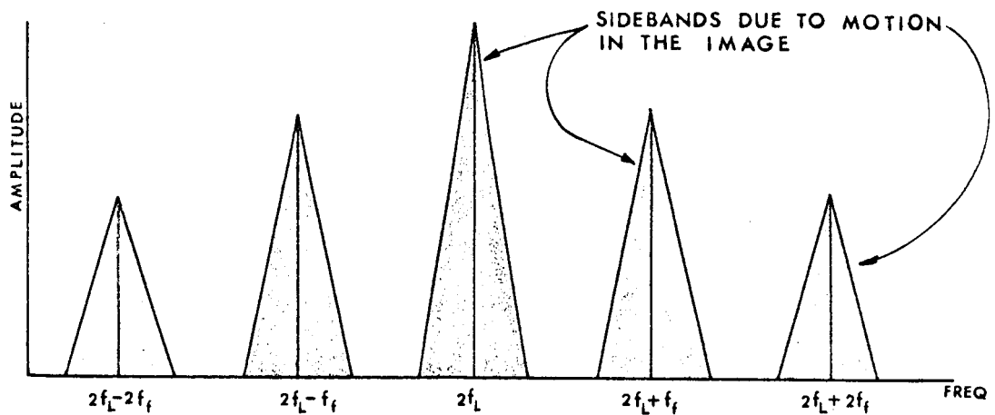
DETAIL OF A TYPICAL REGION OF THE VIDEO SPECTRUM SHOWING THE EFFECT OF MOTION IN THE IMAGE
