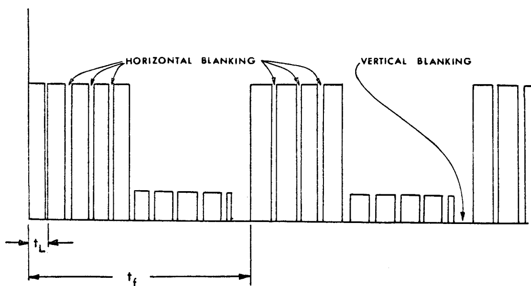
TIME DOMAIN VIDEO OUTPUT FOR ABOVE IMAGE
