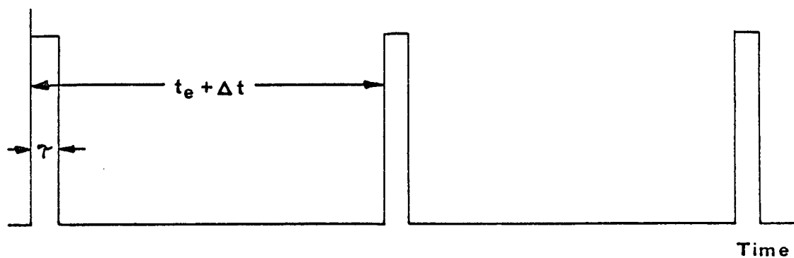
TIME DOMAIN OUTPUT RESULTING FROM SCANNING THE IMAGE BELOW NEGLECTING BLANKING
