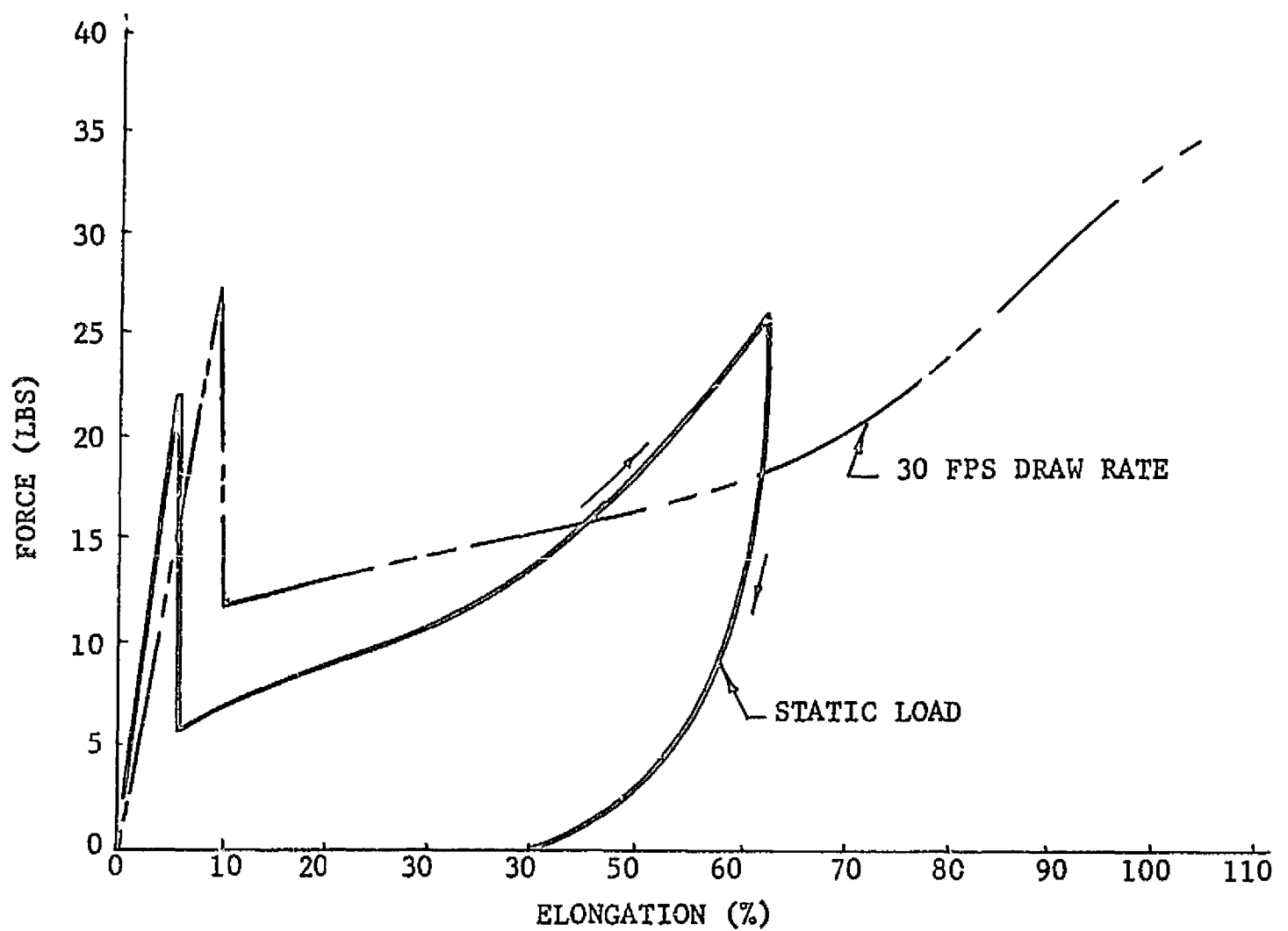
FIGURE 6 ELONGATION OF A LOAD BEARING TAPE ASSEMBLY FORMIC ACID TREATED NYLON
