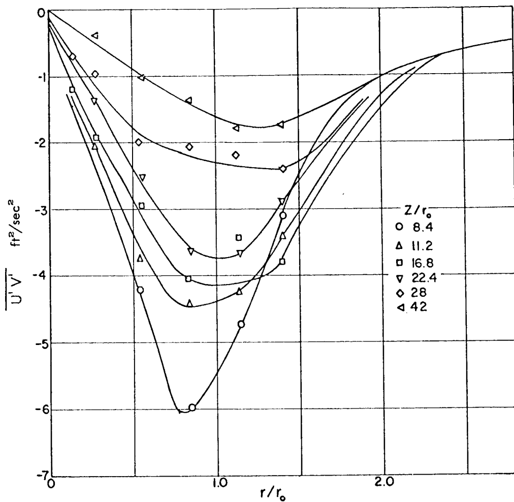
FIGURE V - 1 - 22 TURBULENT SHEAR STRESS PROFILES FOR \frac{U_o}{U_i} = 3.4
