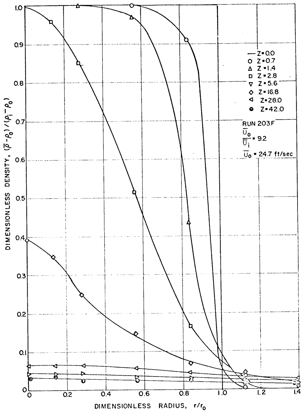
FIGURE V - 2 - 10 CONCENTRATION PROFILES, \frac{U_0}{U_i} = 9.2 , \frac{\rho_0}{\rho_i} = 0.25
