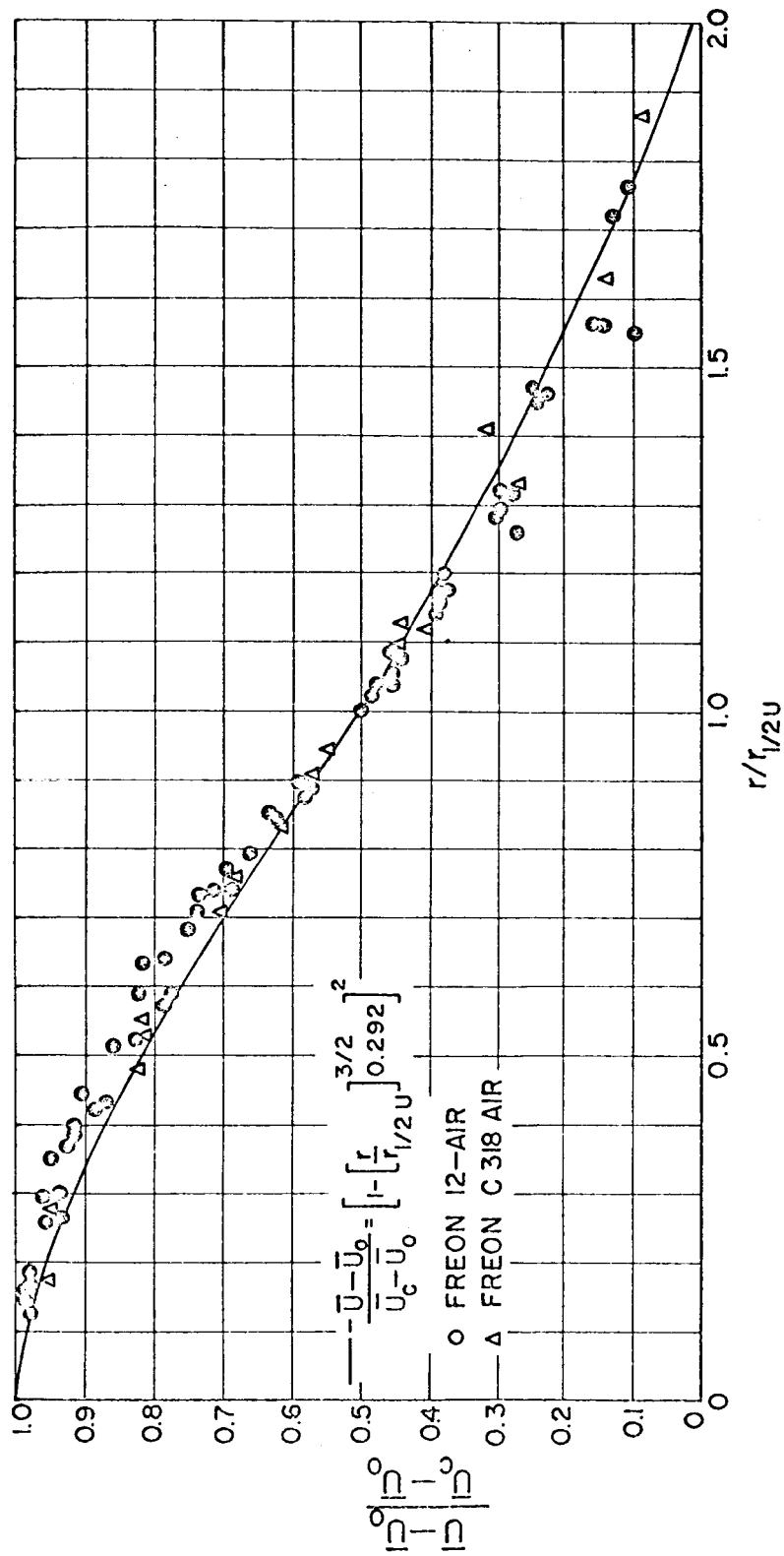
FIGURE V - 2- 21 SIMILARITY PLOT OF VELOCITY PROFILES FOR ALL HETEROGENEOUS CASES
