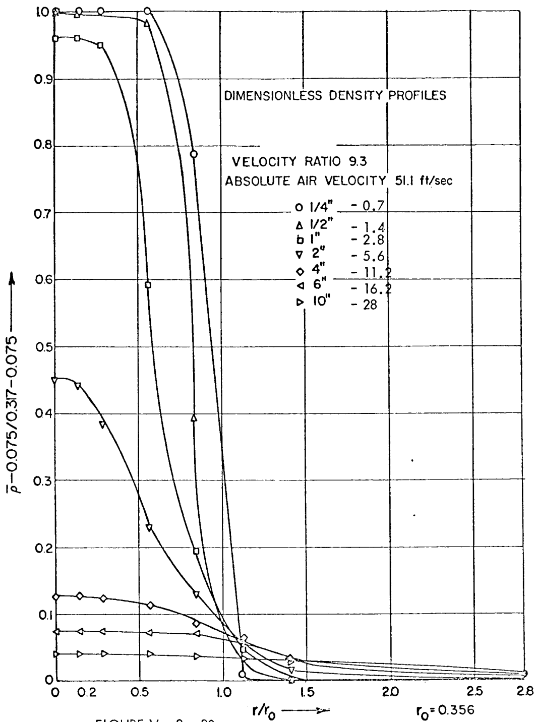
FIGURE V - 2 - 30 CONCENTRATION PROFILES, \frac{U_o}{U_i} = 9.3, \frac{\rho_o}{\rho_i} = 0.25
