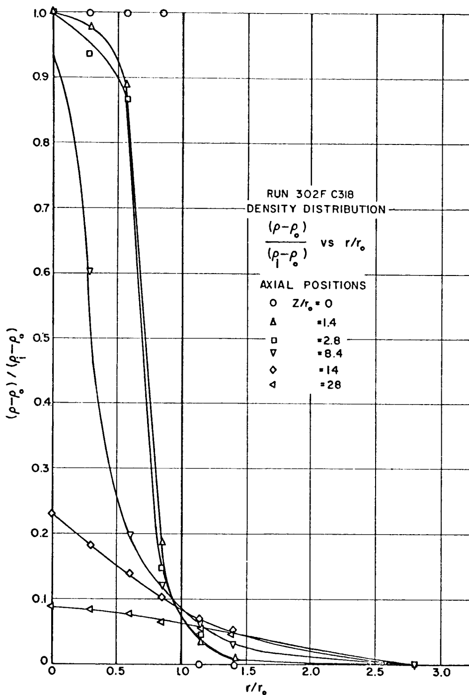
FIGURE V - 2 - 19 CONCENTRATION PROFILES, \frac{U_o}{U_i} = 5.8 , \frac{\rho_o}{\rho_i} = 0.143
