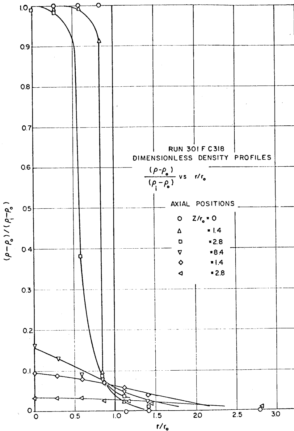
FIGURE V - 2 - 18 CONCENTRATION PROFILES, \frac{U_o}{U_i} = 11.5 \quad \frac{\rho_o}{\rho_i} = 0.143
