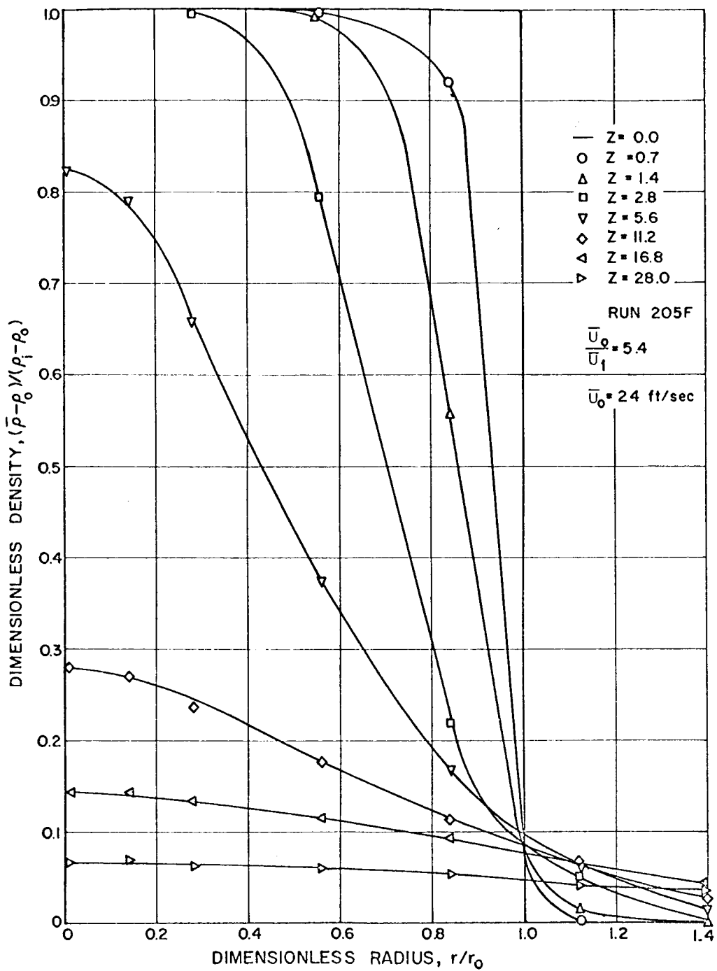
FIGURE V - 2 - 12 CONCENTRATION PROFILES, \frac{U_o}{U_i} = 5.4, \frac{\rho_o}{\rho_i} = 0.25
