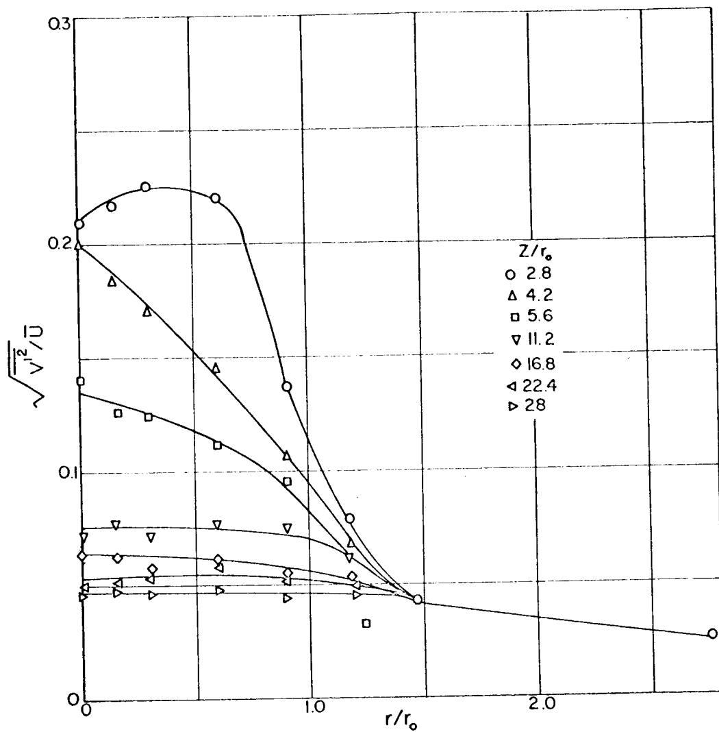
FIGURE V - 1 - 18 RADIAL TURBULENCE INTENSITY PROFILES FOR \frac{\bar{u}_o}{\bar{u}_i} = 8
