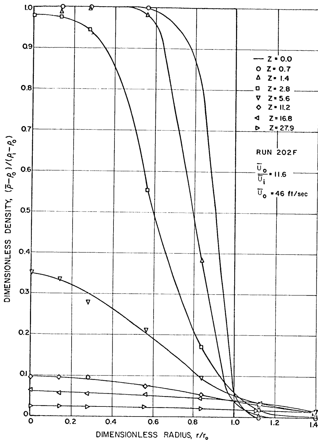
FIGURE V - 2- 9 CONCENTRATION PROFILES, \frac{U_o}{U_i} = 11.6, \frac{c_o}{\rho_i} = 0.25
