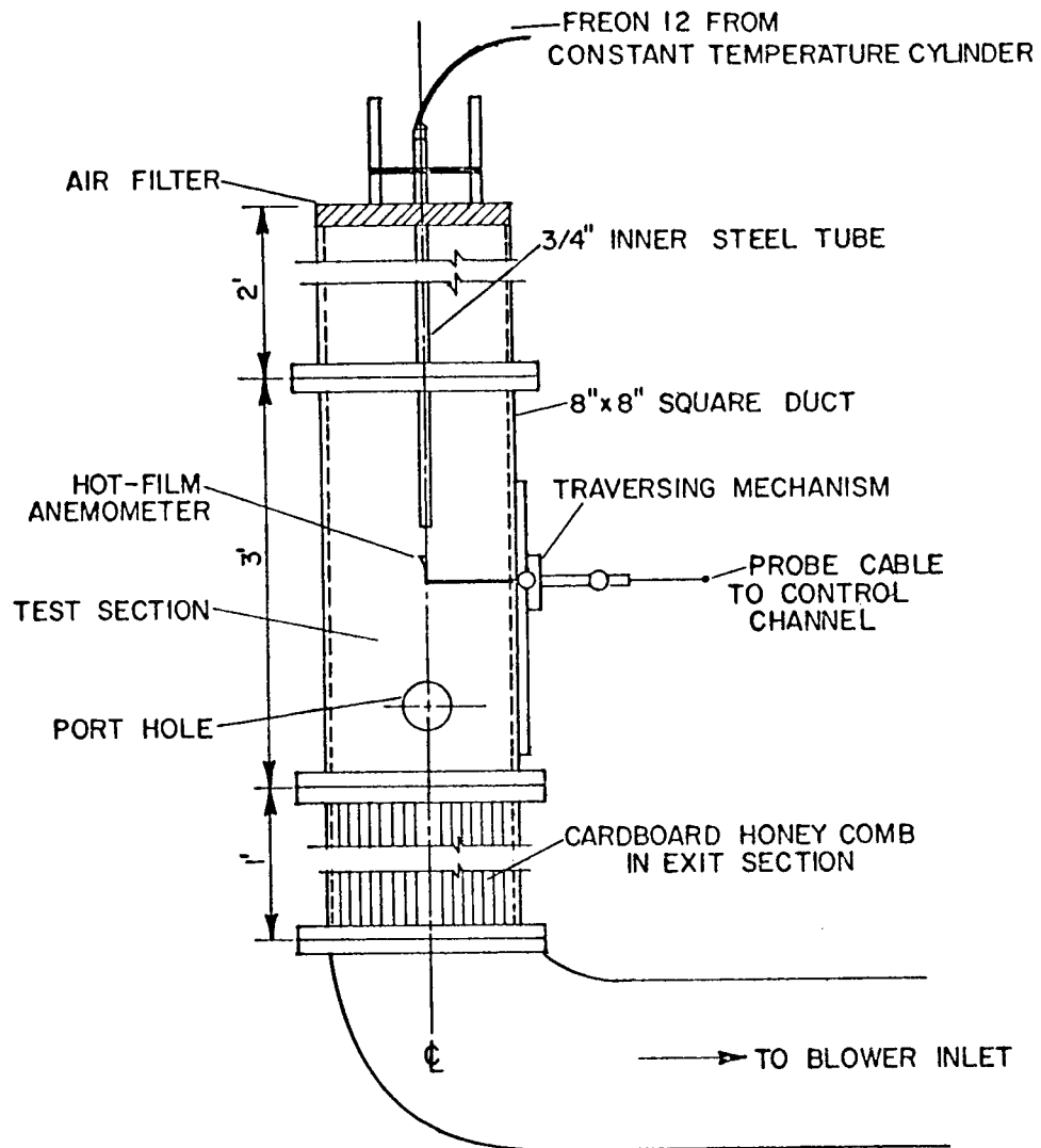
TEST SECTION FIGURE IV - 1 - 1
