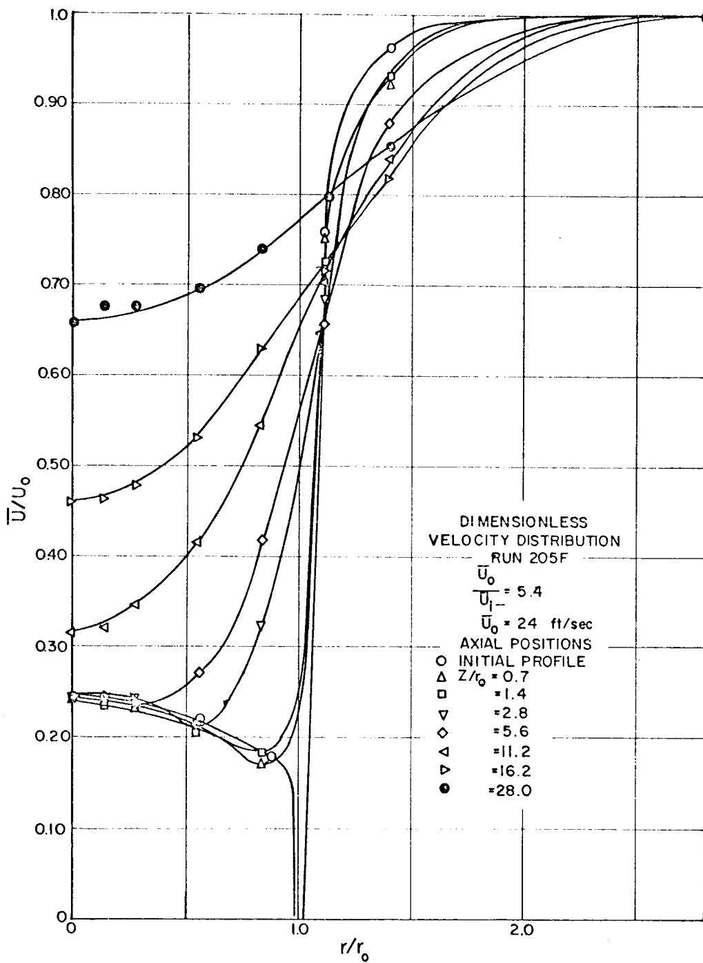
FIGURE V - 2 - 5 DIMENSIONLESS VELOCITY PROFILES, HETEROGENEOUS, \frac{\bar{U}_0}{\bar{U}_i} = 5.4, \bar{U}_0 = 24 \text{ ft/sec}, \frac{\rho_0}{\rho_i} = 0.25
