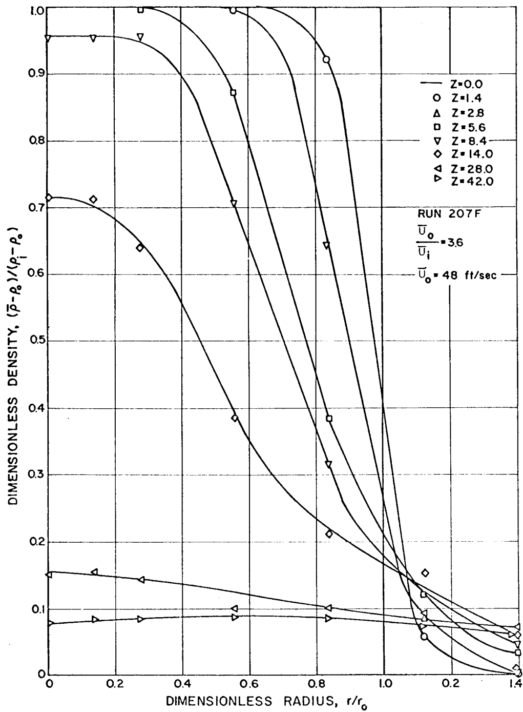
FIGURE V - 2 - 14 CONCENTRATION PROFILES, \frac{U_o}{U_i} = 3.6, \frac{\rho_o}{\rho_i} = 0.25
