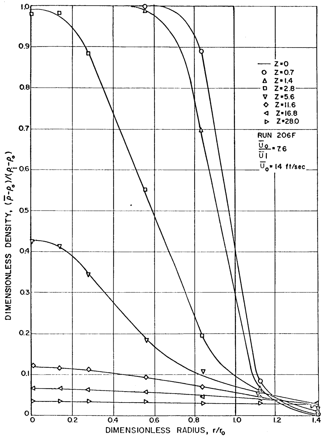
FIGURE V - 2 - 13 CONCENTRATION PROFILES, \frac{U_o}{U_i} = 7.6 , \frac{\rho_o}{\rho_i} = 0.25
