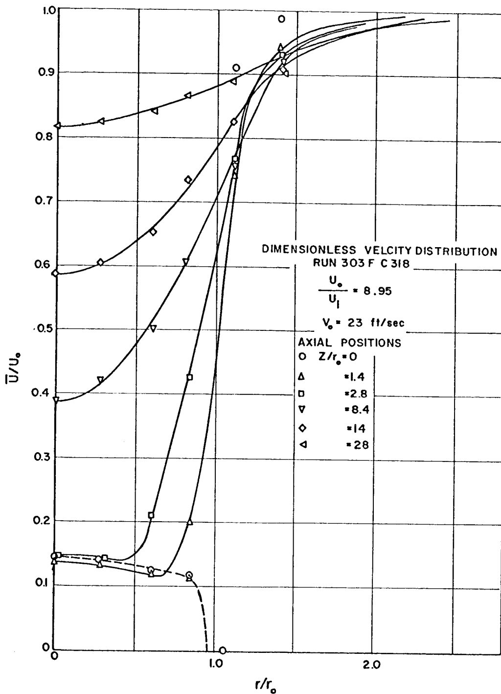
FIGURE V - 2 - 17 DIMENSIONLESS VELOCITY PROFILES, \frac{U_o}{U_i} = 8.9, U_o = 23 \text{ ft/sec} \frac{\rho_o}{\rho_i} = 0.143
