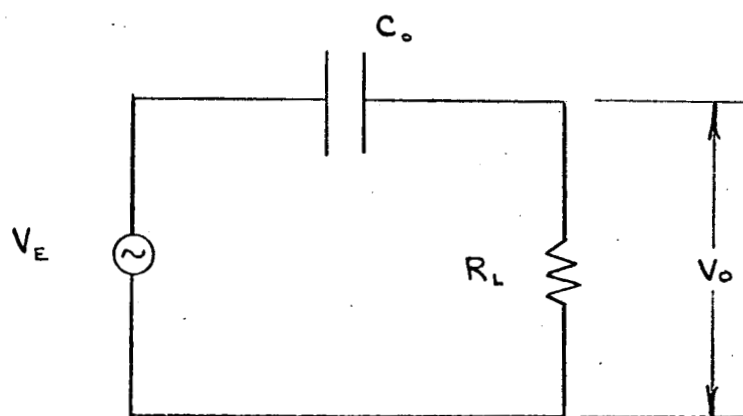
Fig. 34 THEVENIN CIRCUIT
