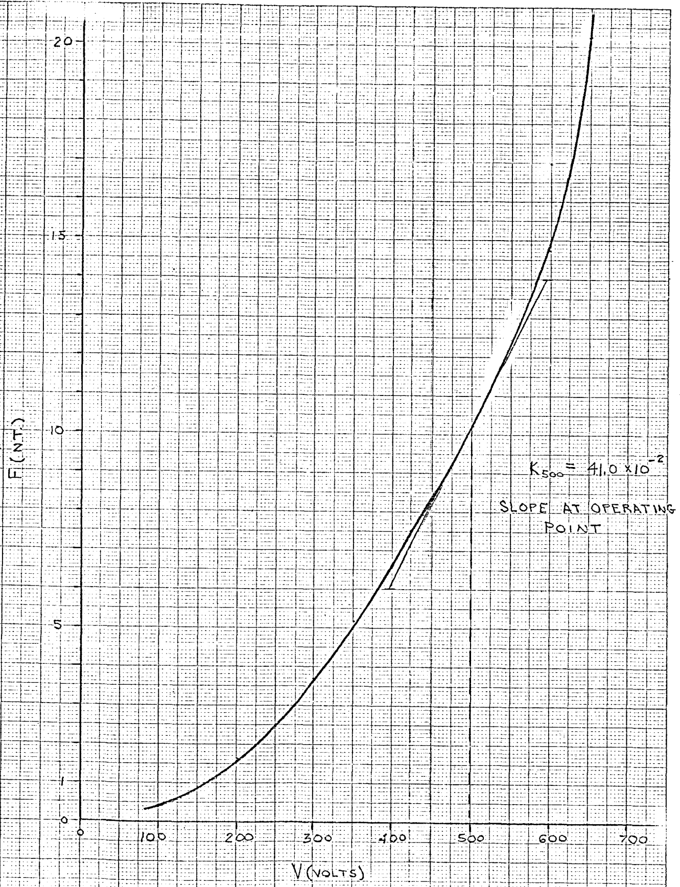
Fig. 9 GRAPHICAL LINEARIZATION OF EQUATION 3 ABOUT AN OPERATING POINT AT 500 VOLTS
