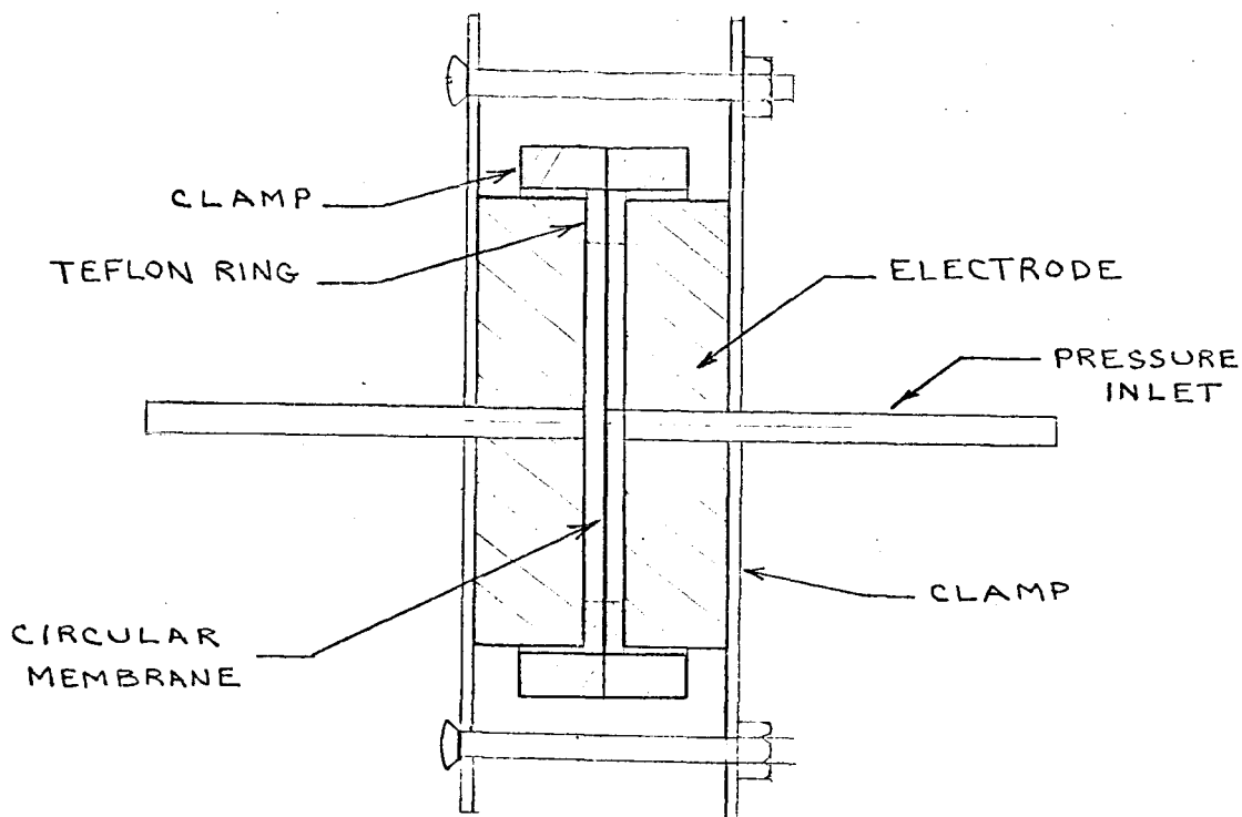
Fig.1. CROSS SECTION OF A CAPACITIVE PRESSURE TRANSDUCER
