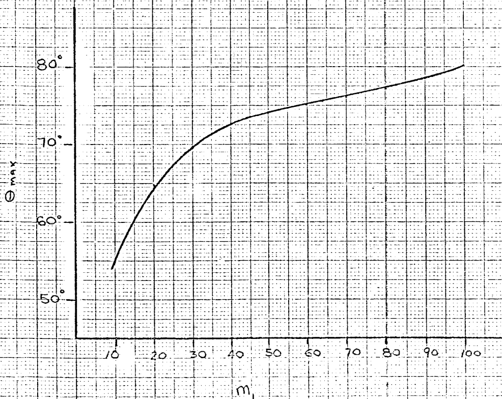
FIG. 13 \Theta_{max} vs. m_1 FOR PHASE LEAD ELEMENT
