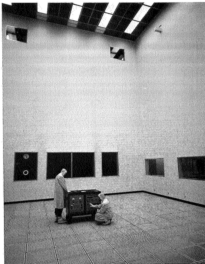
Fig. 5. SADL vertical laminar flow hardware assembly area
