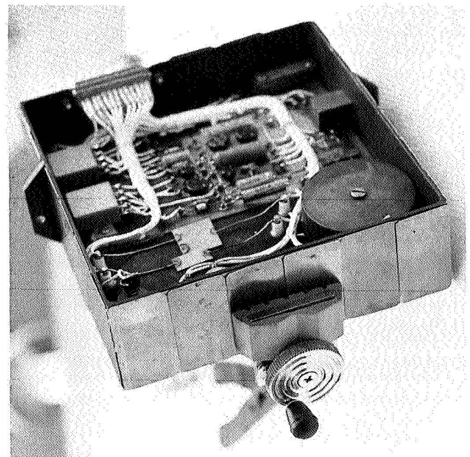
Fig. 1. Non-functional planar assembly (fabricated in the EASL) consisting of stainless-steel coupons and electronic components
