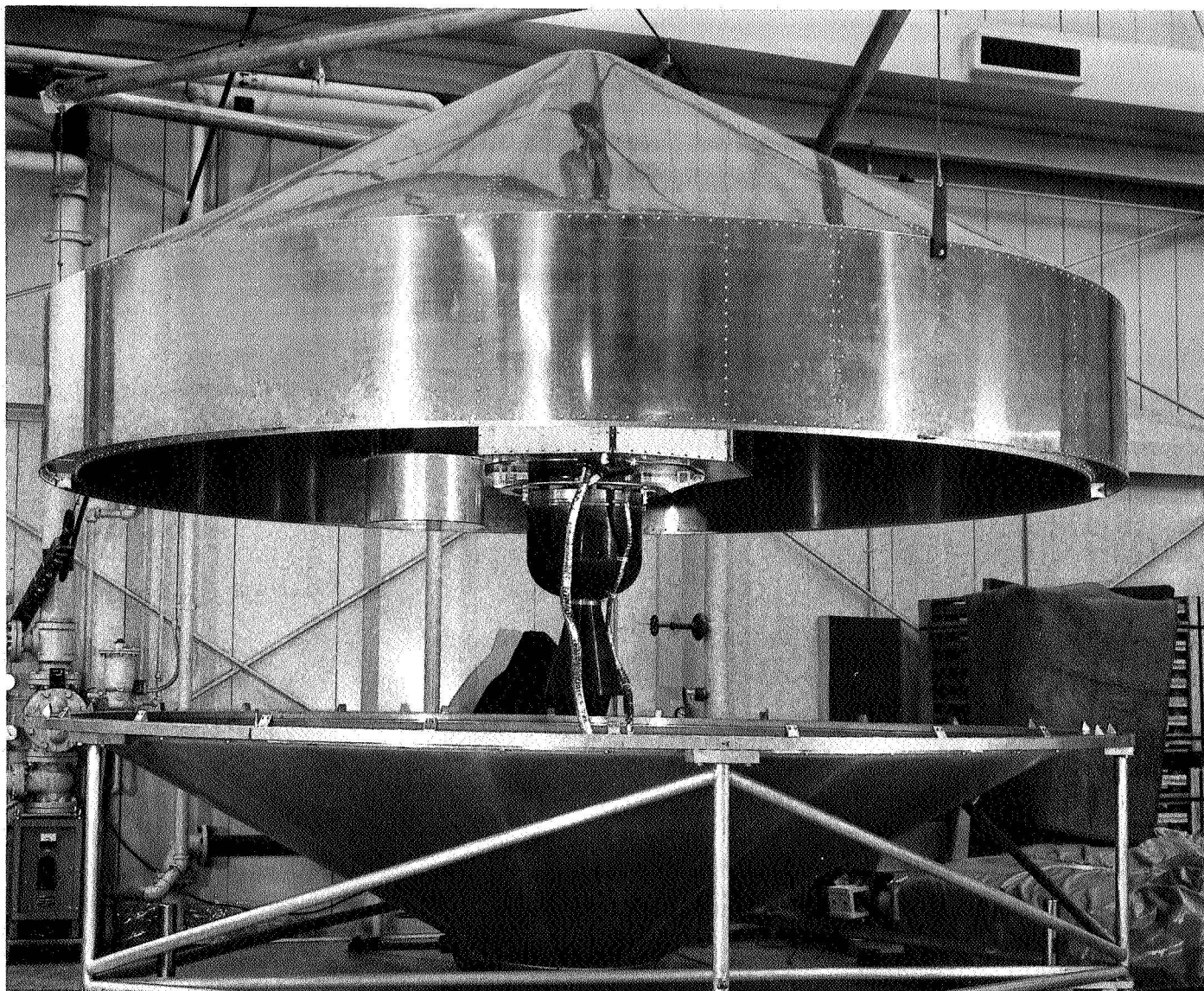
Fig. 6. Capsule mechanical training model (CMTM)
