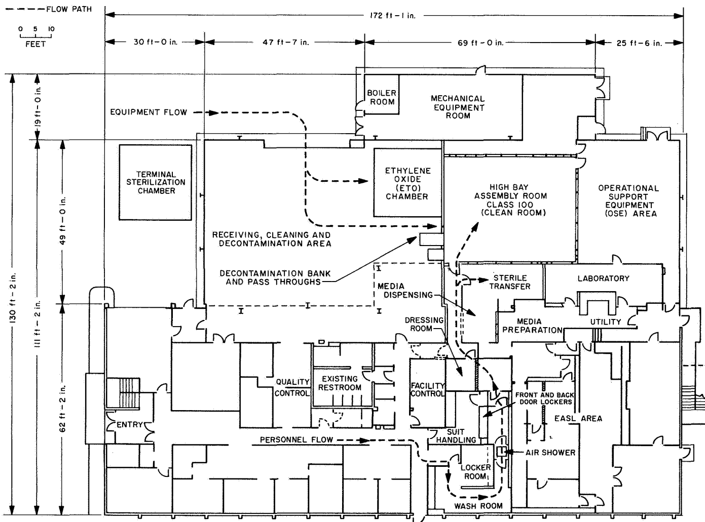
Fig. 4. Floor plan of the SADL facility
