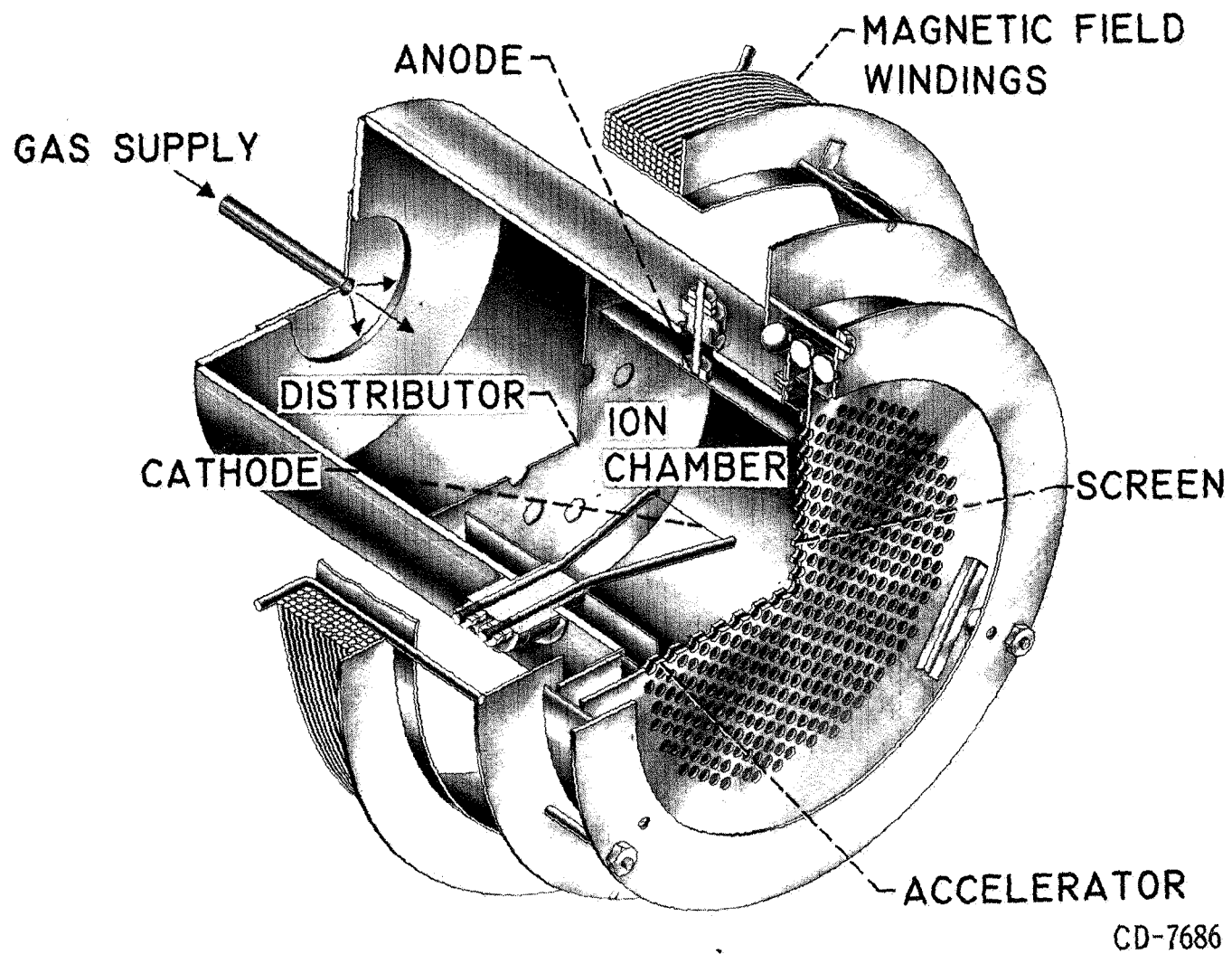
Figure 1. - 10-centimeter-diameter electron-bombardment ion source.
