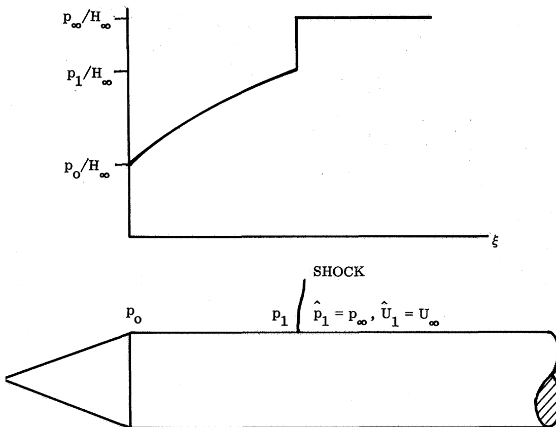
Fig. 3-1 Sketch of Inviscid Terminal-Shock Aerodynamics
