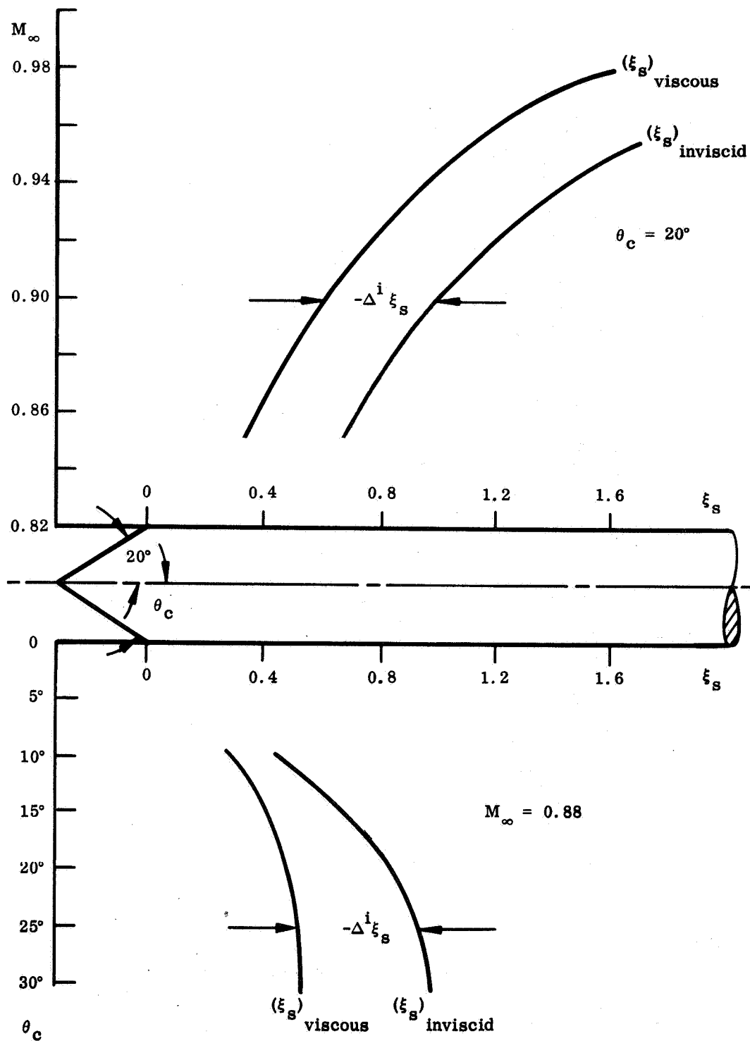
Fig. 3-10 Terminal-Shock Location in Inviscid and Viscous Flow on Cone-Cylinder Bodies at \alpha = 0
