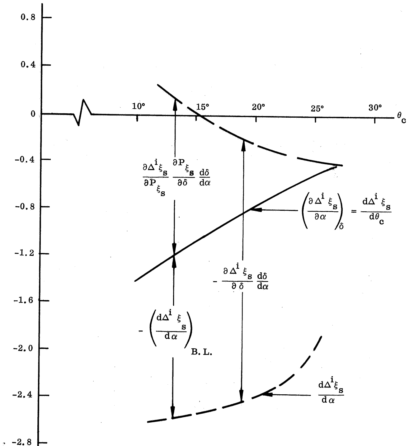
Fig. 3-14 Breakdown of the Angle-of-Attack Effect \frac{d\Delta^i \xi_s}{d\alpha} Into its Various Components at \alpha = 0 and M_\infty = 0.88
