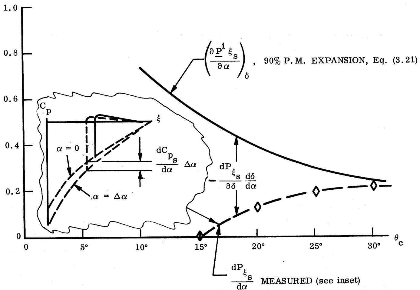
Fig. 3-13 Effect of Angle-of-Attack on Adverse Pressure Gradient Around \alpha = 0 at M_\infty = 0.88
