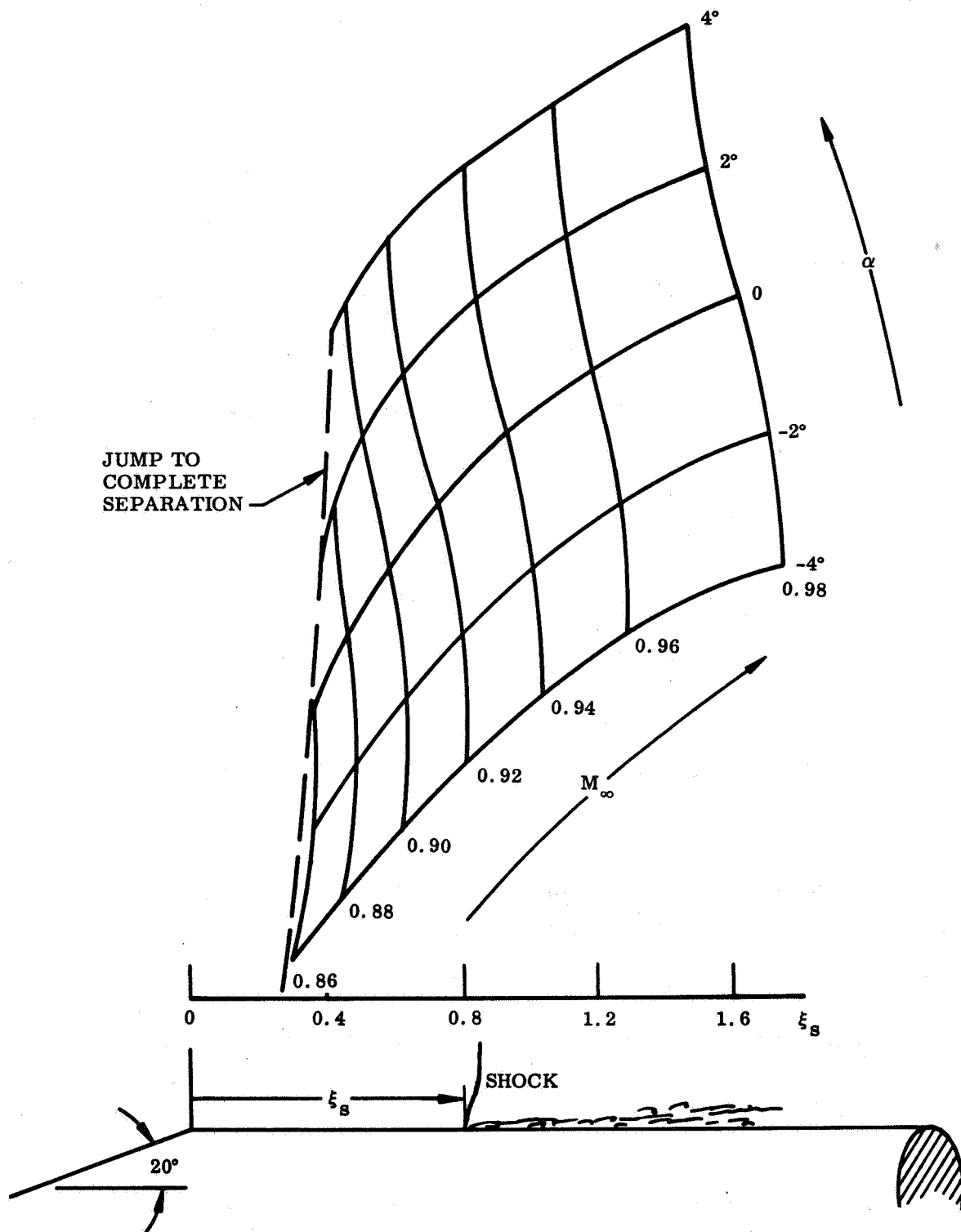
Fig. 2-6 Combined Effect of Mach Number and Angle-of-Attack on the Terminal-Shock Location on a 20° Cone-Cylinder Body
