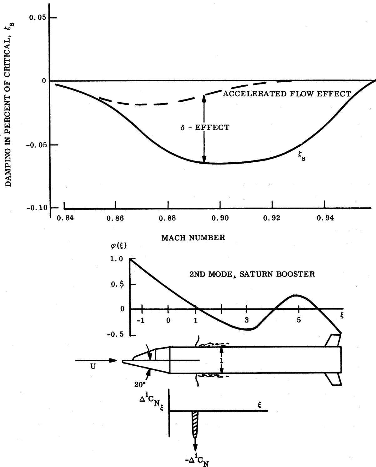
Fig. 4-1 Effect of Separation-Induced Terminal-Shock Movement on the Damping of an Elastic Vehicle Oscillating in Its Second Bending Mode
