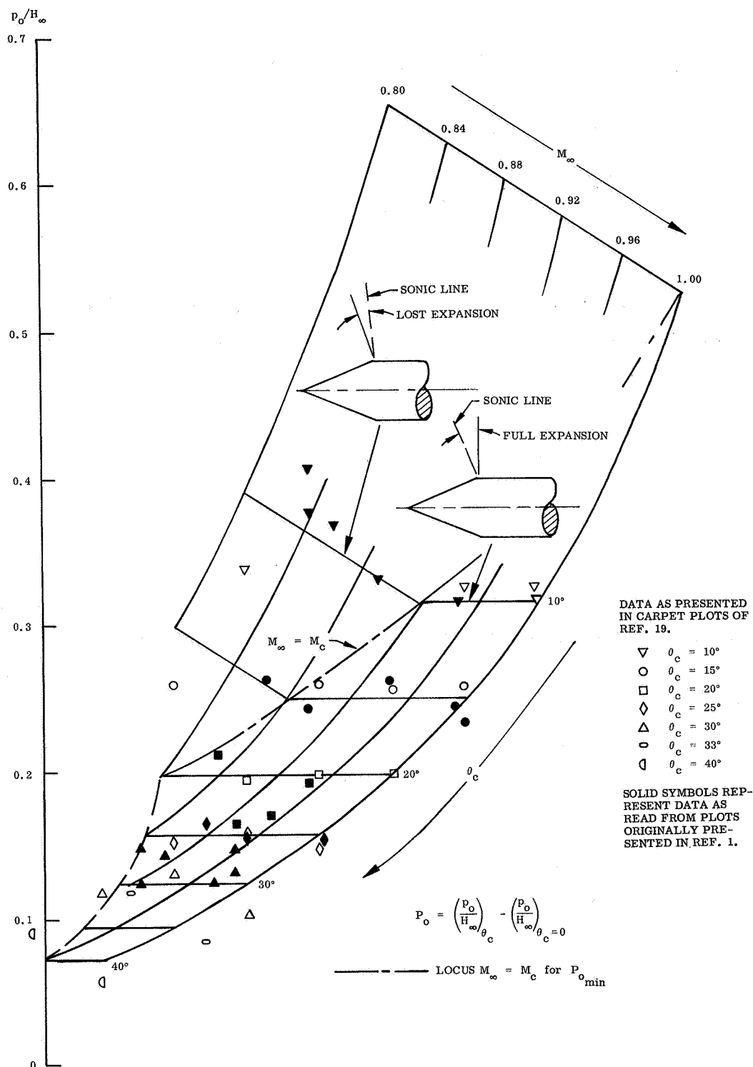
Fig. 3-5 Shoulder Pressure P_o as a Function of Cone Angle \theta_c and Mach Number M_\infty at \alpha = 0
