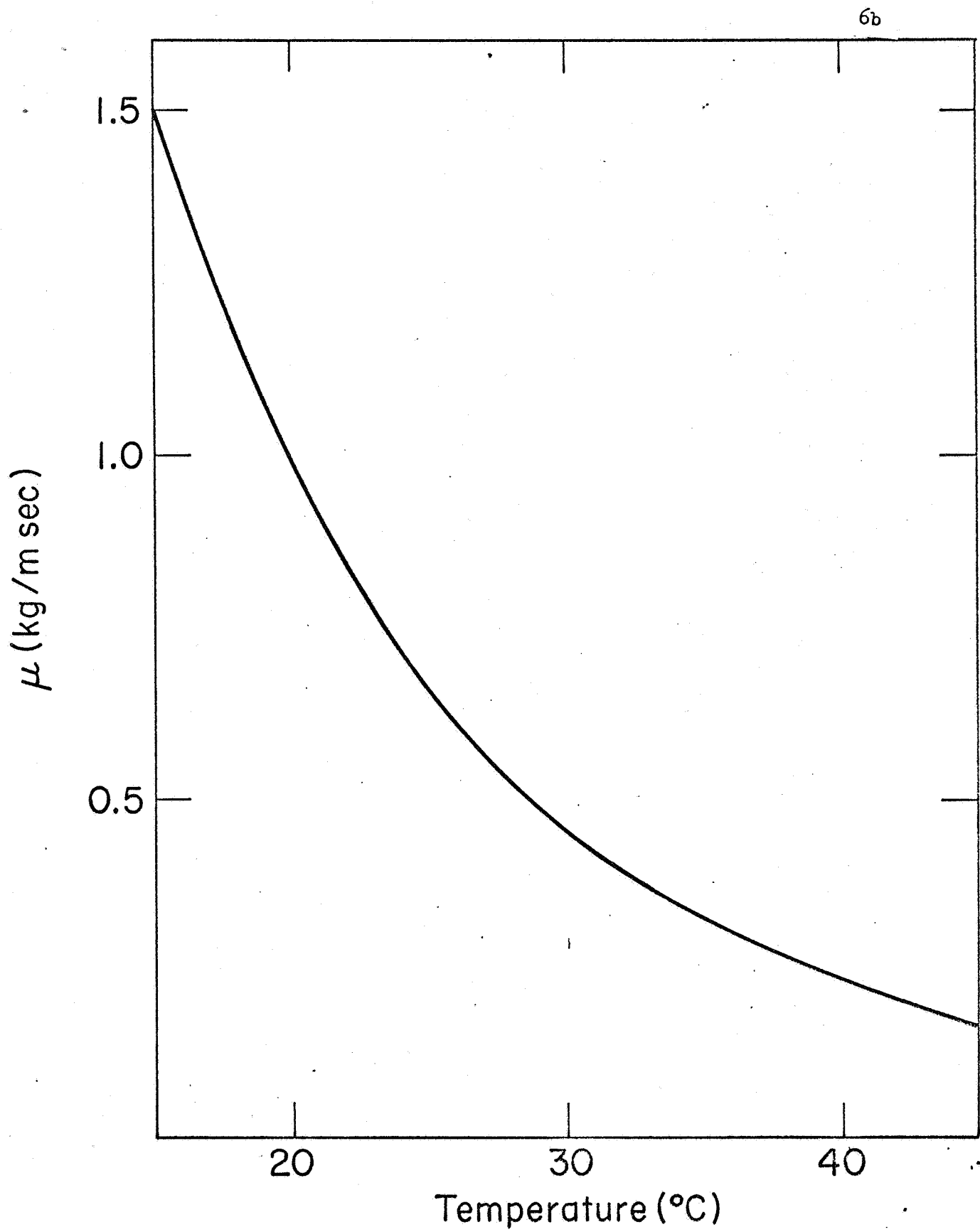
Fig. 9 Fluid properties as functions of temperature: b) Viscosity of castor oil
