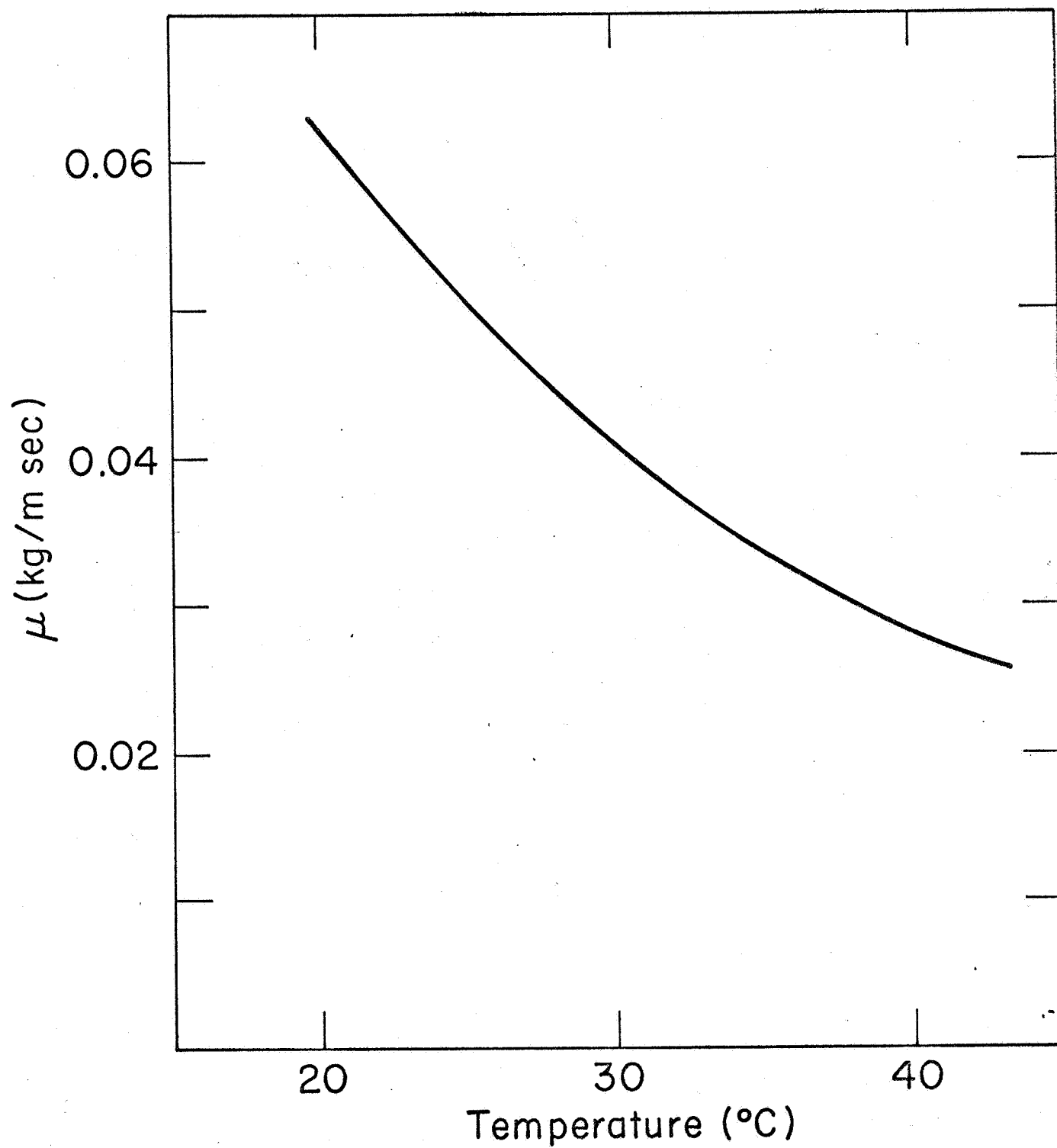
Fig. 9 Fluid properties as functions of temperature: a) Viscosity of corn oil
