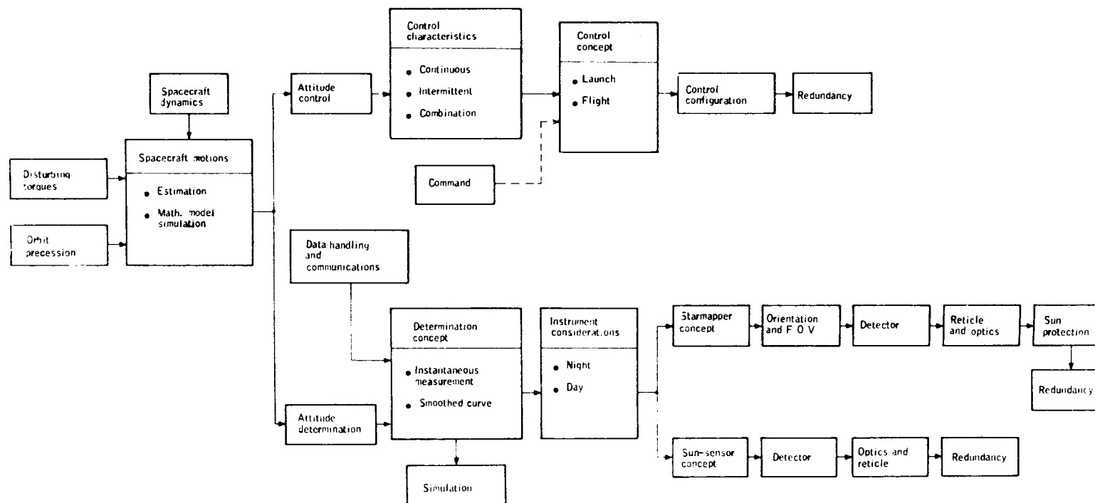
Figure 55. Attitude Determination and Control Study Flow Diagram
