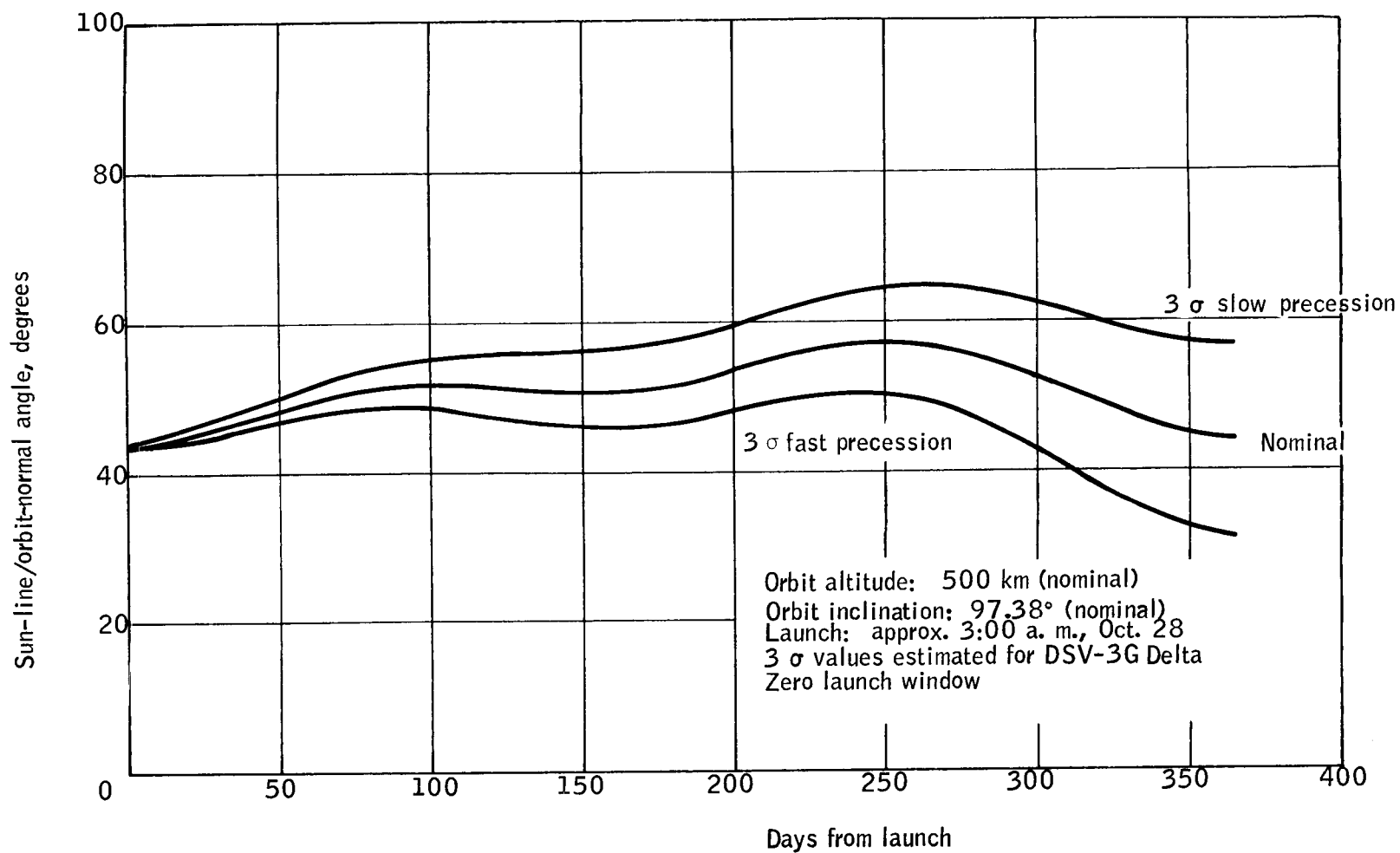
Figure 31. Sun-Line/Orbit-Normal Angle versus Days
