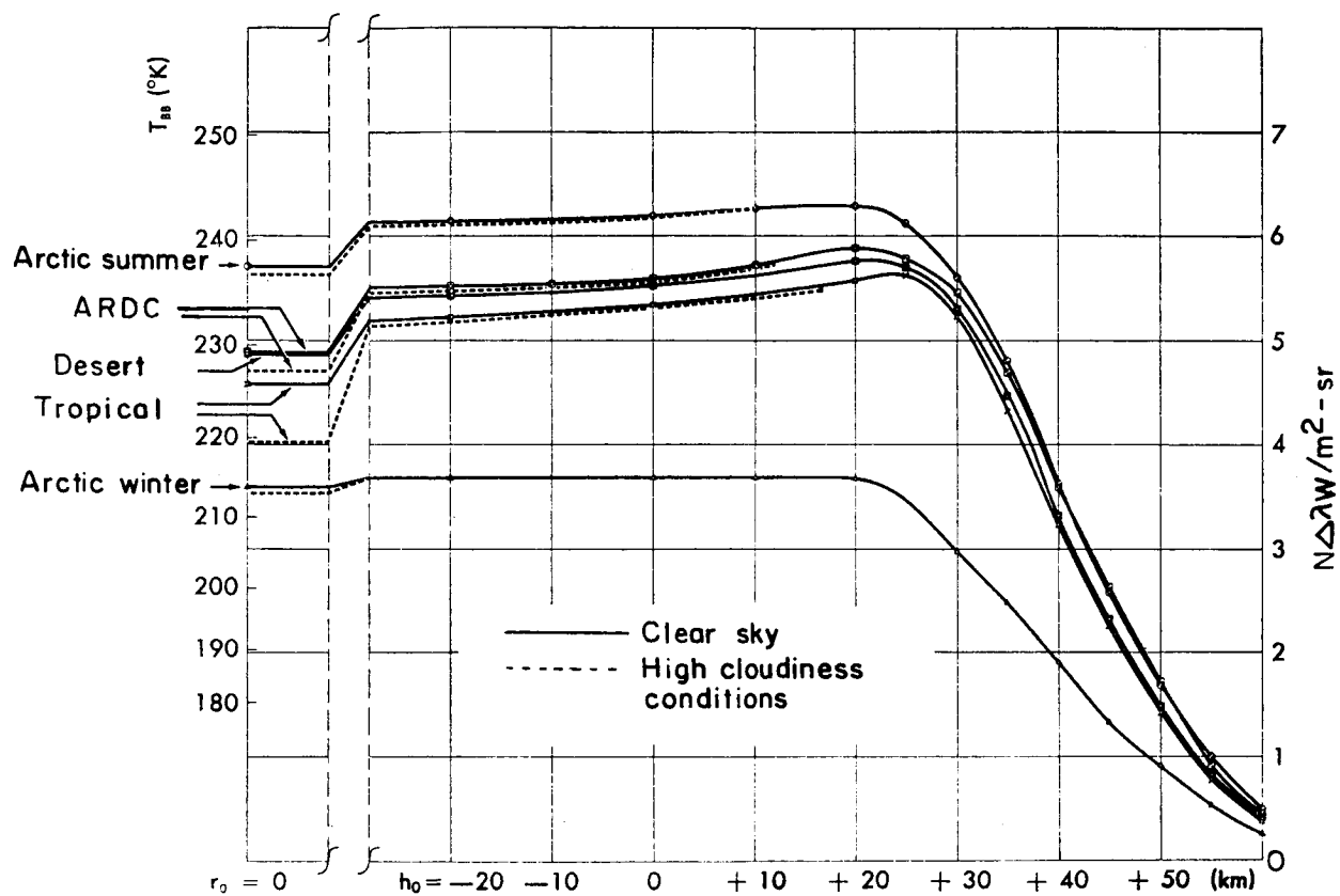
Figure 3. Curves of Radiance in the 15 Micron \text{CO}_2 Band versus Altitude for Five Model Atmosphere (ref. 1)
