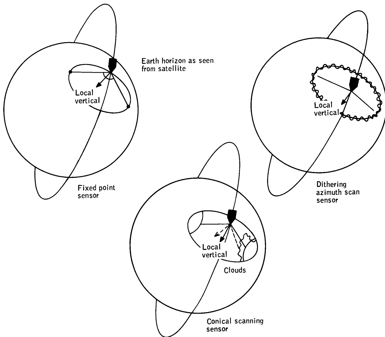
Figure 1. Examples of Horizon Sensor Operation
