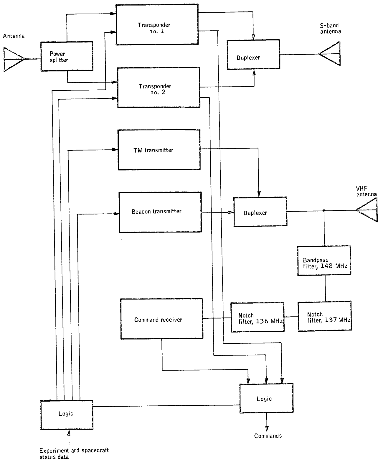
Figure 67. Communication Subsystem Block Diagram
