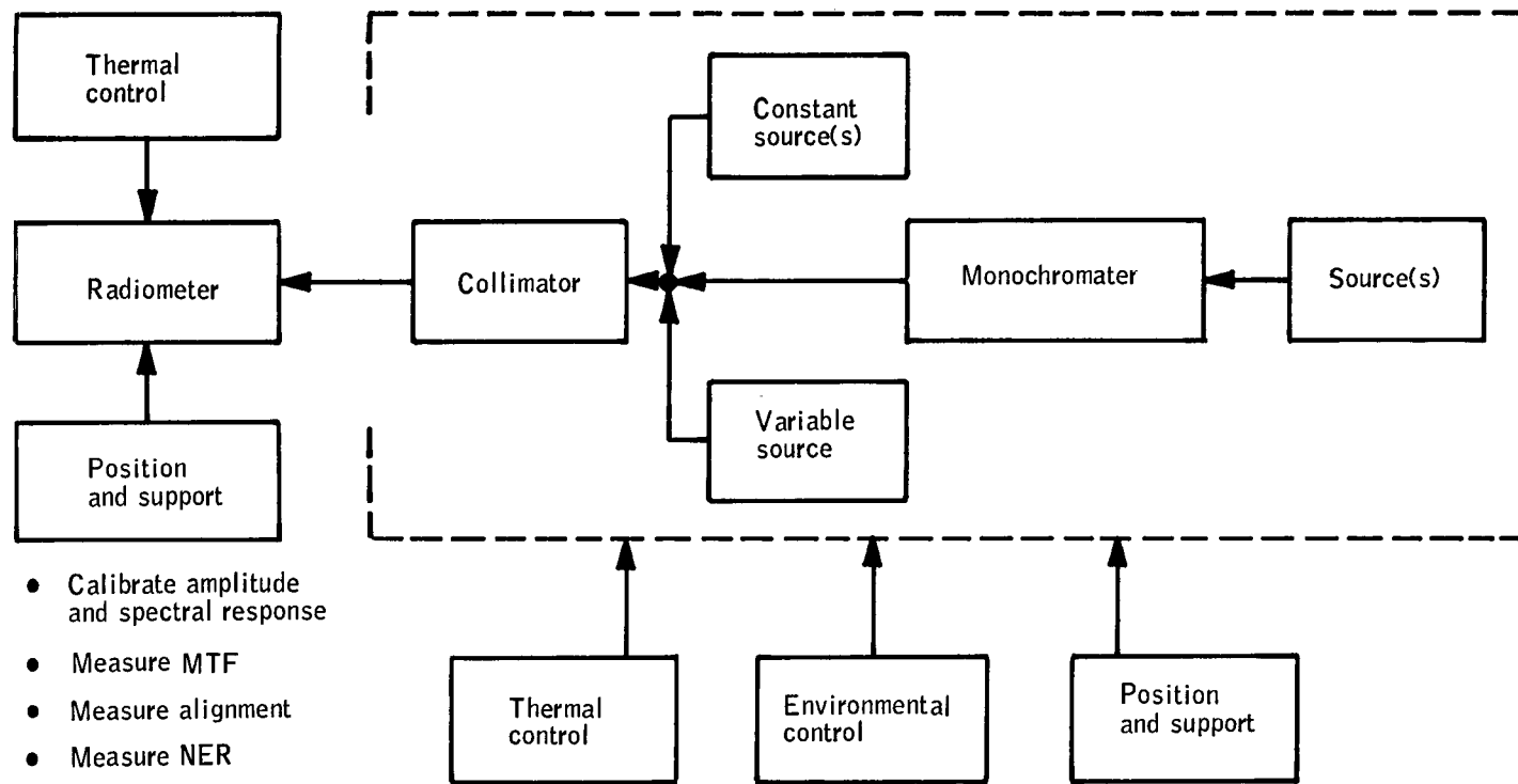
Figure 39. Primary Calibration Schematic Block Diagram
