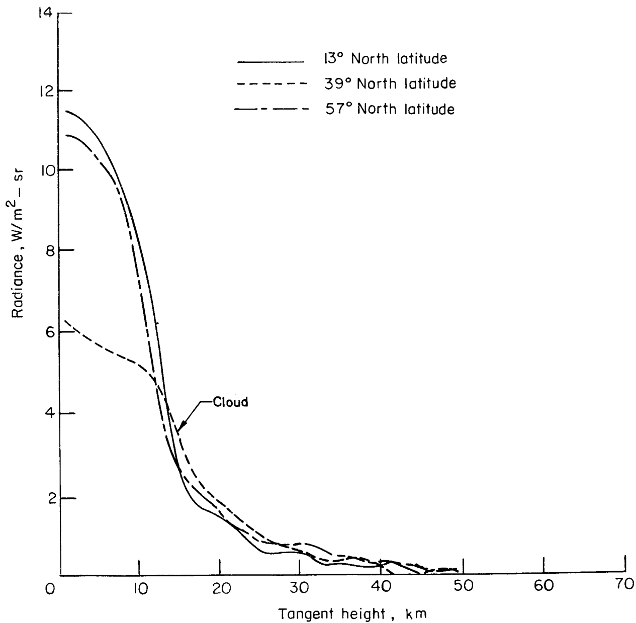
Figure 5. Measured Radiance Profiles in 315\text{ cm}^{-1} to 475\text{ cm}^{-1} Band (ref. 2)
