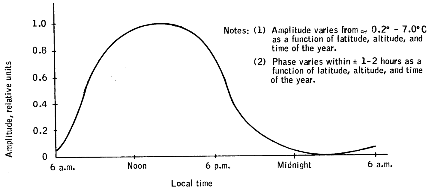
Figure 18. Typical Curve of Diurnal Temperature Variation
