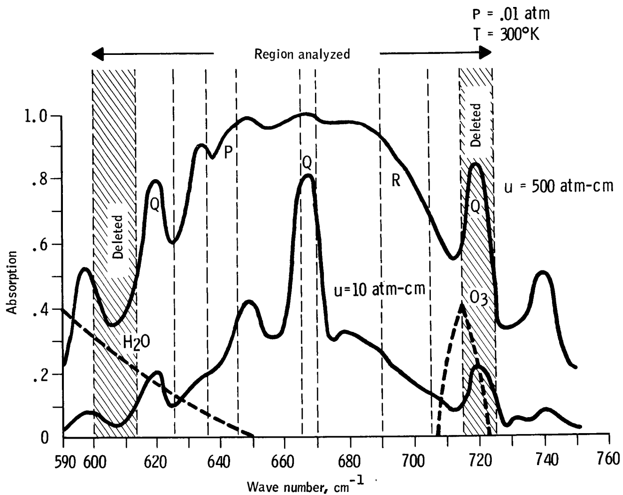
Figure 16. \text{CO}_2 Spectral Absorption
