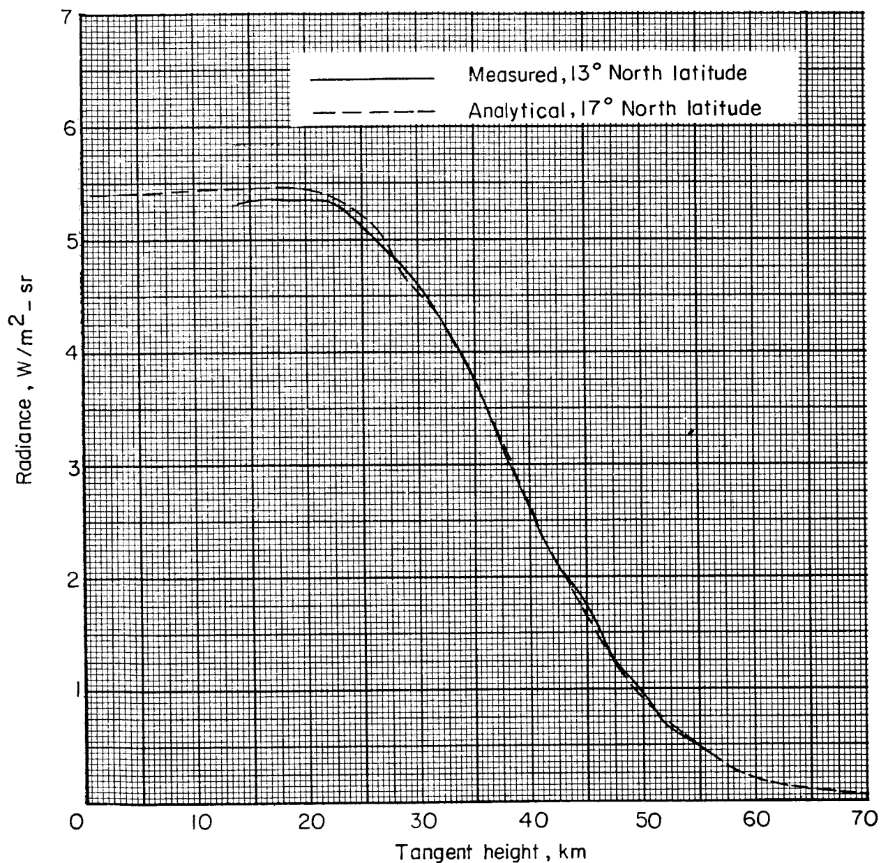
Figure 4. Comparison of Measured and Analytical Radiance Profiles in 615\text{ cm}^{-1} to 715\text{ cm}^{-1} Band (ref. 2)
