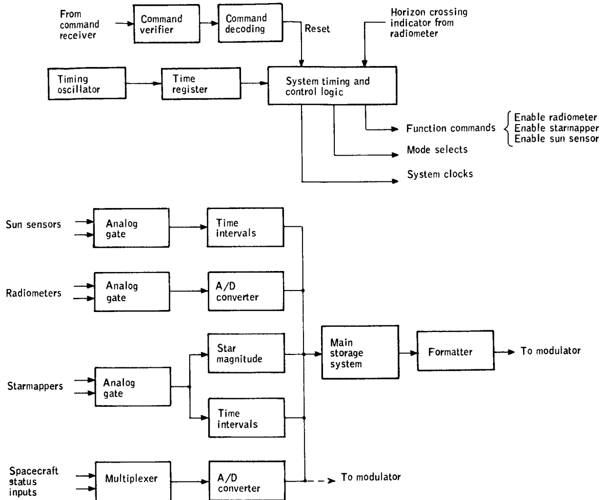
Figure 63. Data Handling Subsystem Block Diagram
