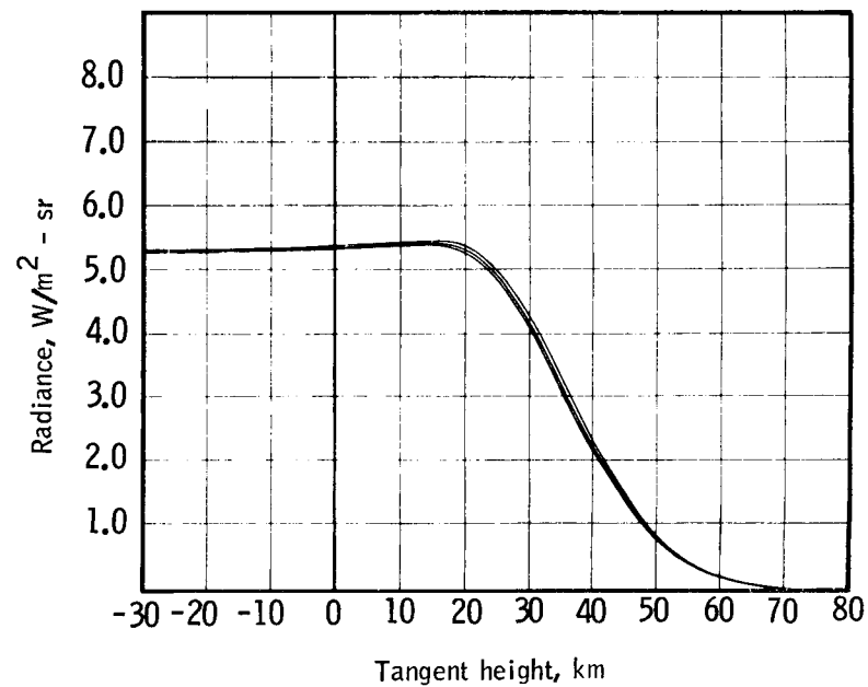
b. Radiance profile variation -30 to +80 km \pm 10\%
