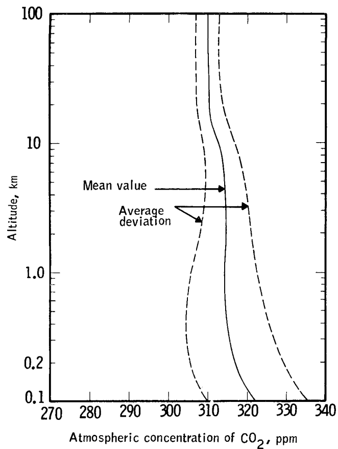
a. \text{CO}_2 variation 0 to 100 km \pm 3\%
