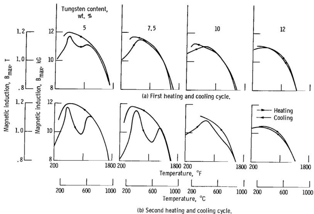
Figure 6. - Effect of tungsten content on magnetic stability of alloy \text{Co-Ti-}\frac{1}{2}\text{Zr-}\frac{1}{2}\text{C} . Maximum magnetizing force, 100 oersteds (7958 A/m).
