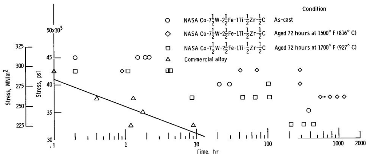
Figure 15. - Stress-rupture data for alloy Co-7 \frac{1}{2} W-2 \frac{1}{2} Fe-1Ti- \frac{1}{2} Zr- \frac{1}{2} C and commercial alloy at 1400° F (760° C).
