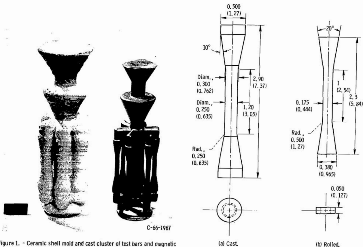
Figure 2. - Tensile and stress-rupture specimens. (Dimensions in inches (and cm).)
