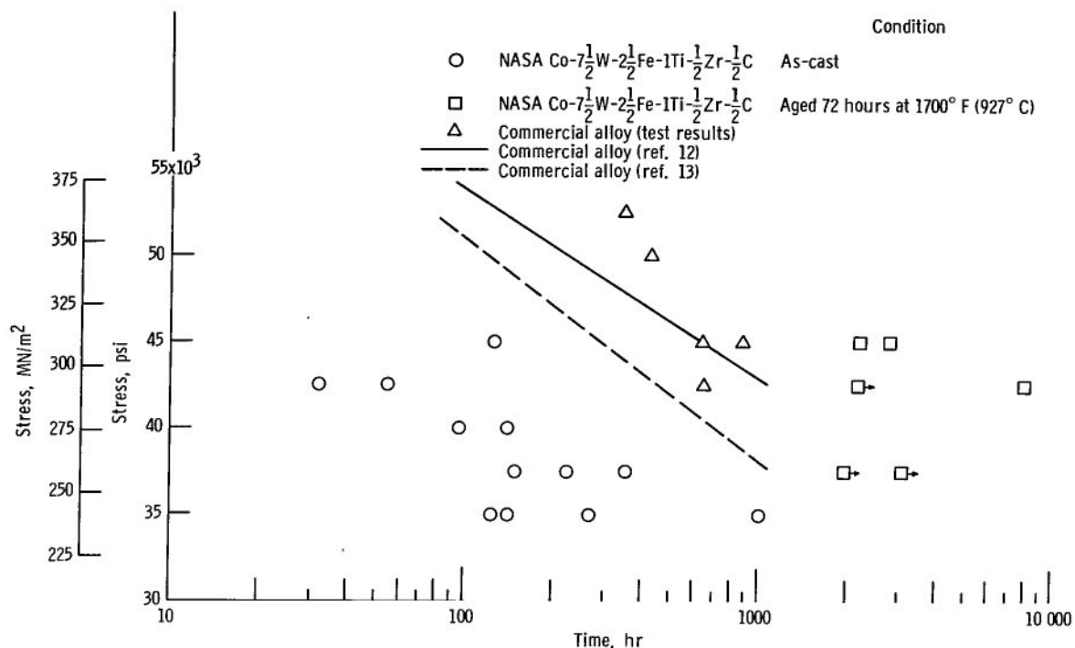
Figure 13. - Stress-rupture data for \text{Co-7}\frac{1}{2}\text{W-2}\frac{1}{2}\text{Fe-1Ti-}\frac{1}{2}\text{Zr-}\frac{1}{2}\text{C} alloy and commercial alloy at 1200^{\circ}\text{F} ( 649^{\circ}\text{C} ).
