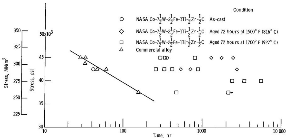
Figure 14. - Stress-rupture data for alloy \text{Co-7}\frac{1}{2}\text{W-2}\frac{1}{2}\text{Fe-1Ti-}\frac{1}{2}\text{Zr-}\frac{1}{2}\text{C} and commercial alloy at 1300^{\circ}\text{F} ( 704^{\circ}\text{C} ).
