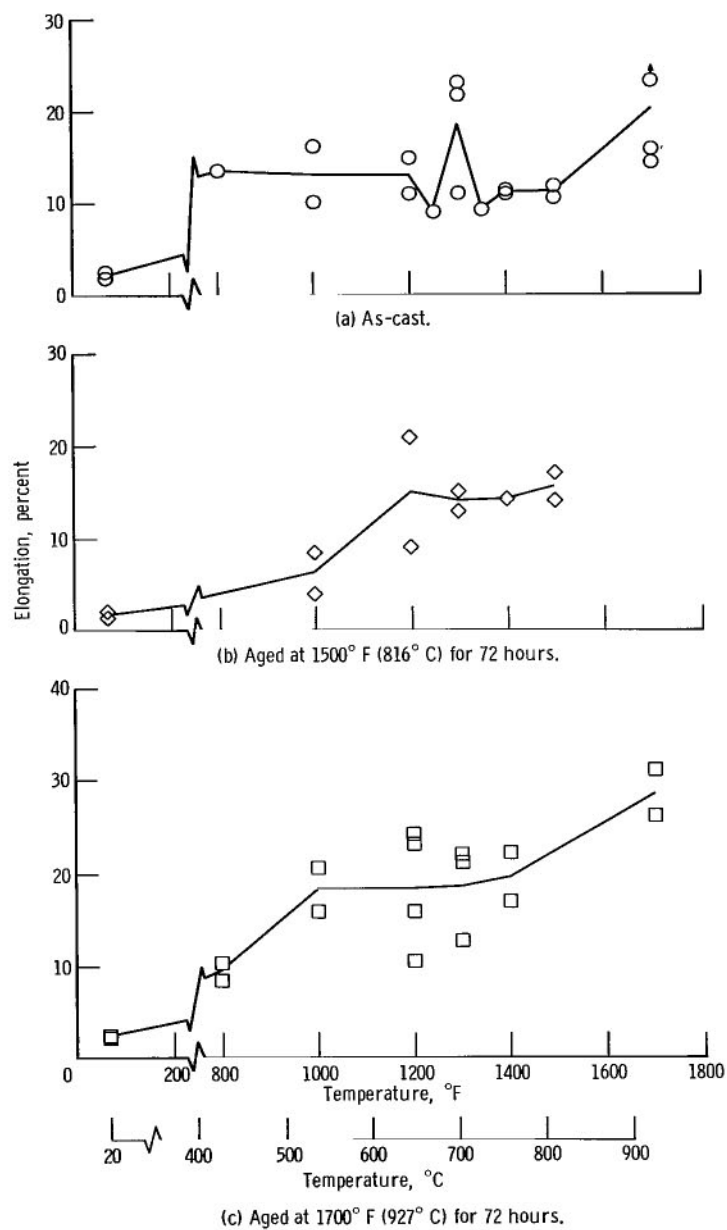
Figure 12. - Effect of temperature on tensile ductility of alloy \text{Co}-7\frac{1}{2}\text{W}-2\frac{1}{2}\text{Fe}-1\text{Ti}-1\frac{1}{2}\text{Zr}-1\frac{1}{2}\text{C} .
