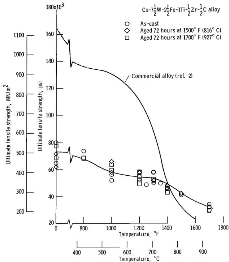
Figure 11. - Effect of temperature on ultimate tensile strength of alloy Co-7½W-2½Fe-1Ti-½Zr-½C and of commercial magnetic alloy.
