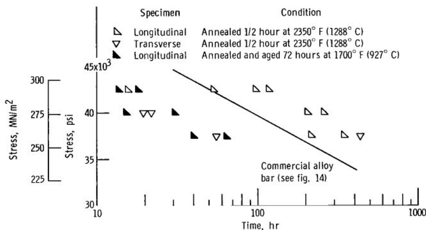
Figure 16. - Stress-rupture data for alloy Co-7 \frac{1}{2} W-2 \frac{1}{2} Fe-1Ti- \frac{1}{2} Zr- \frac{1}{2} C sheet at 1300° F (704° C).
