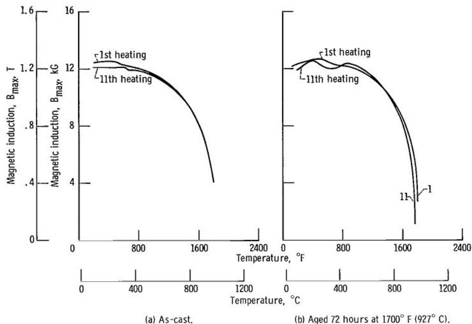
Figure 8. - Effect of heat treatment on magnetic stability of alloy \text{Co}-7\frac{1}{2}\text{W}-2\frac{1}{2}\text{Fe}-1\text{Ti}-\frac{1}{2}\text{Zr}-\frac{1}{2}\text{C} after repeated heating cycles. Maximum magnetizing force, 100 oersteds (7958 A/m).
