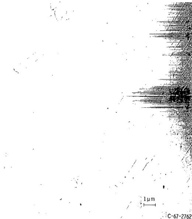
Figure 23. - Electron micrograph of cast alloy Co - 7\frac{1}{2} W - 2\frac{1}{2} Fe - 1 Ti - \frac{1}{2} Zr - \frac{1}{2} C aged 72 hours at 1700° F (927° C) and exposed for 1000 hours at 1300° F (704° C). X10 500.
