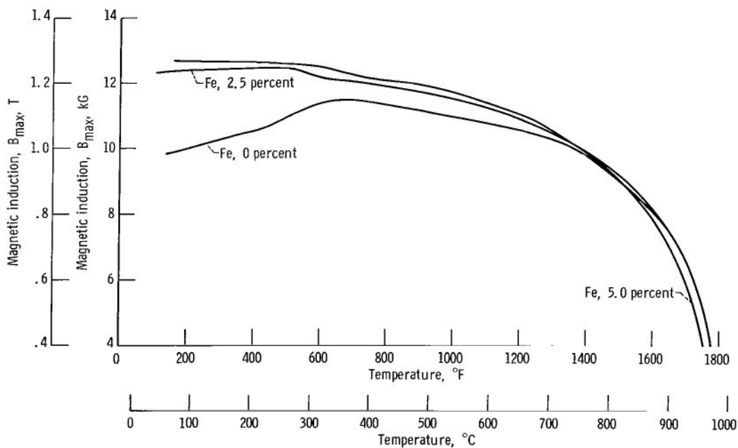
Figure 7. - Effect of temperature and iron content on magnetic induction of alloy \text{Co-}\frac{7}{2}\text{W-Ti-}\frac{1}{2}\text{Zr-}\frac{1}{2}\text{C} . Maximum magnetizing force, 100 oersteds (7958 A/m). Data obtained during first heating of cast specimens.
