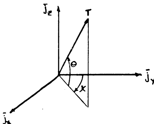
Figure 4-2 PLATFORM (P) COORDINATE SYSTEM
