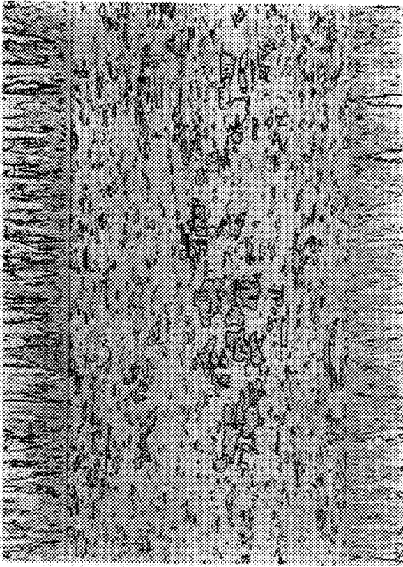
(a) Ni-1ThO 2
