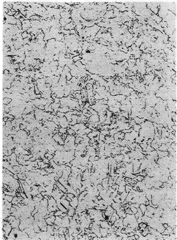
(b) Ni-13.5Cr-1ThO 2
