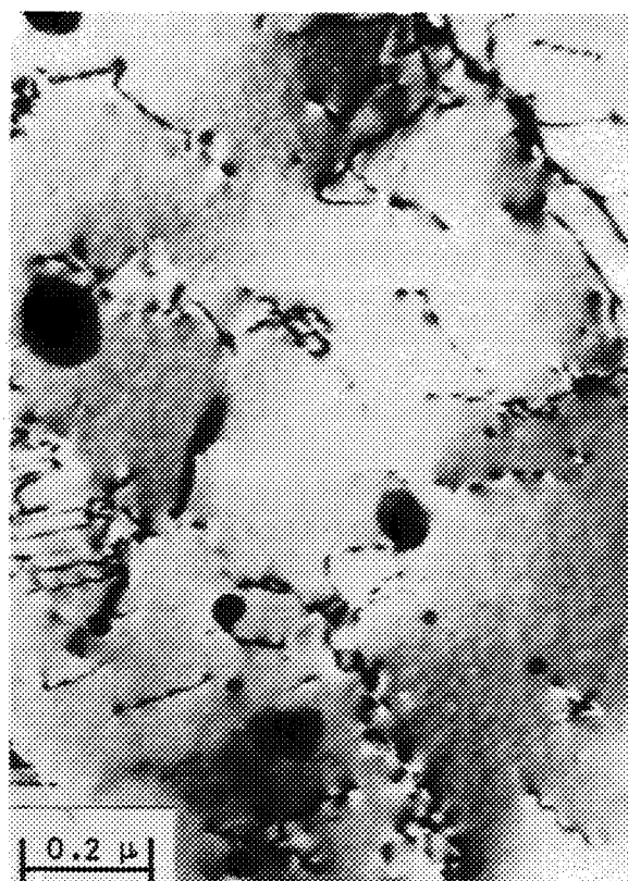
(b) Ni-13.5Cr-1ThO 2
