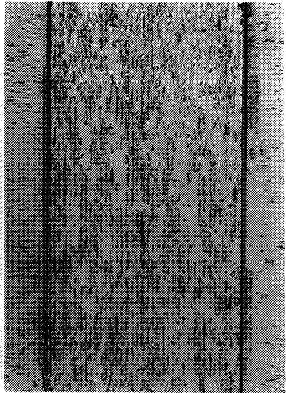
(b) Ni-13.5Cr-1ThO 2
