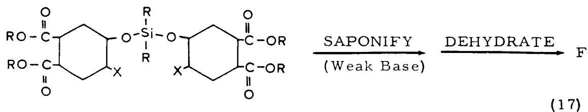
SYNTHESIS F
