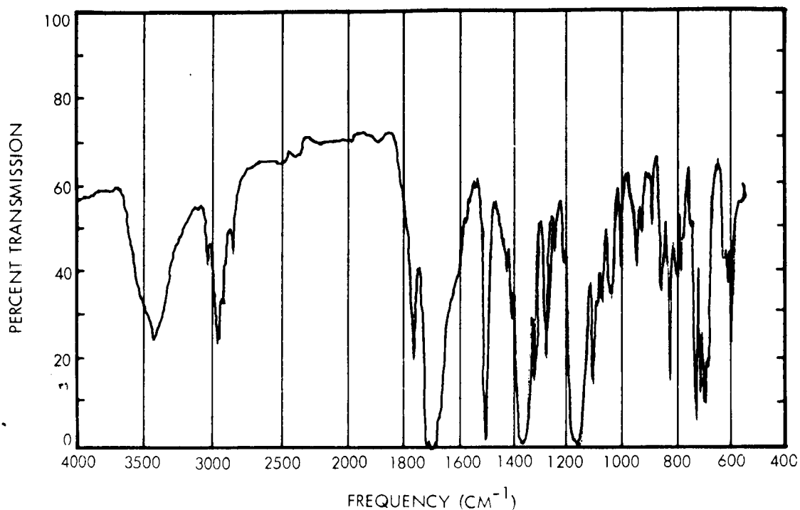
Figure A-12. Infrared Spectrum of p,p'-Diphenylmethane-di(3,6-Endomethylene-1,2,3,6-Tetrahydro-phthalimide)
