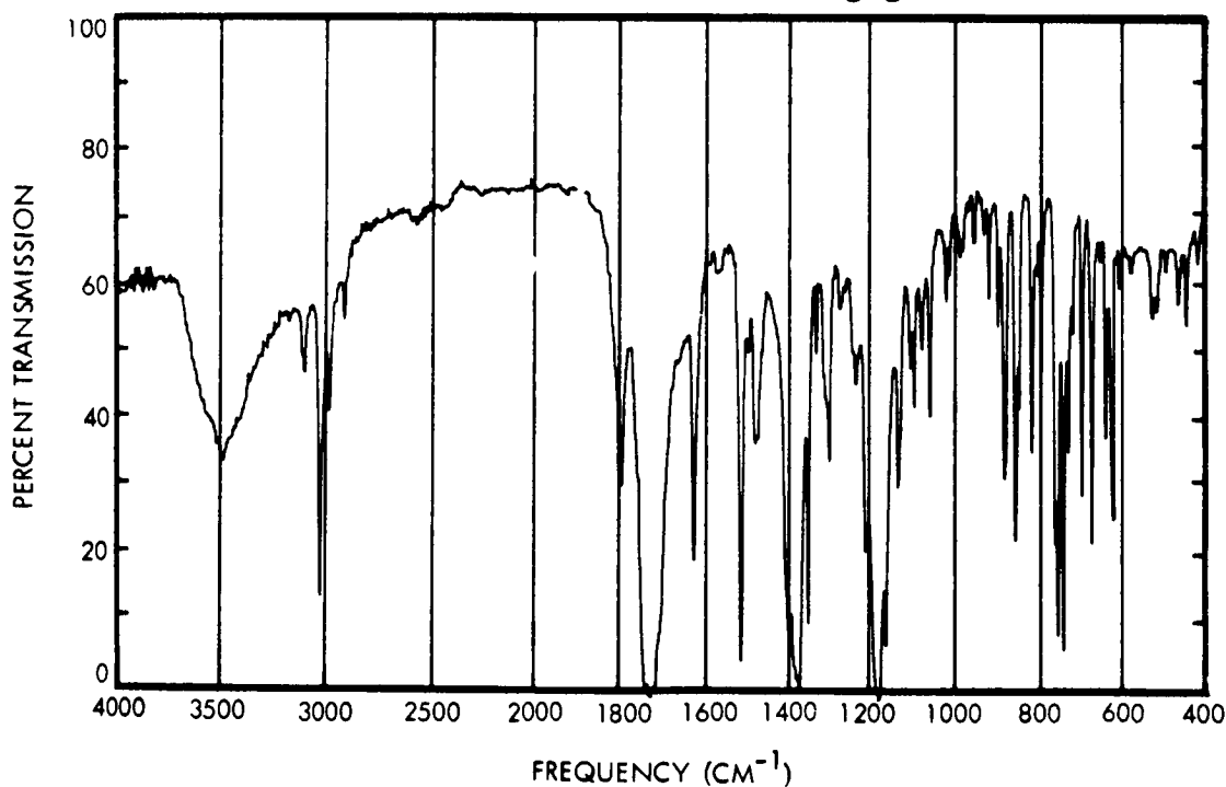
Figure A-13. Infrared Spectrum of m-Phenylene di-(3,6-Endomethylene-1,2,3,6-Tetrahydro-phthalimide)
