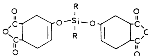
MONOMER F
