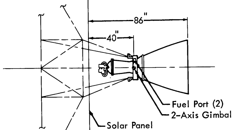
TITAN IIIC TRANSTAGE ENGINE
