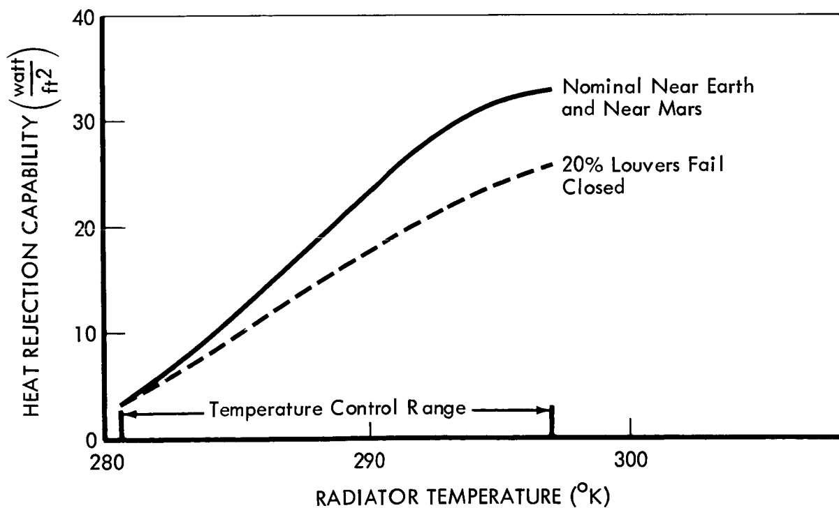
Figure 1.2.12-5: RADIATOR-LOUVER PERFORMANCE
