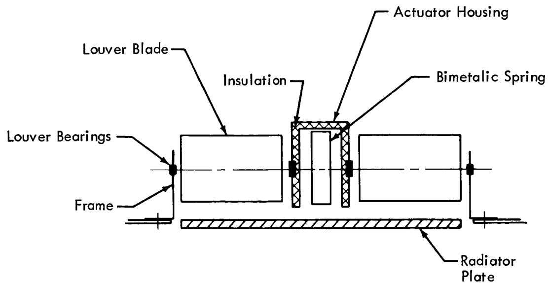
Figure 1.2.12-4: RADIATOR-LOUVER ASSEMBLY SCHEMATIC
