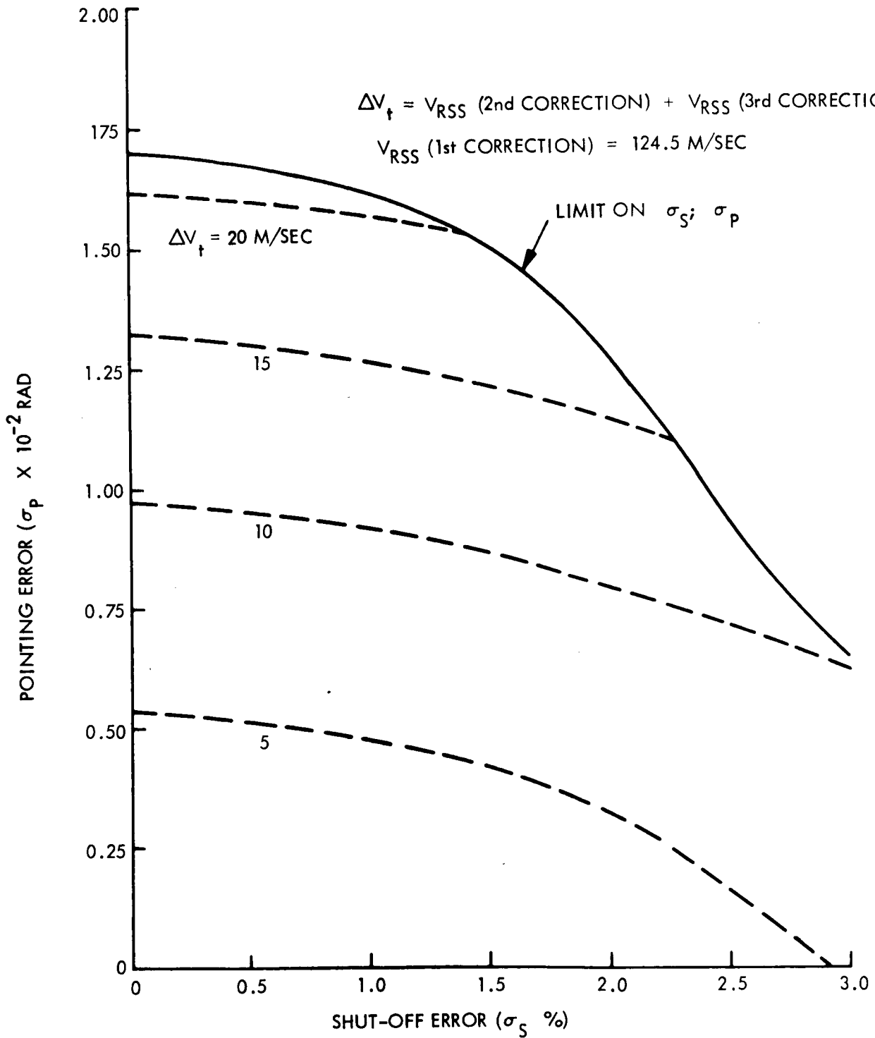
Figure 25. Guidance Accuracy Requirements 1973 Earth-Mars Trajectory
