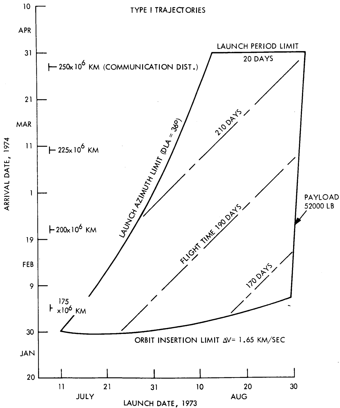
Figure 2. 1973 Mission Envelope - Type I Trajectories
