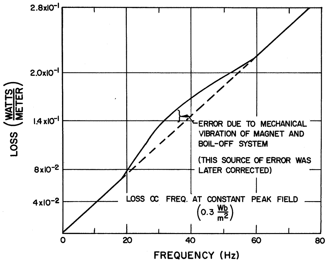
Fig. 5 Loss vs Frequency at Constant Peak Field
