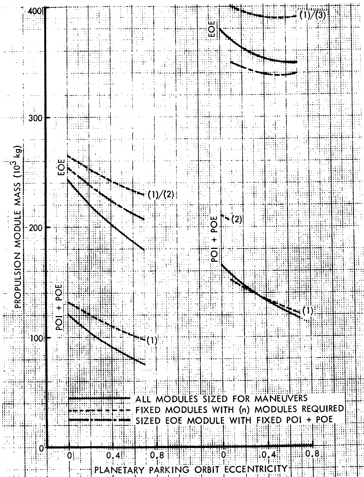
Figure 99. Fixed Propulsion Module Mass Requirements (1999 Mars Opposition)
