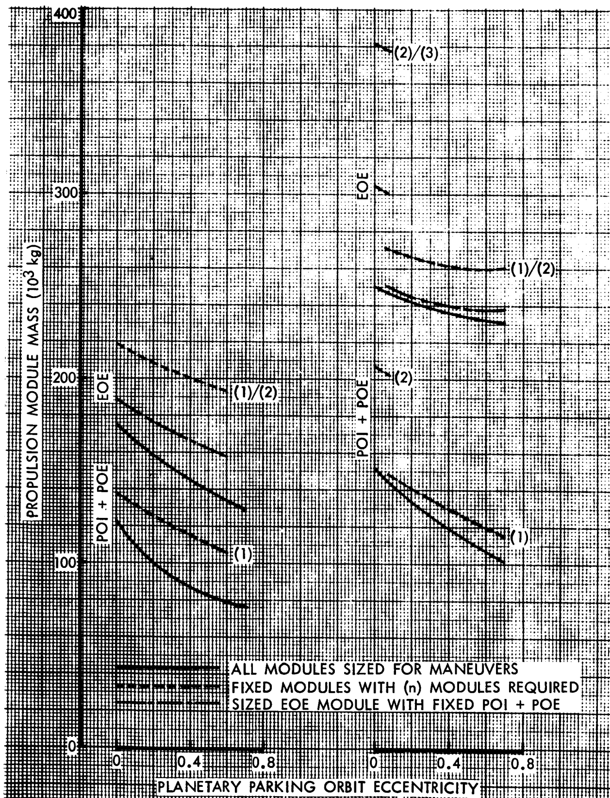
Figure 98. Fixed Propulsion Module Mass Requirements (1988 Mars Opposition)
