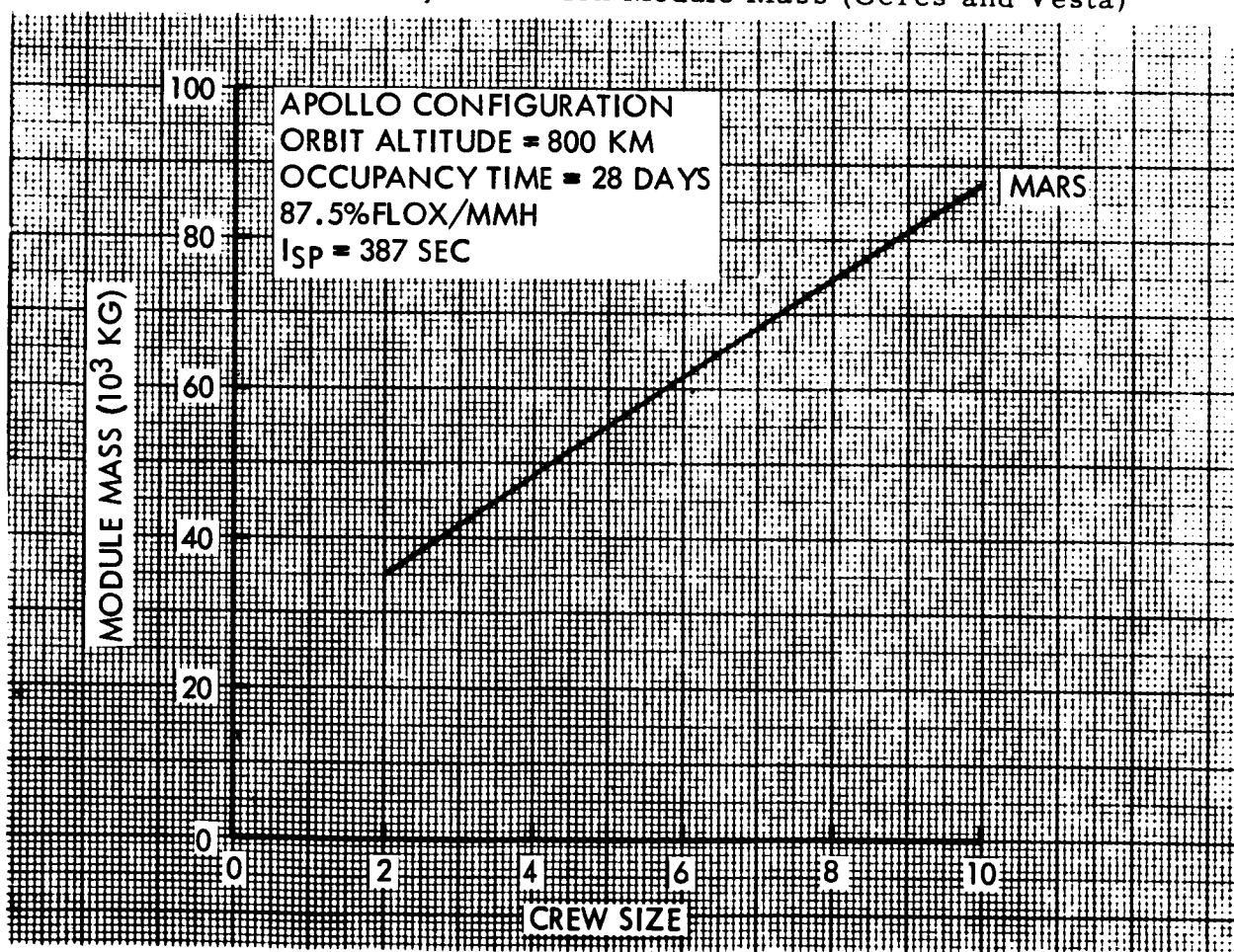
Figure 67. Planetary Excursion Module Mass (Mars)
