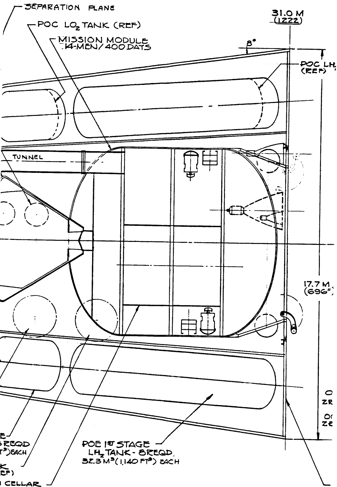
INBOARD PROFILE
