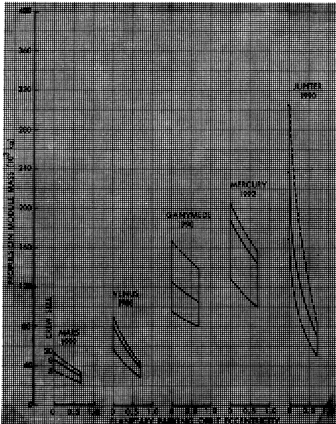
Figure 93. POE Propulsion Module Mass Requirements (20-Man Module with 8-Man Crew)
