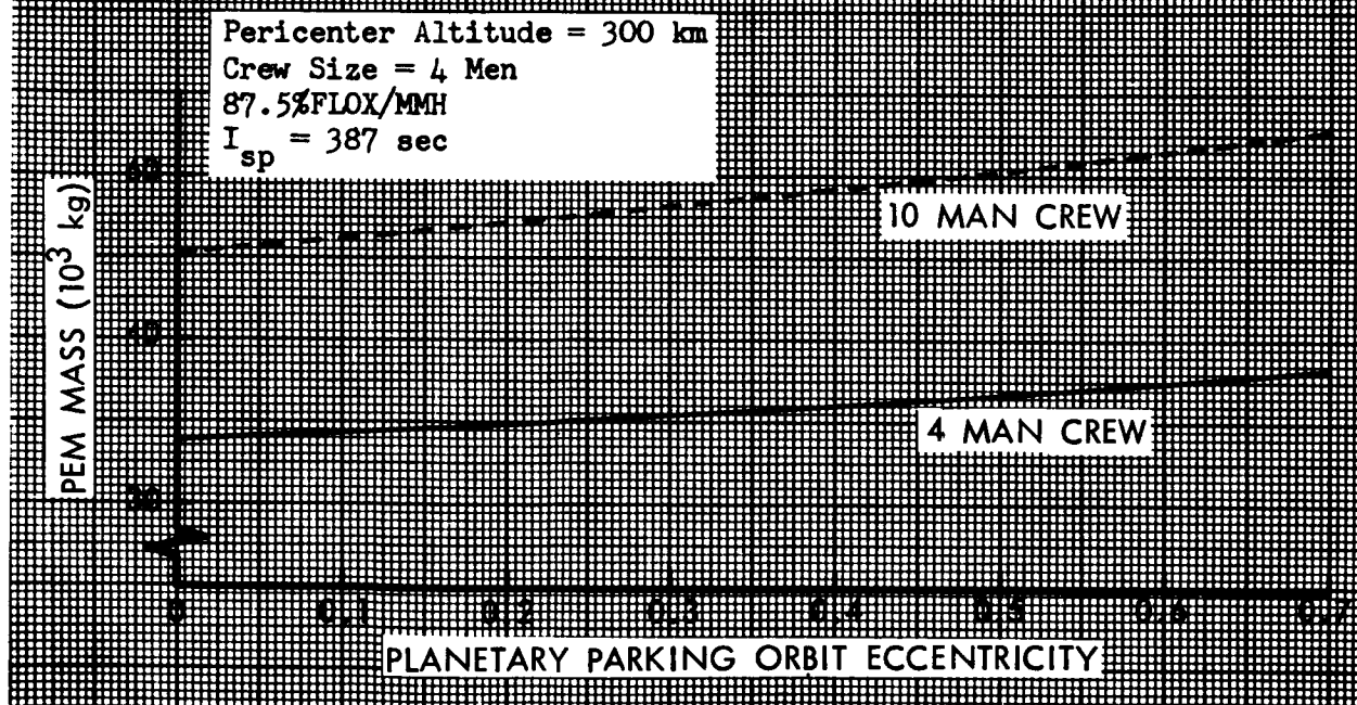
Figure 77. Ganymede Planetary Excursion Module Mass
