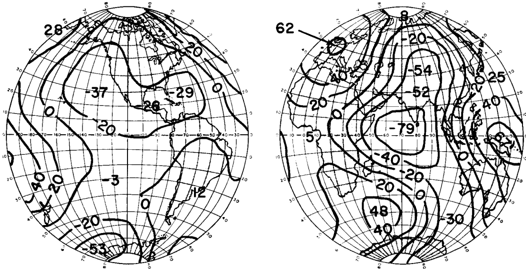
Fig. 1. Geoid heights in meters referred to an ellipsoid of flattening 1/298.25. Based on solution J, Table 6.
