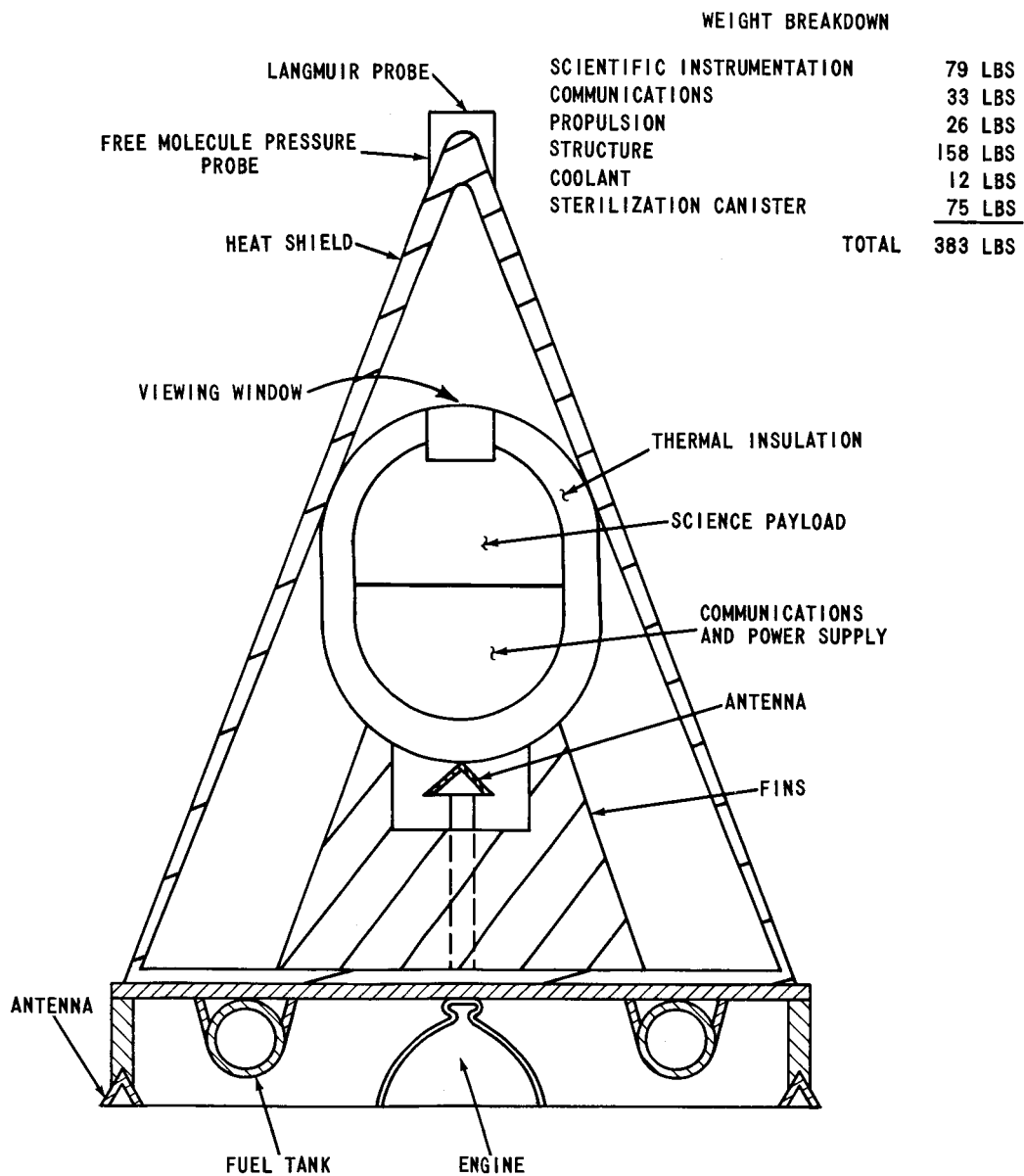
FIGURE 12 - OUTLINE OF PHOTO SINKER PROBE
