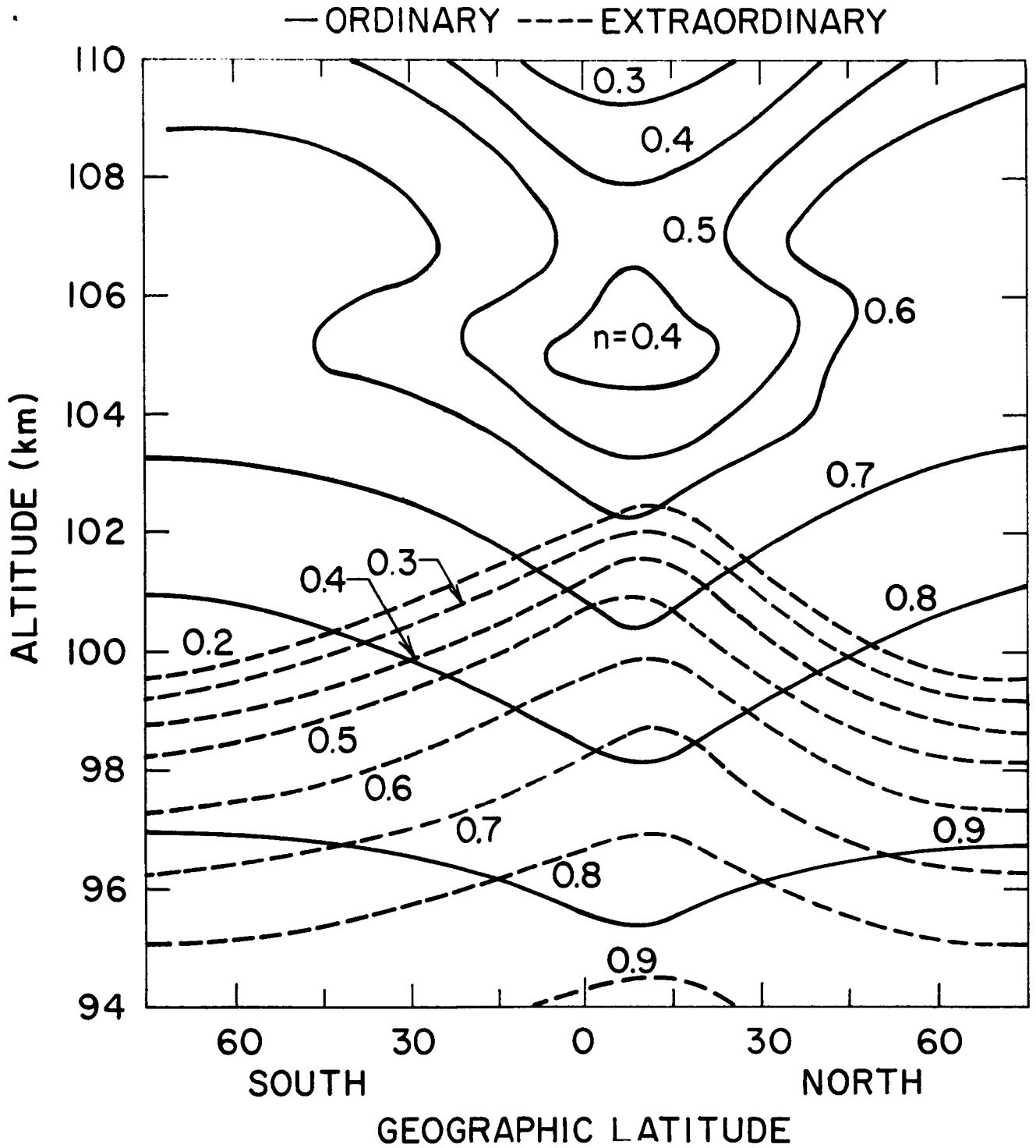
Figure 3.10 Contours showing height variation of constant refractive index levels for the ordinary and the extraordinary waves on 3.0 MHz.
