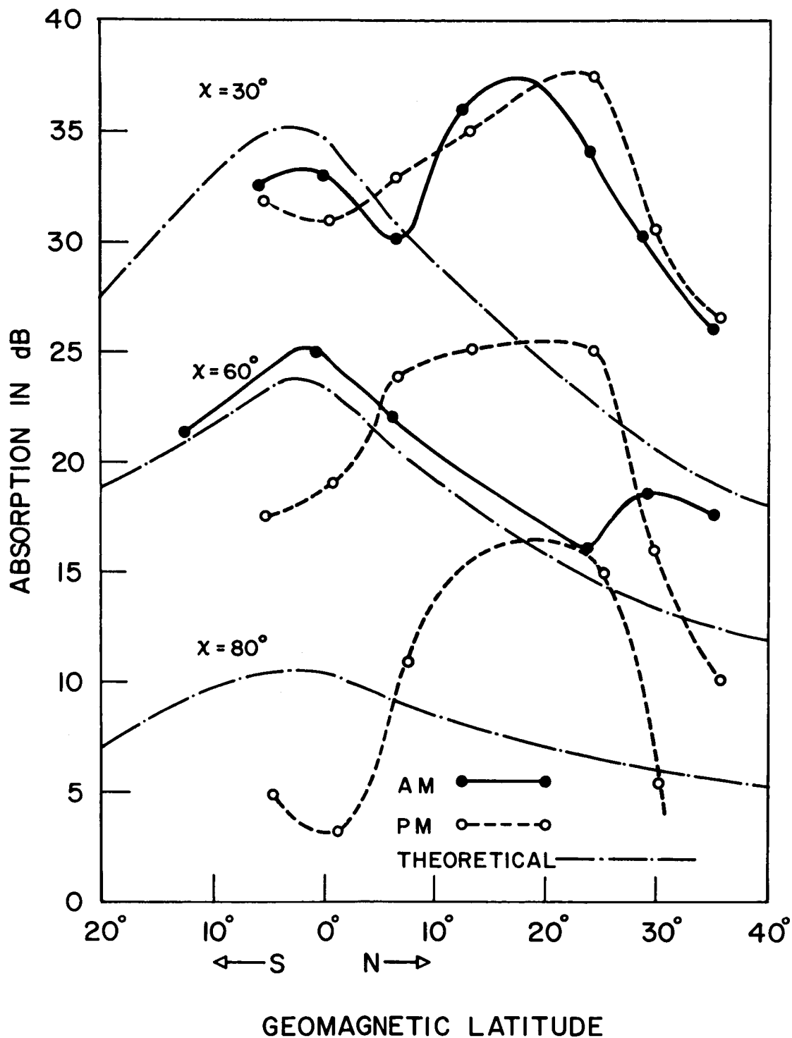
Figure 2.5 Absorption measured on board the USNS Croatan is shown as a function of the geomagnetic latitudes for each of the solar zenith angles 30, 60 and 80°. Also shown is the corresponding computed latitudinal variation of absorption presuming latitude invariant models of electron number density and electron collision frequency identical to those observed at a mid-latitude station.
