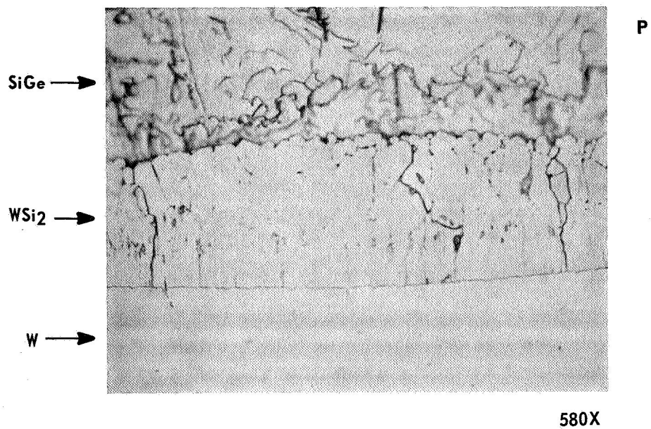
FIGURE 12. SOLAR PANEL COLD JUNCTION STRUCTURES AS-BONDED Reference Cold Shoe Bonds
