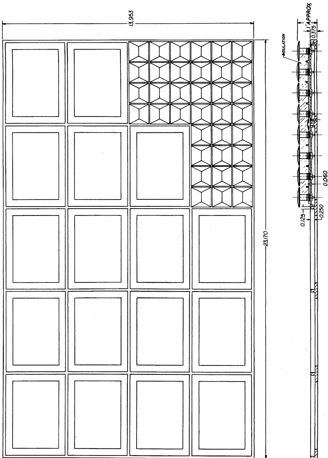
FIGURE A-3. REFERENCE DESIGN—GENERATOR PANEL ASSEMBLY
