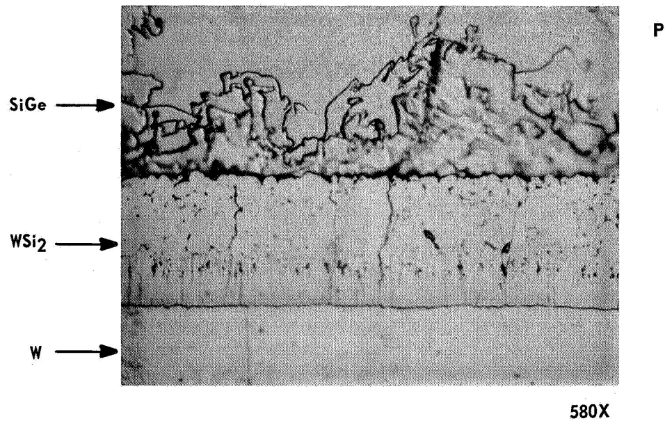
FIGURE 13. SOLAR PANEL COLD JUNCTION STRUCTURES ISOTHERMALLY TESTED SiGe-To-W Bonds---500°C - 500 Hrs. Vacuum
