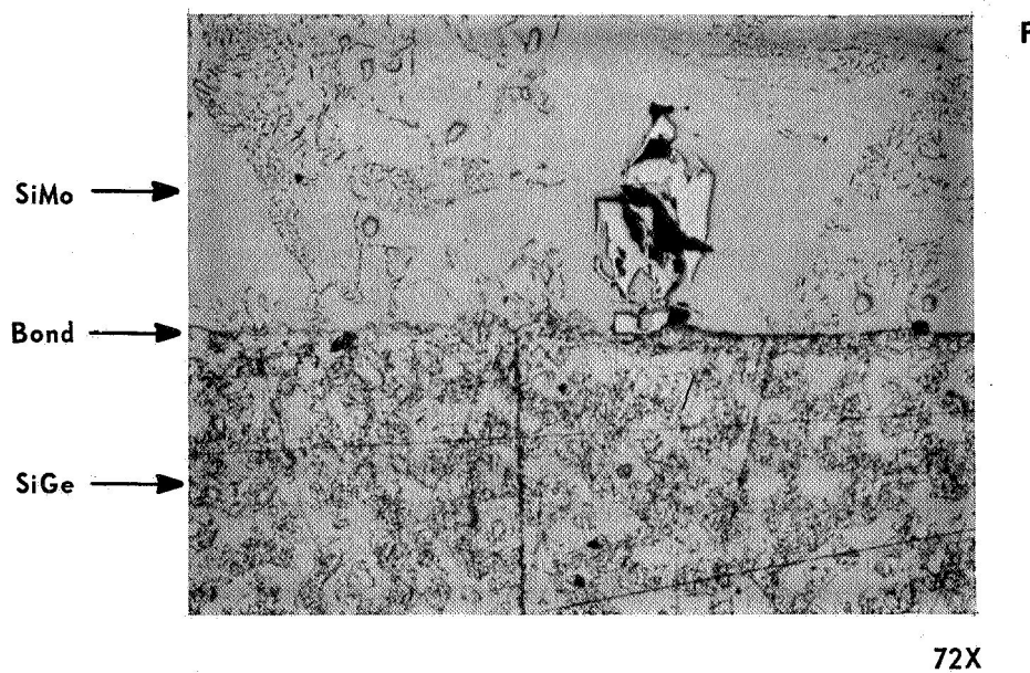
FIGURE 8. SOLAR PANEL HOT JUNCTION STRUCTURE AS-BONDED Sound Bond (Selected Areas show 1/2 of each bond with obvious liquid phase and 1/2 with no obvious liquid phase).
