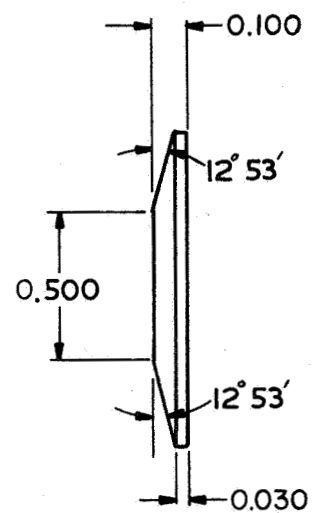
FIGURE 19. "HIPPED" HOT SHOE MACHINING SEQUENCE - STEPS 3, 4, AND 5
