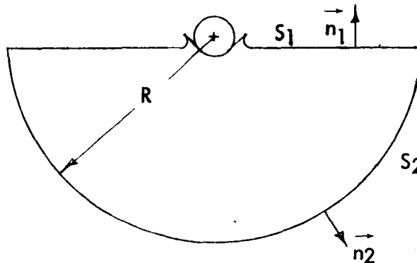
Figure 3. Virtual Mass
